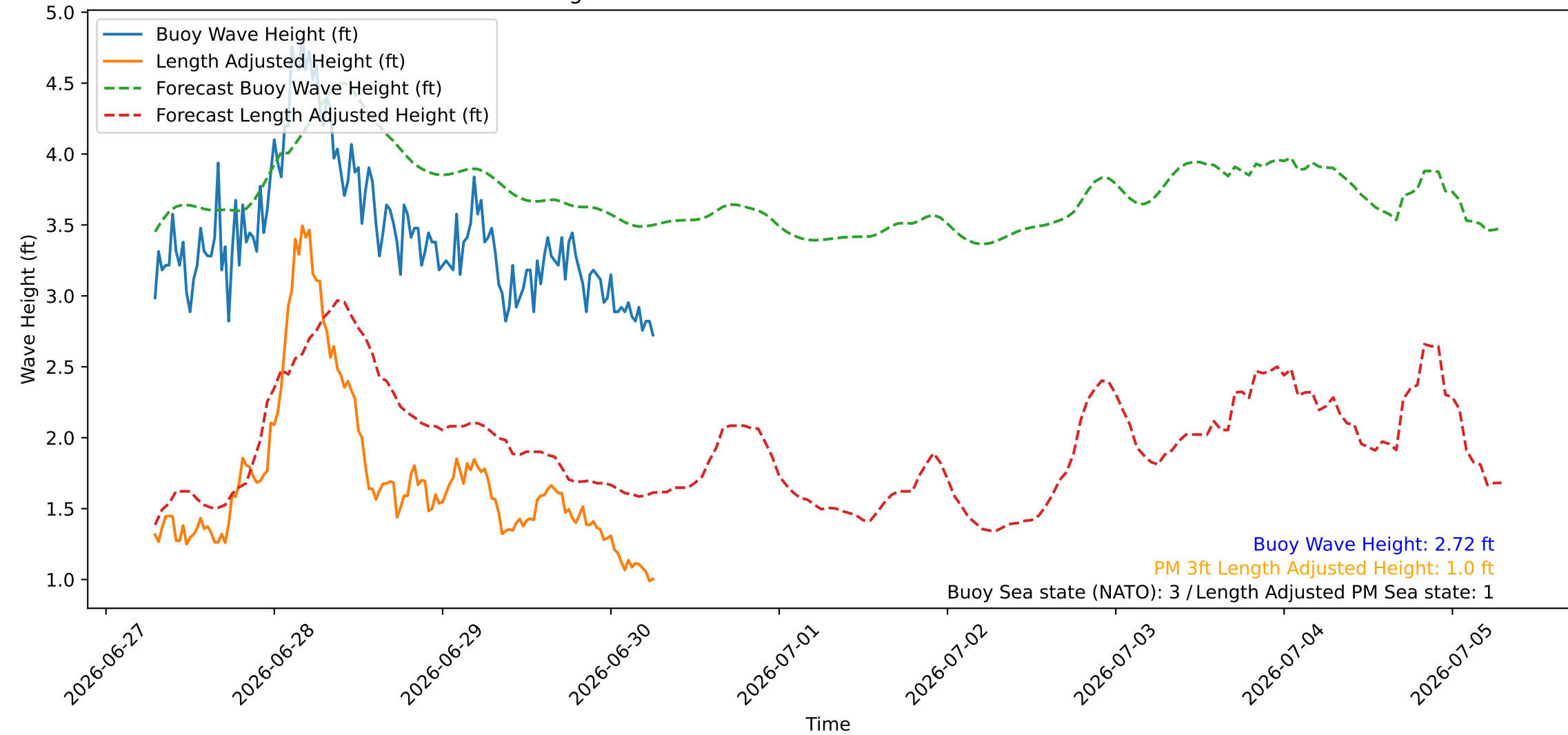
Wave Heights over Time for Green Beach at 2026-06-30 07:01:07
