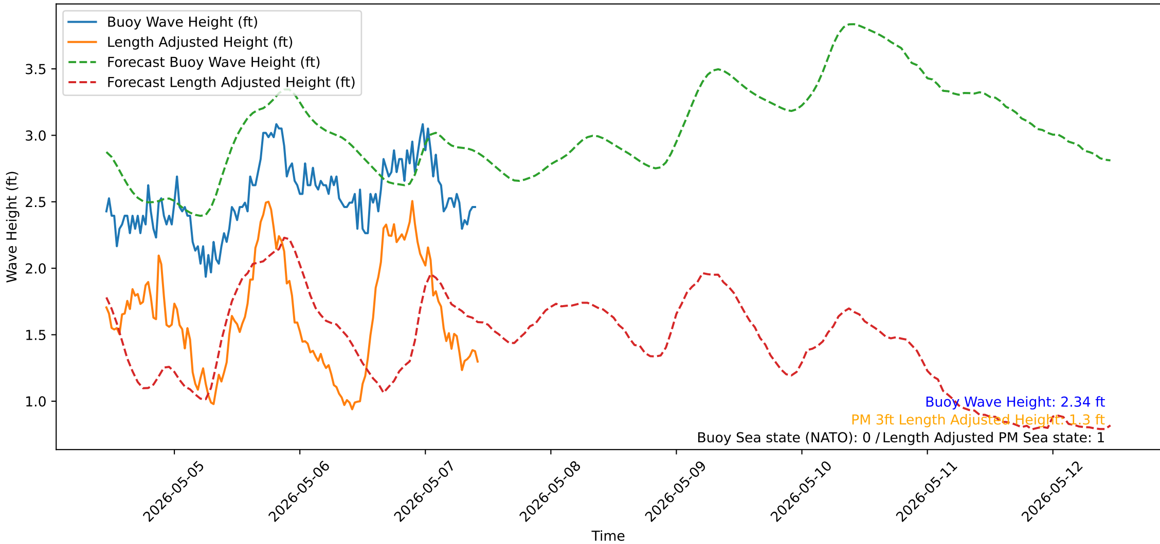
Wave Heights over Time for Red Beach at 2026-05-07 10:40:50
