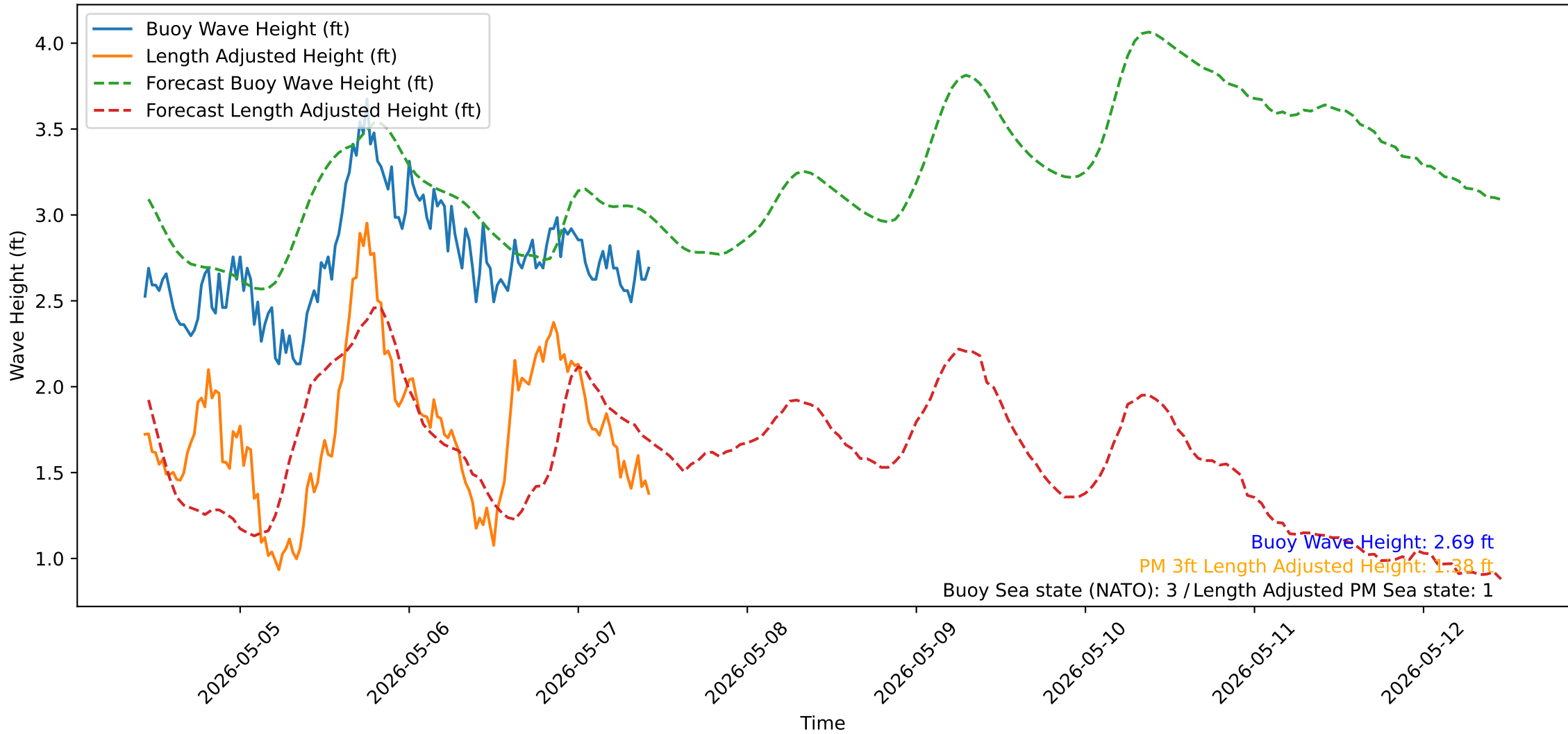
Wave Heights over Time for Green Beach at 2026-05-07 10:41:13
