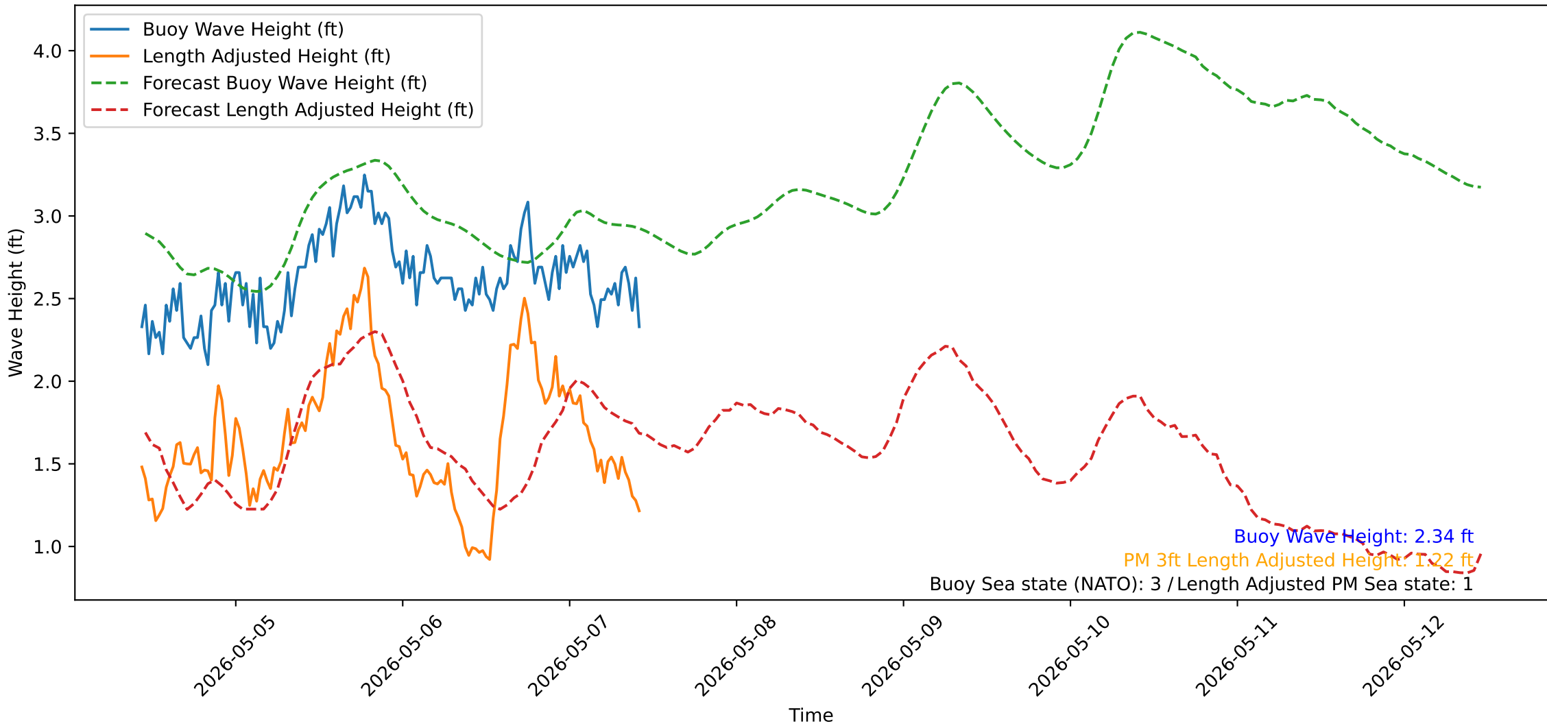
Wave Heights over Time for Oceanside Harbor at 2026-05-07 10:40:31
