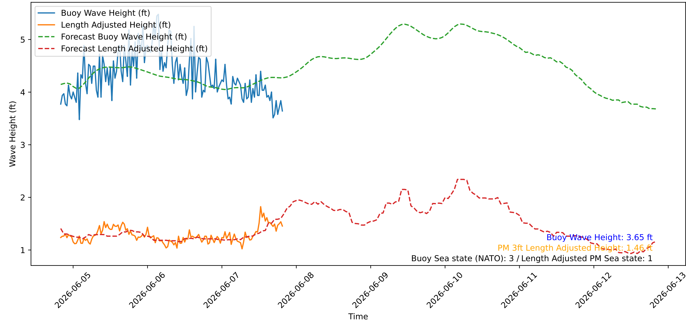
Wave Heights over Time for Oceanside Harbor at 2026-06-07 20:00:26
