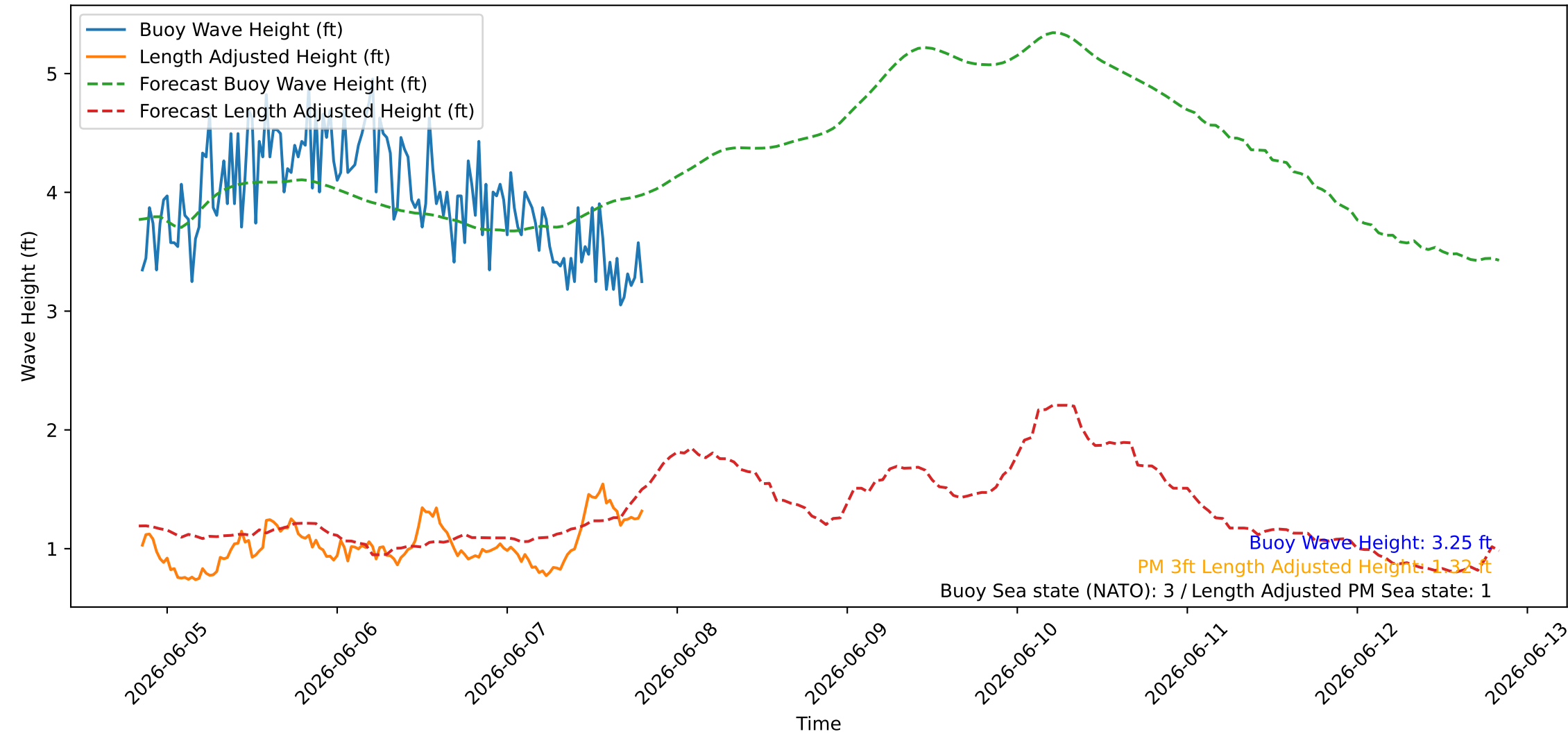
Wave Heights over Time for Red Beach at 2026-06-07 20:00:45
