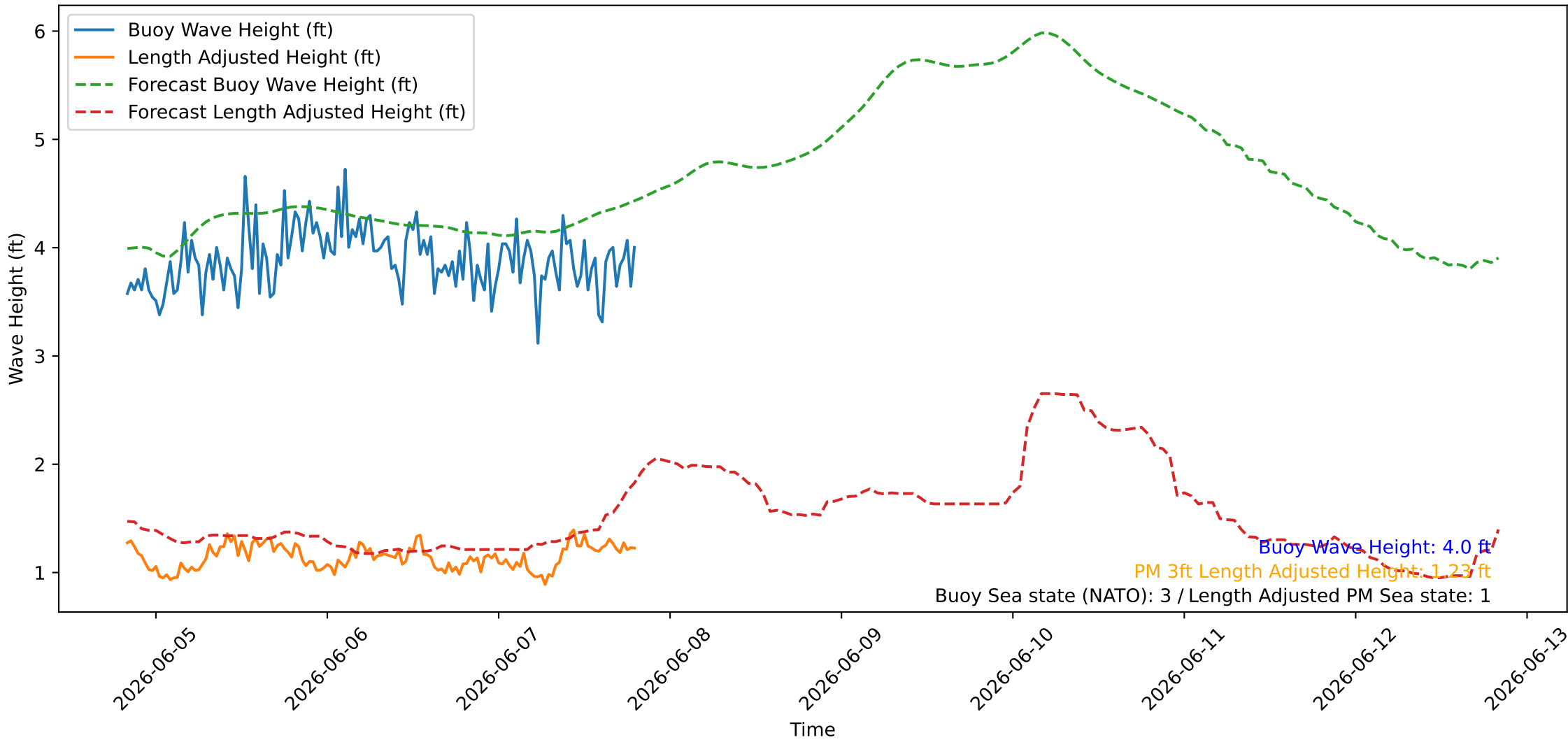
Wave Heights over Time for Green Beach at 2026-06-07 20:01:08
