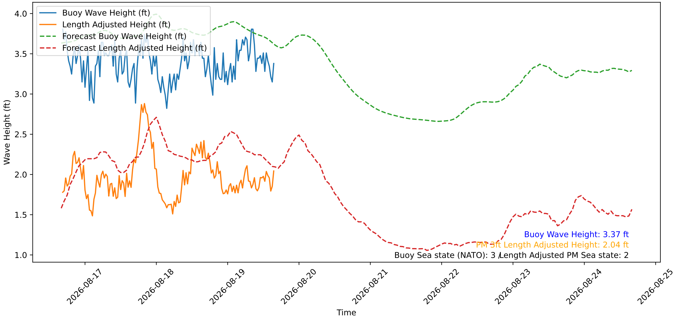
Wave Heights over Time for Oceanside Harbor at 2026-08-19 16:20:26
