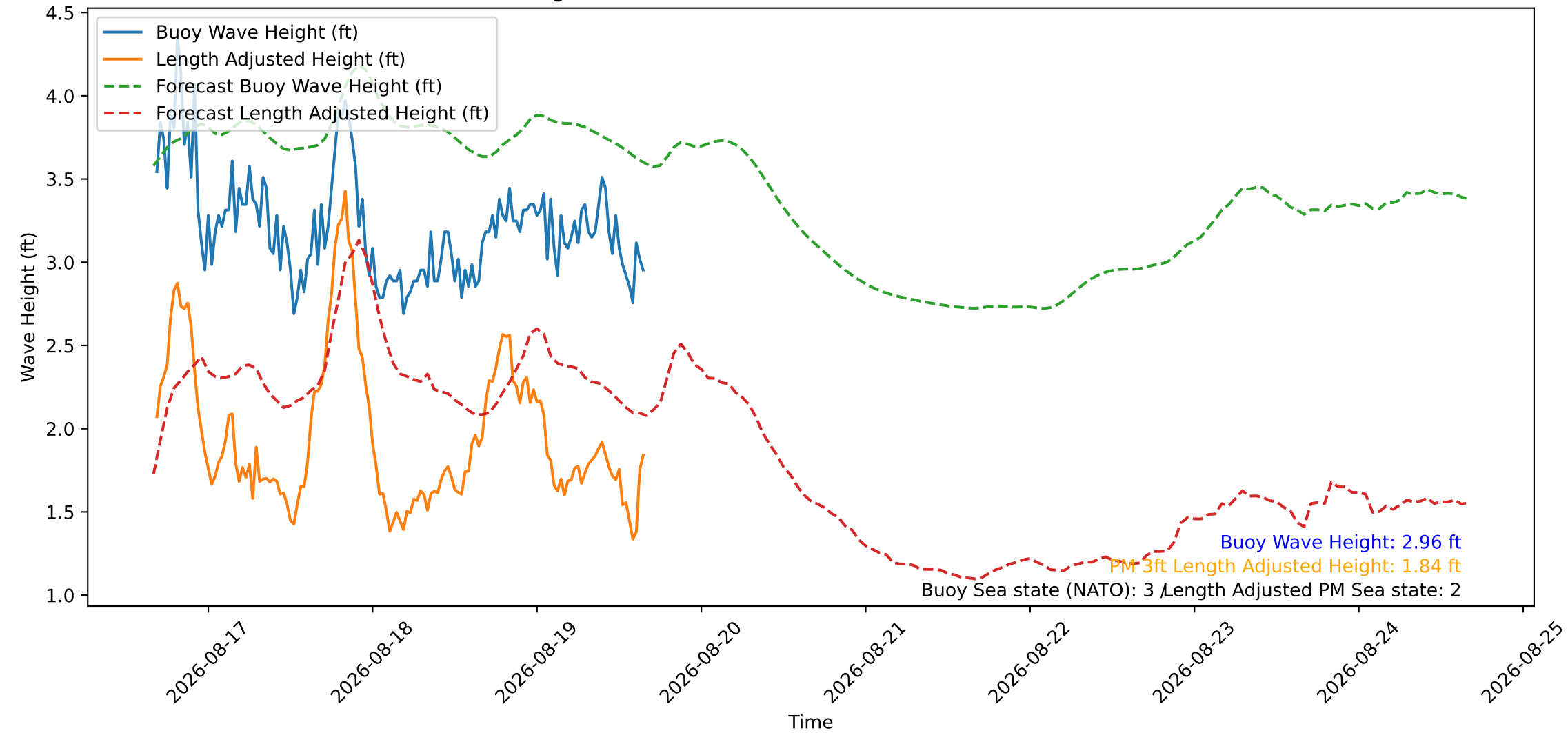
Wave Heights over Time for Green Beach at 2026-08-19 16:21:12
