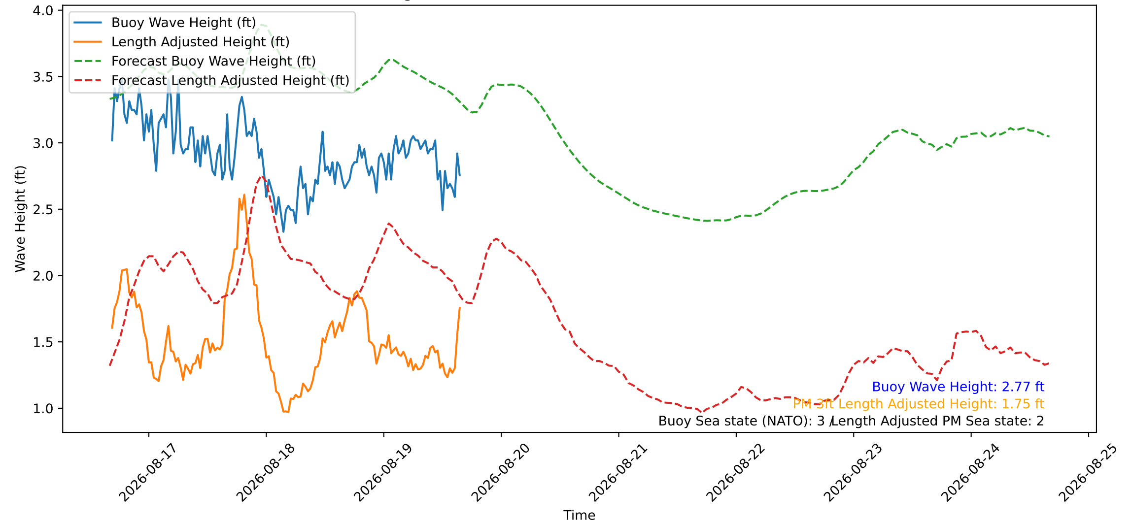
Wave Heights over Time for Red Beach at 2026-08-19 16:20:48
