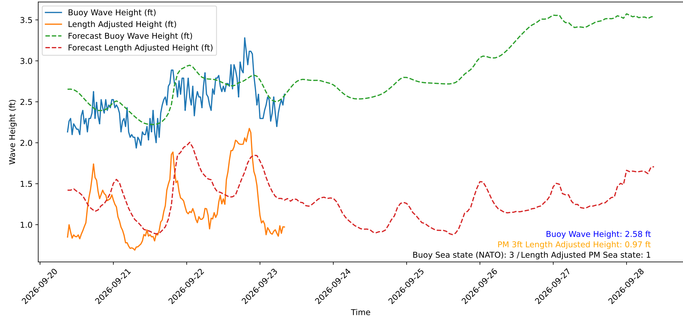
Wave Heights over Time for Red Beach at 2026-09-23 08:40:48
