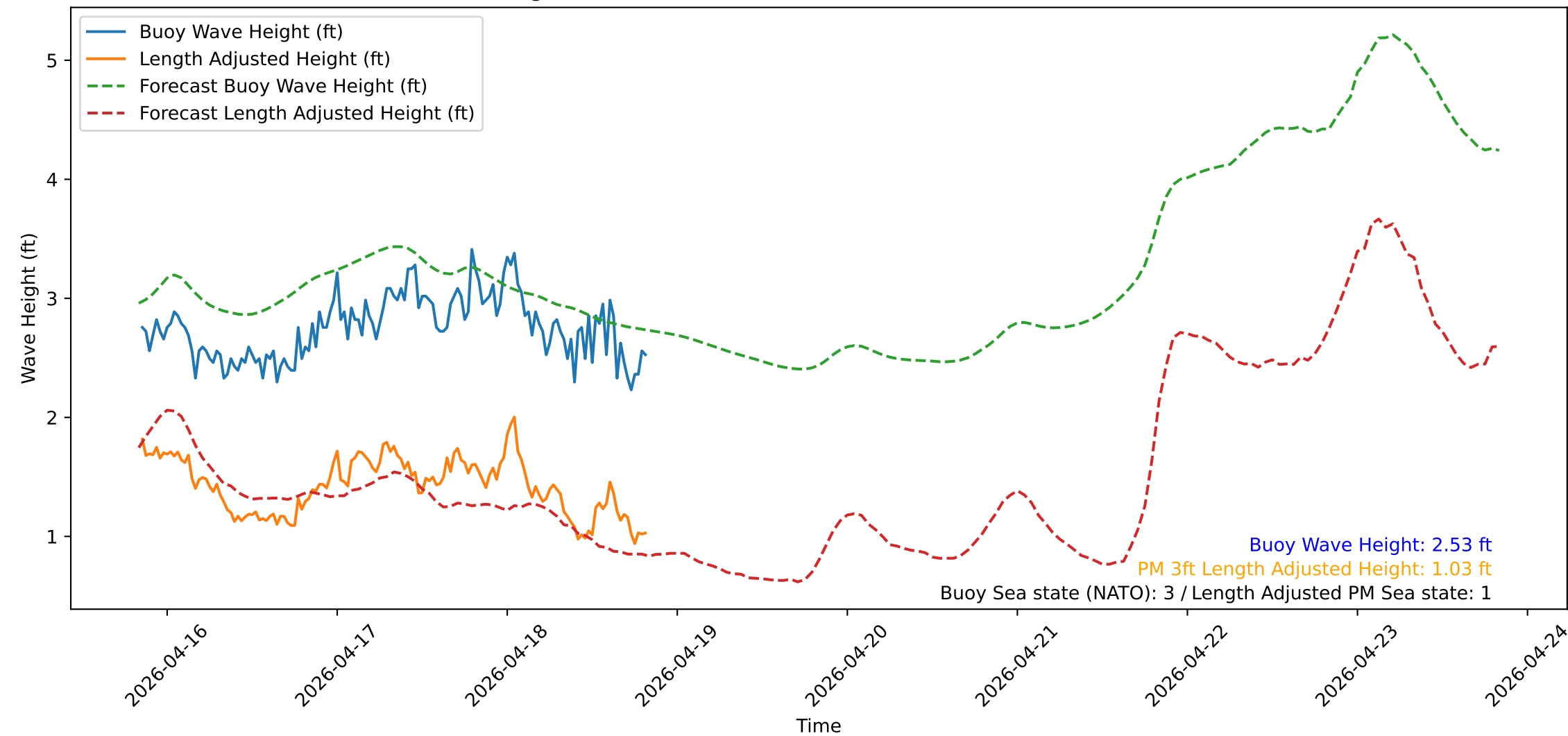
Wave Heights over Time for Oceanside Harbor at 2026-04-18 20:20:31
