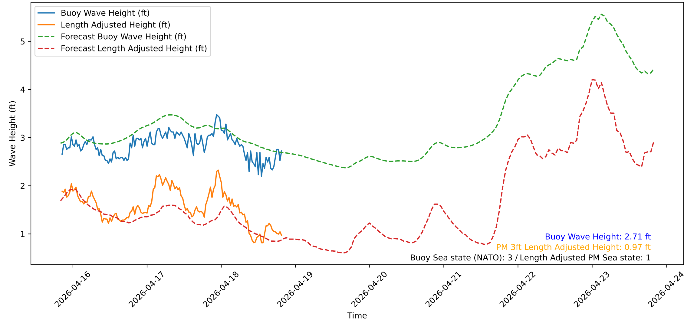
Wave Heights over Time for Green Beach at 2026-04-18 20:21:14
