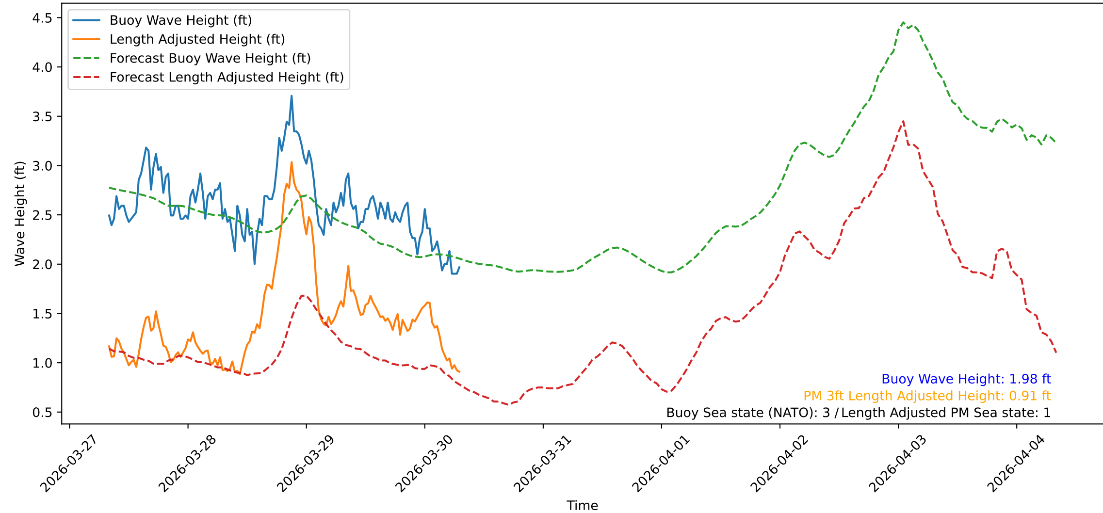
Wave Heights over Time for Green Beach at 2026-03-30 07:51:09
