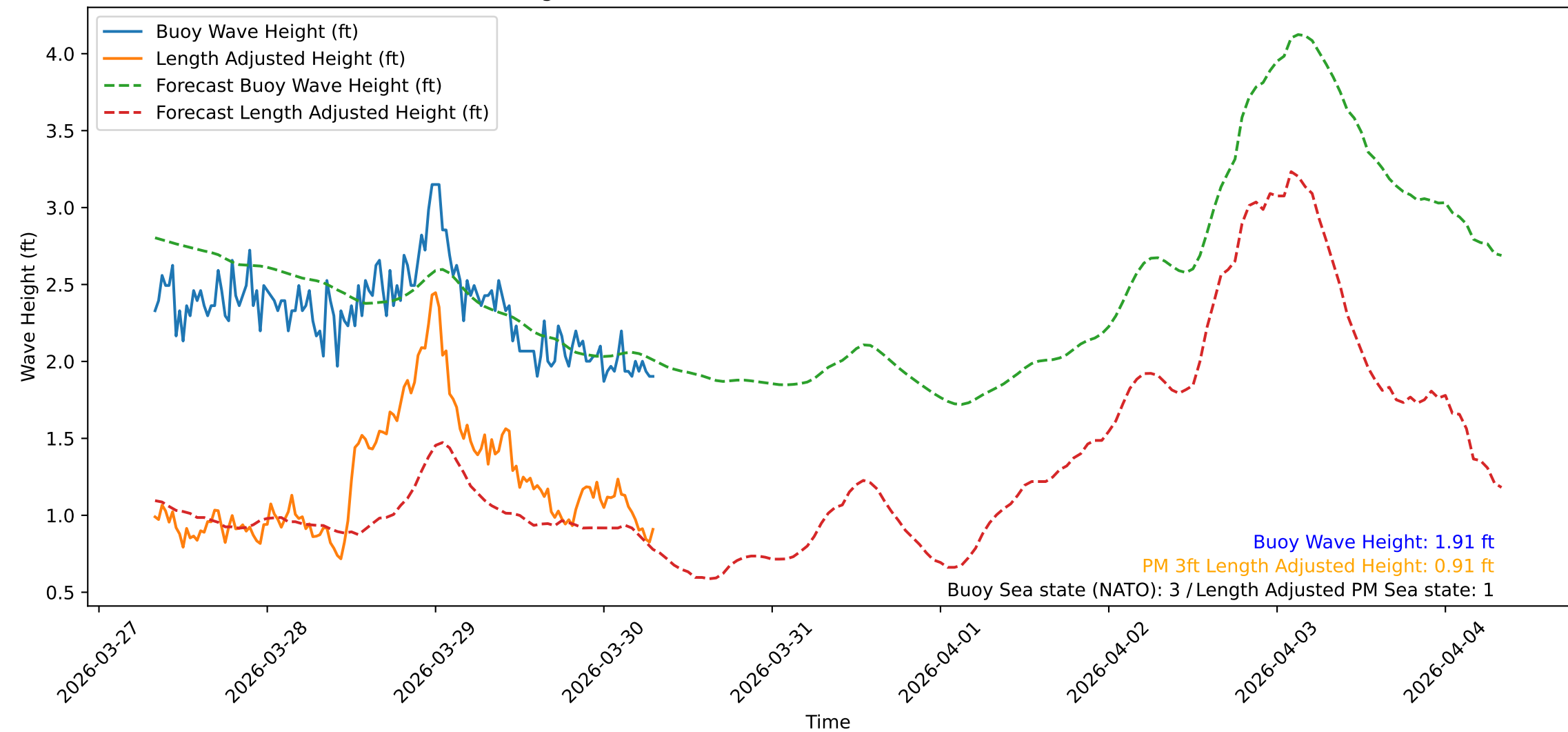
Wave Heights over Time for Oceanside Harbor at 2026-03-30 07:50:32
