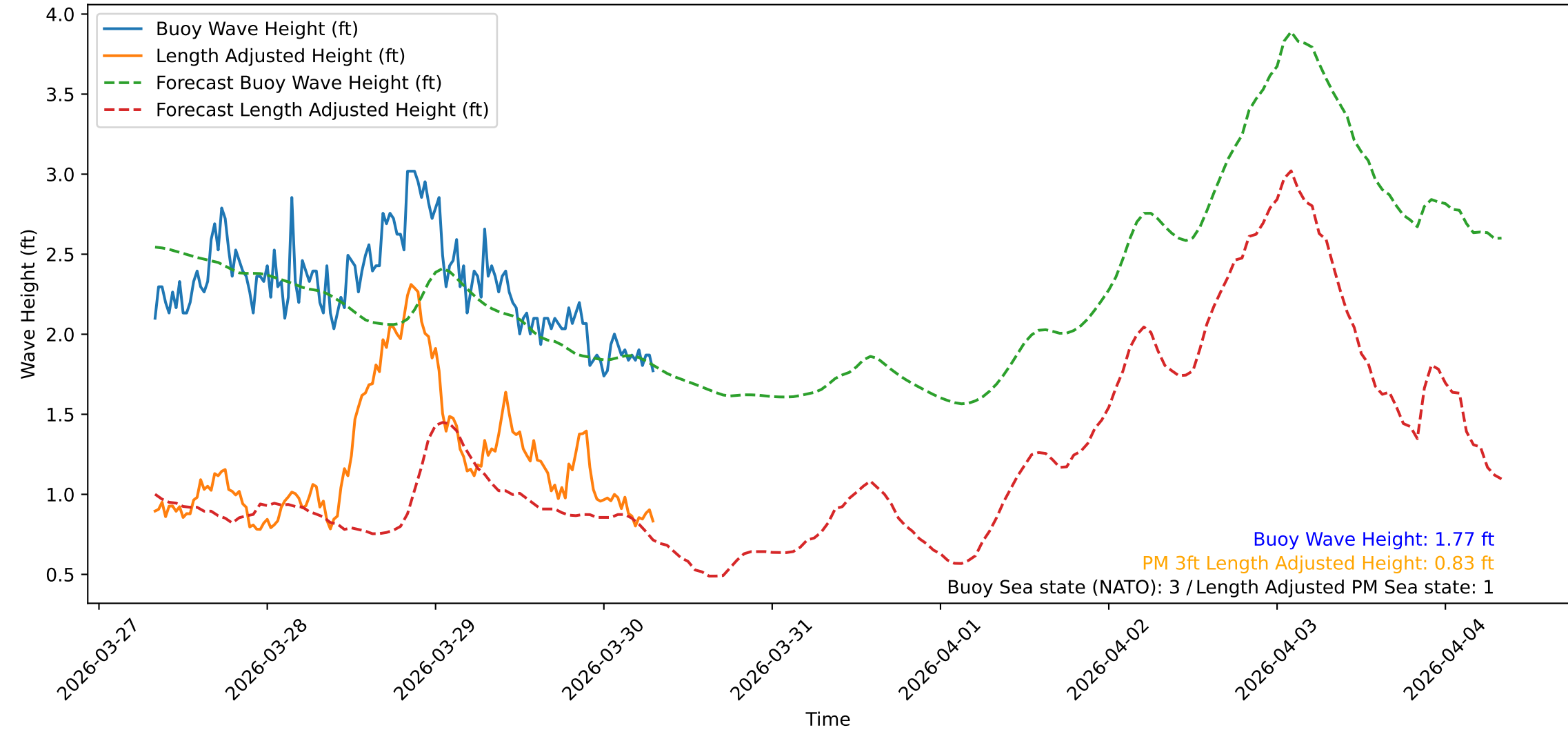
Wave Heights over Time for Red Beach at 2026-03-30 07:50:48
