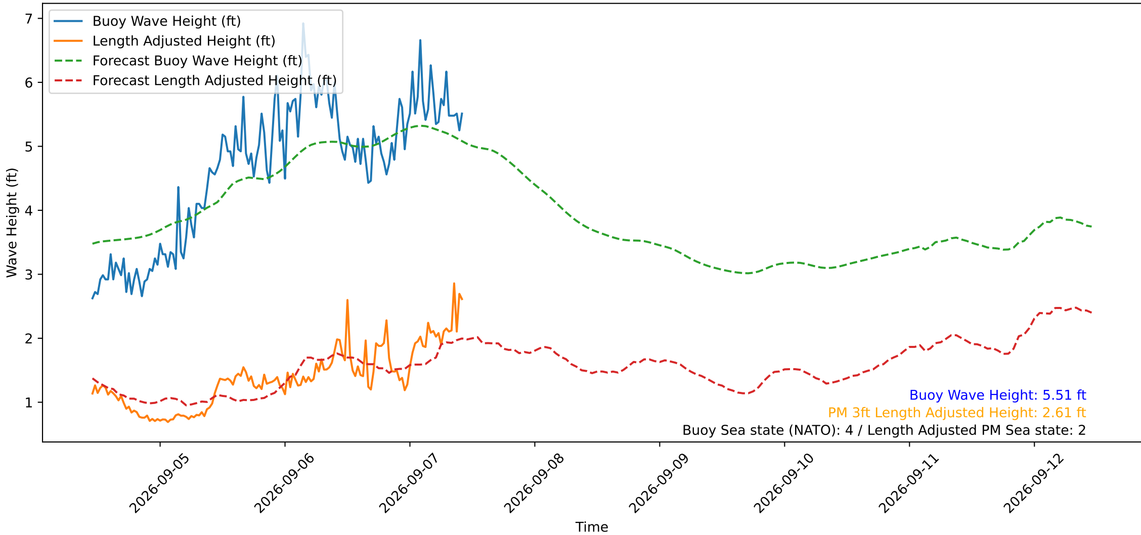
Wave Heights over Time for Red Beach at 2026-09-07 10:40:49
