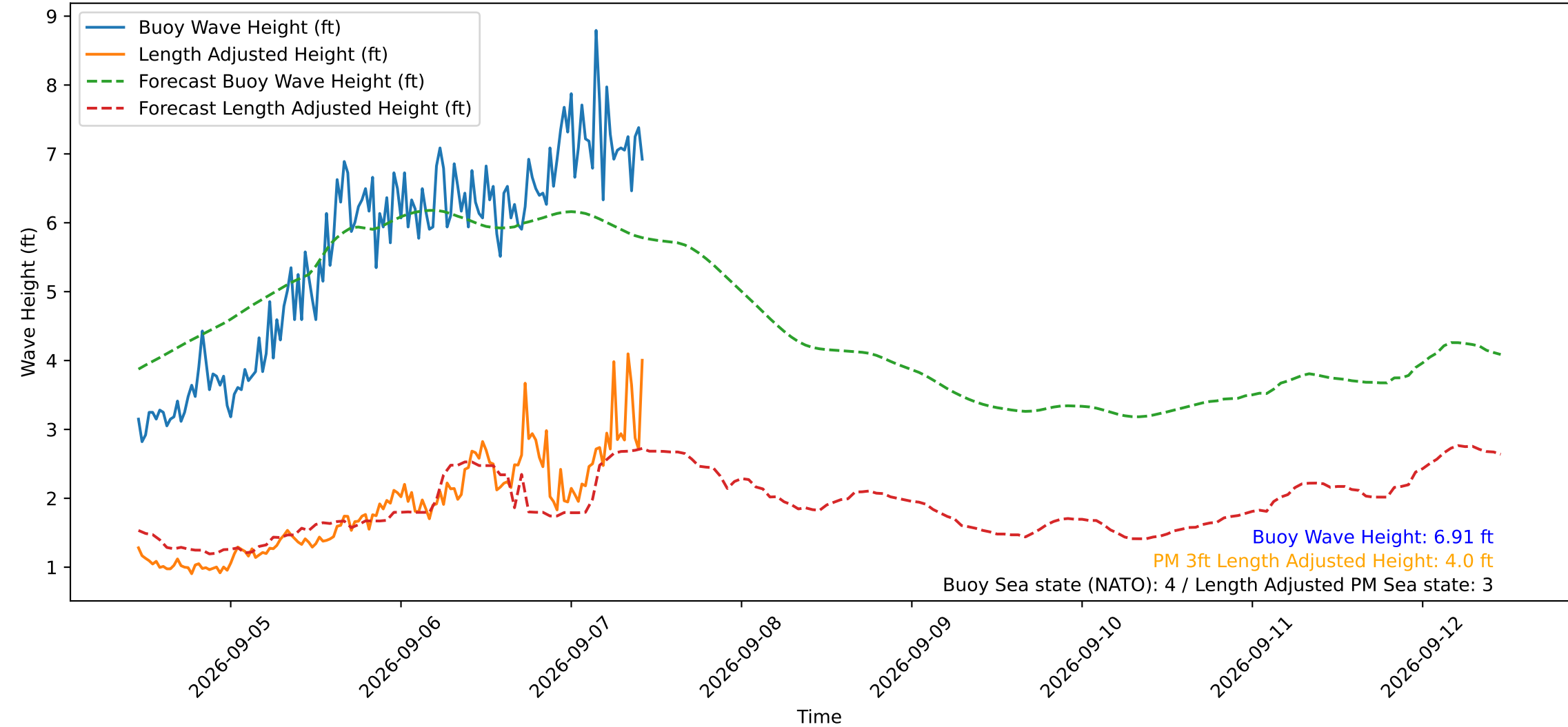
Wave Heights over Time for Green Beach at 2026-09-07 10:41:12
