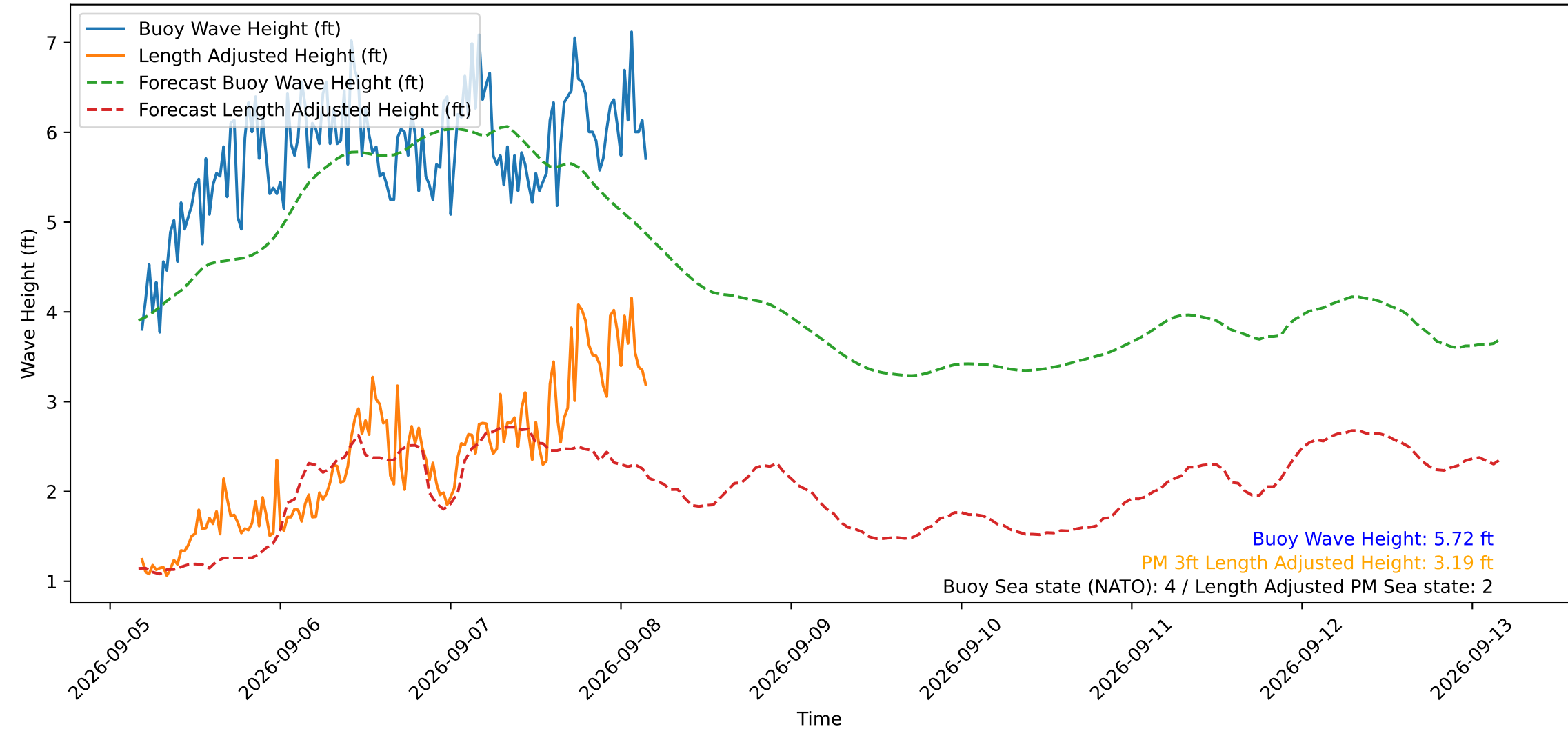
Wave Heights over Time for Oceanside Harbor at 2026-09-08 04:20:29
