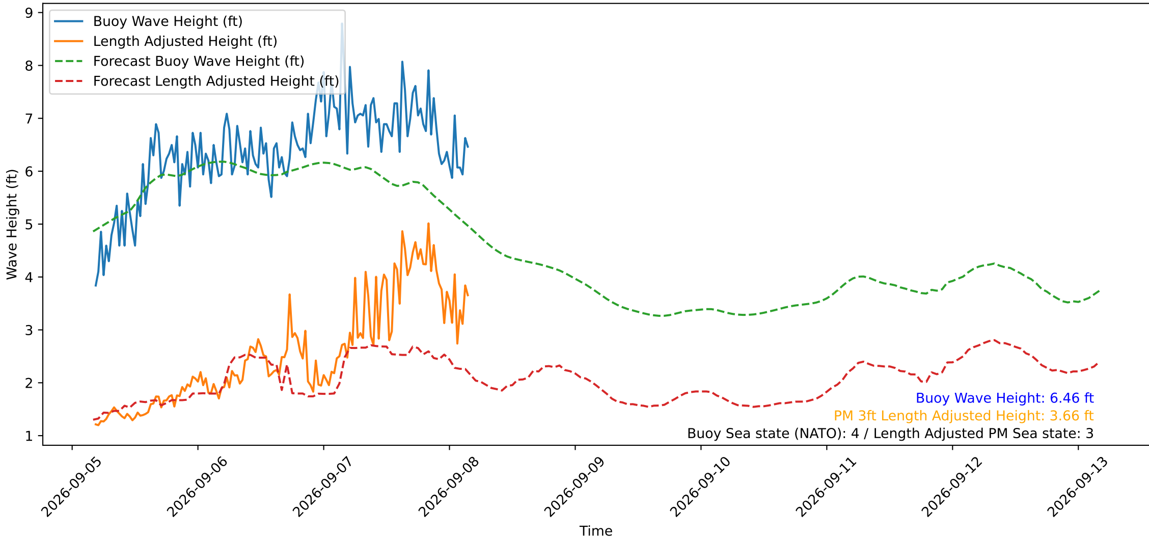
Wave Heights over Time for Green Beach at 2026-09-08 04:21:13
