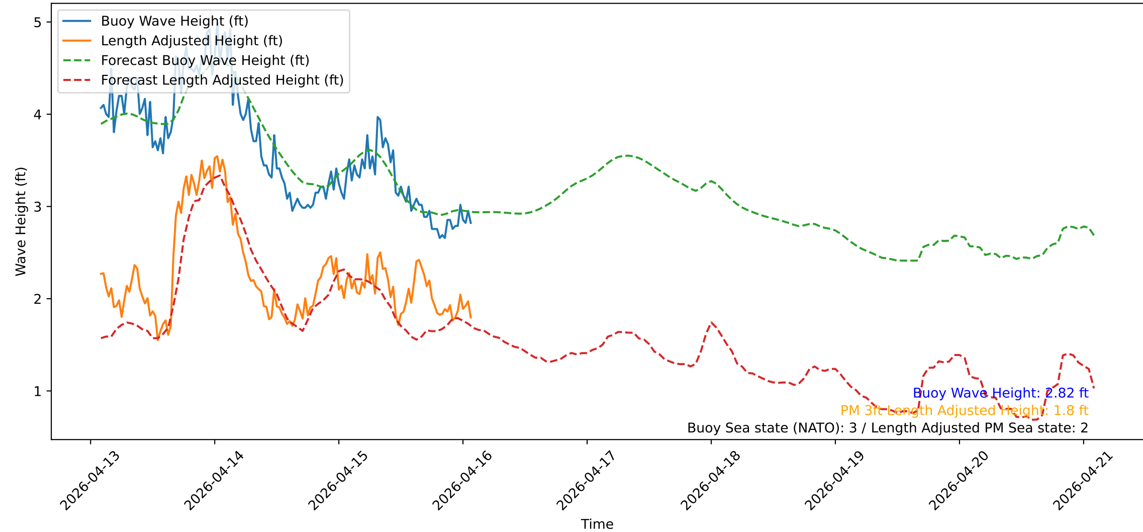
Wave Heights over Time for Green Beach at 2026-04-16 02:11:13
