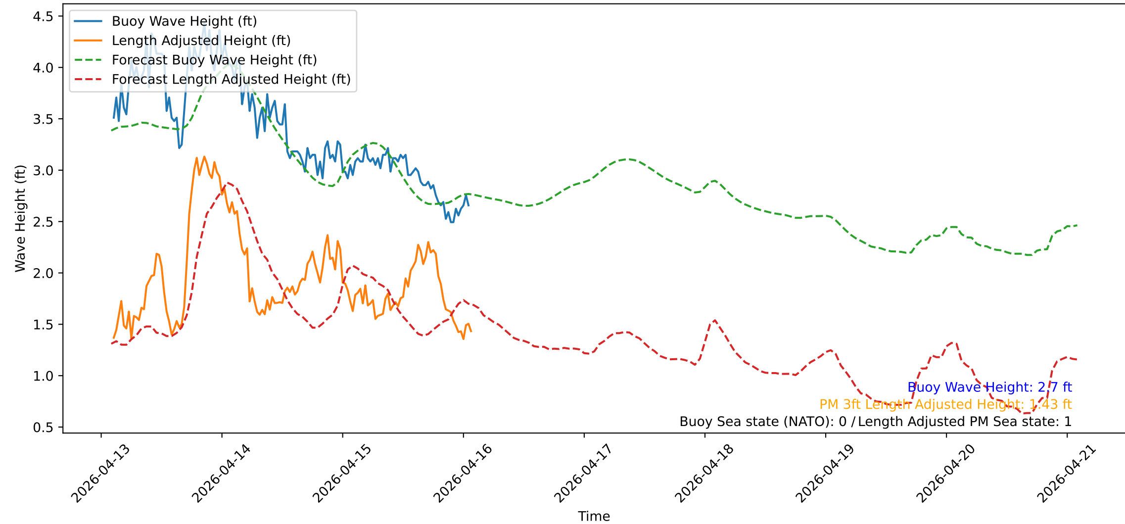
Wave Heights over Time for Red Beach at 2026-04-16 02:10:50
