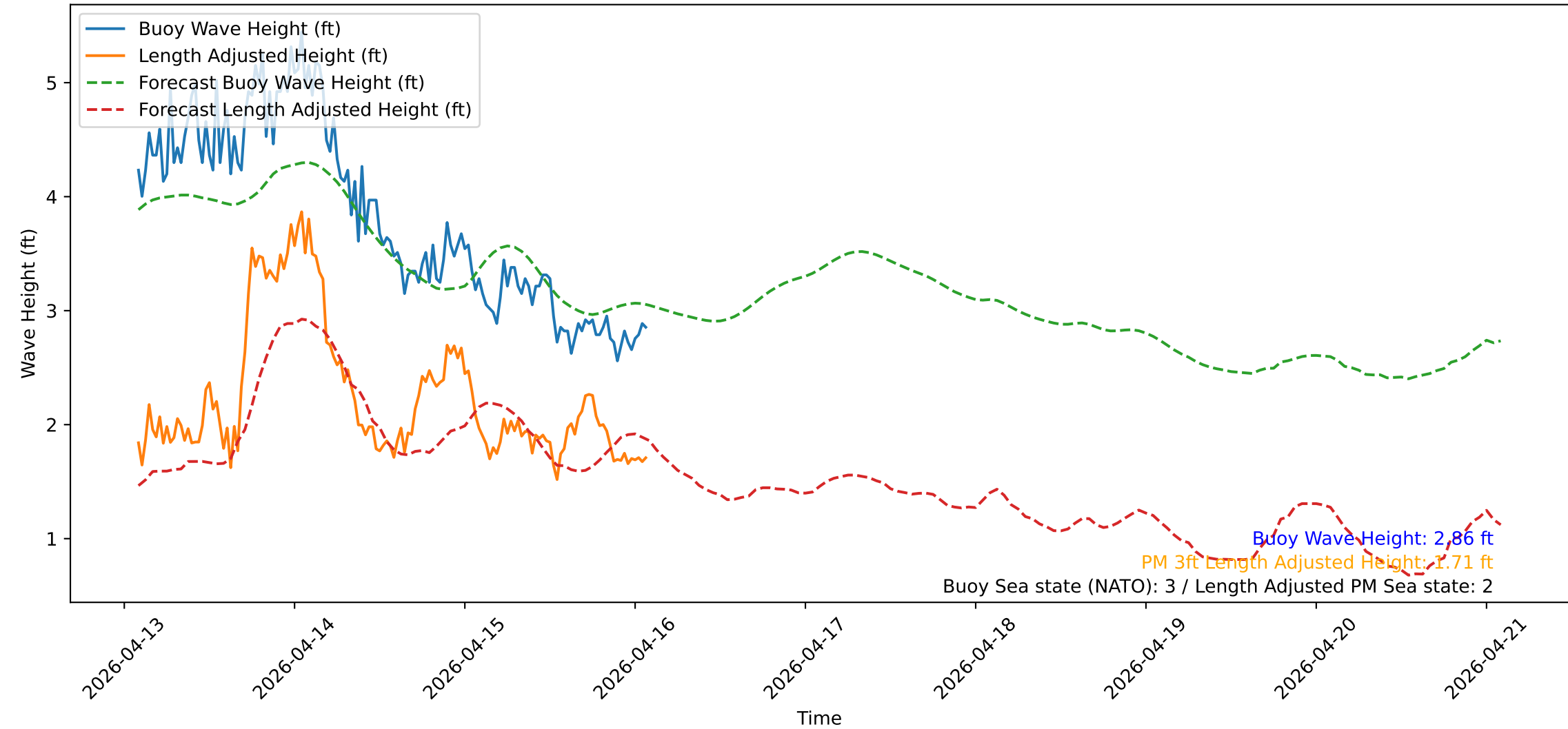
Wave Heights over Time for Oceanside Harbor at 2026-04-16 02:10:31
