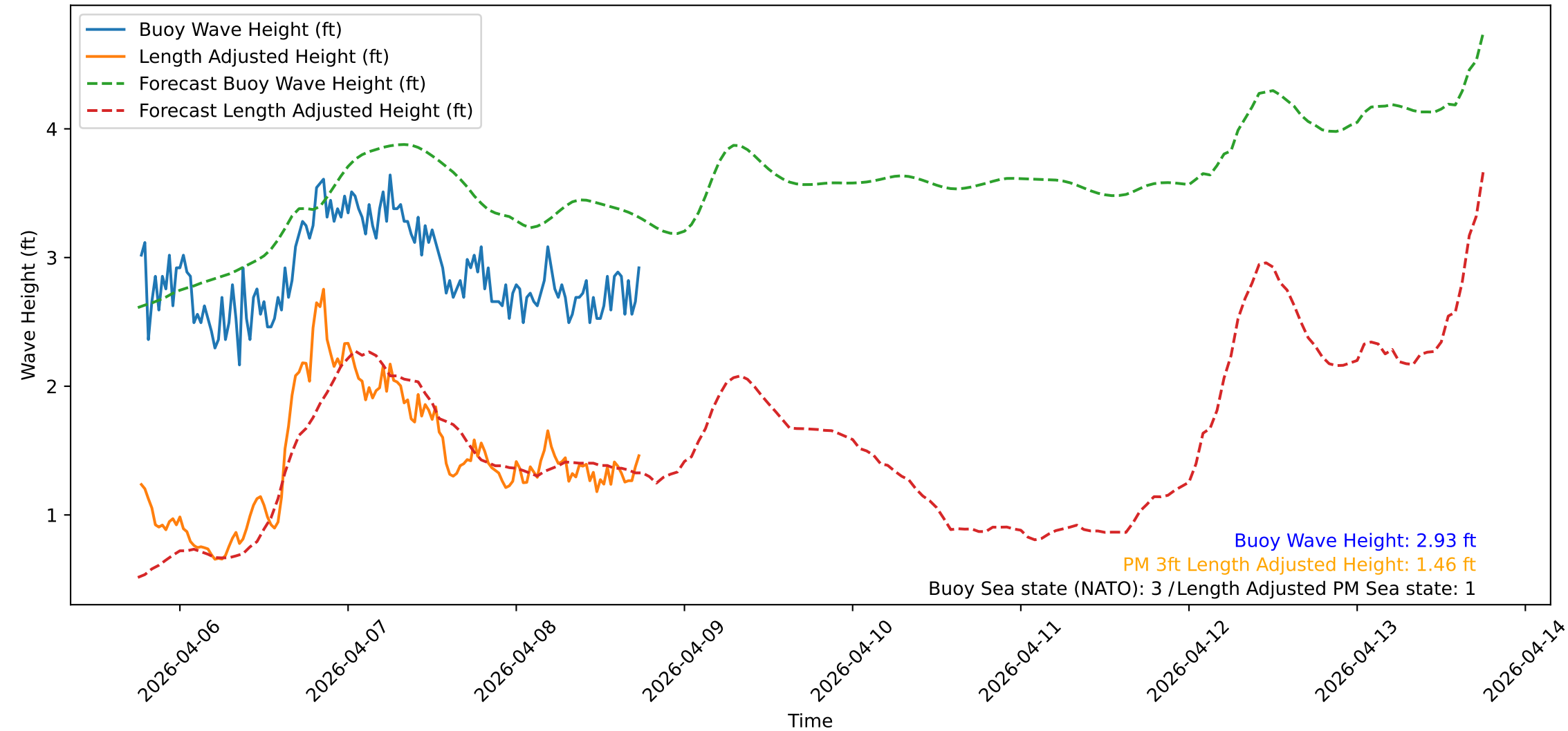
Wave Heights over Time for Oceanside Harbor at 2026-04-08 18:20:31
