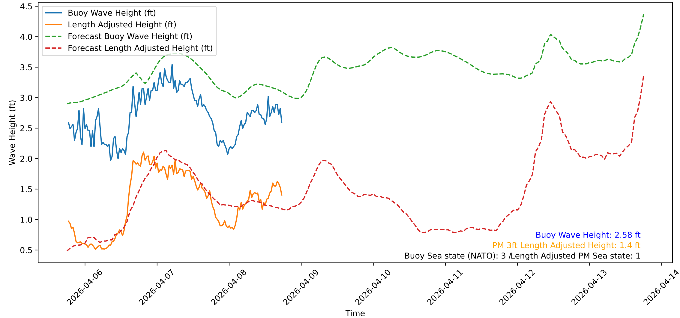
Wave Heights over Time for Red Beach at 2026-04-08 18:20:47
