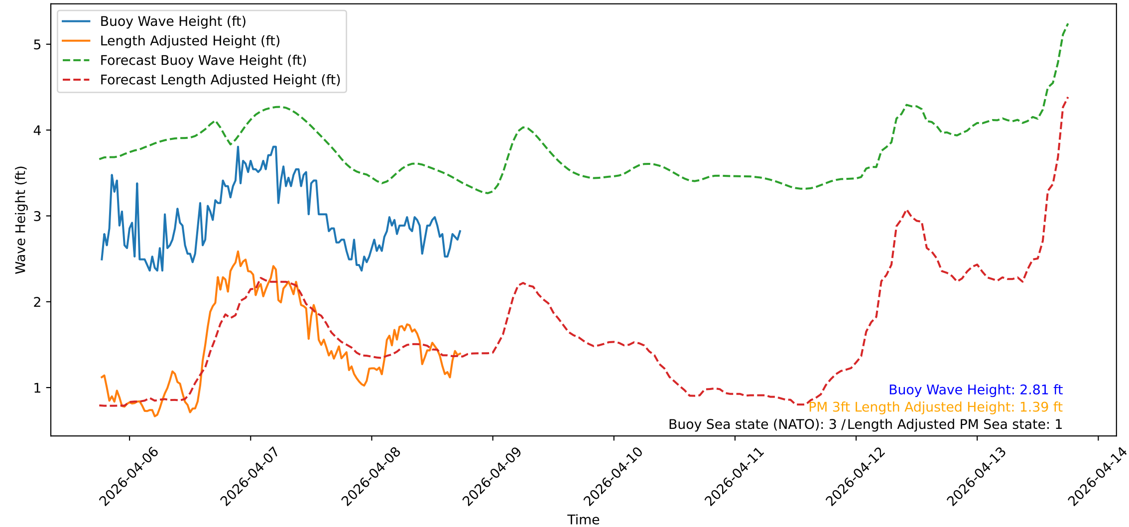
Wave Heights over Time for Green Beach at 2026-04-08 18:21:09
