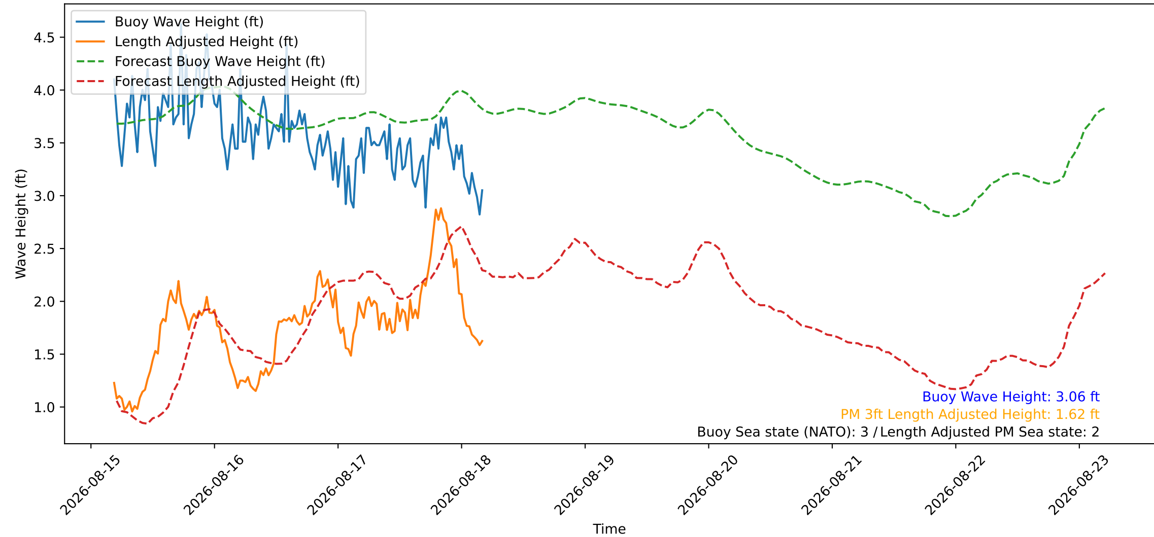
Wave Heights over Time for Oceanside Harbor at 2026-08-18 04:40:26
