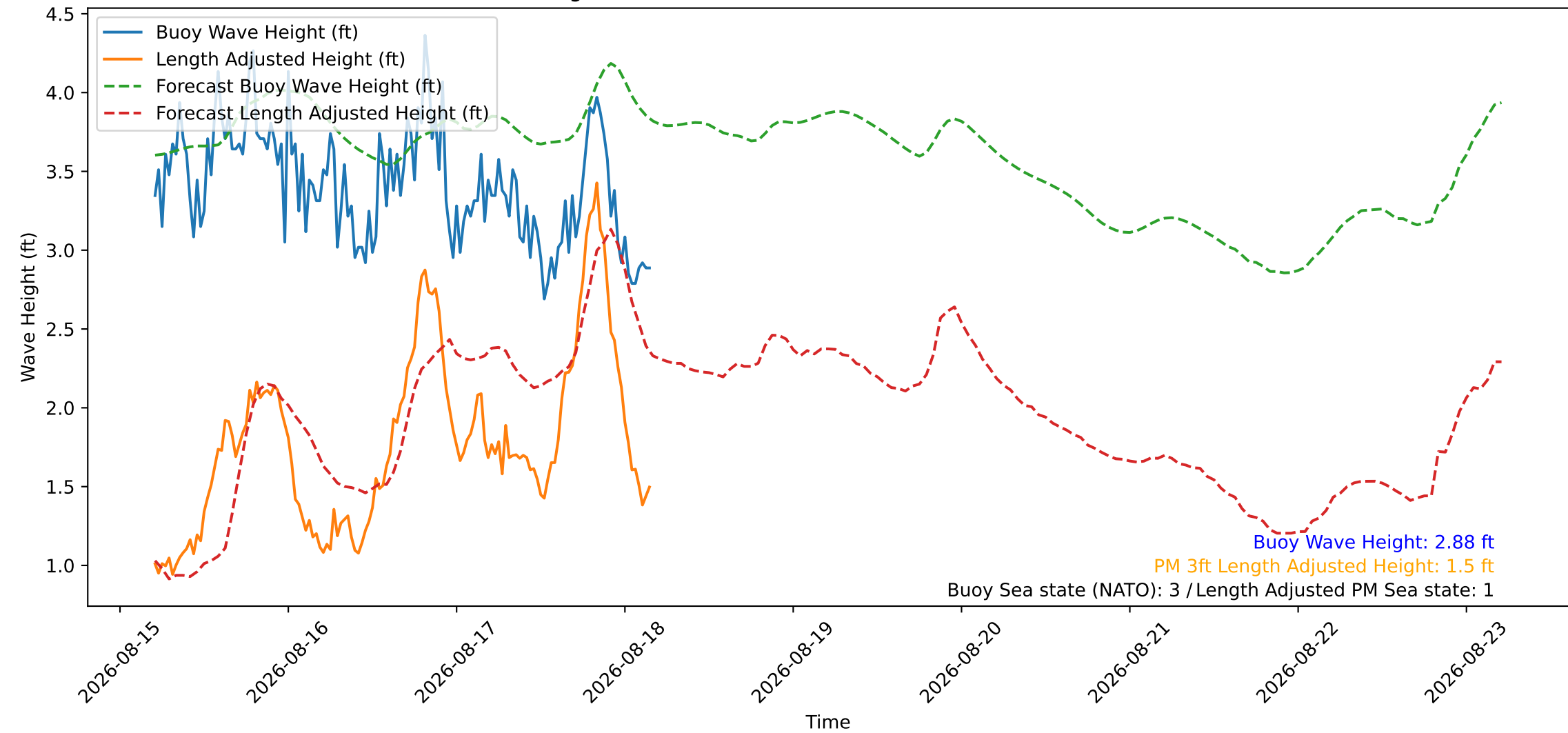
Wave Heights over Time for Green Beach at 2026-08-18 04:41:08
