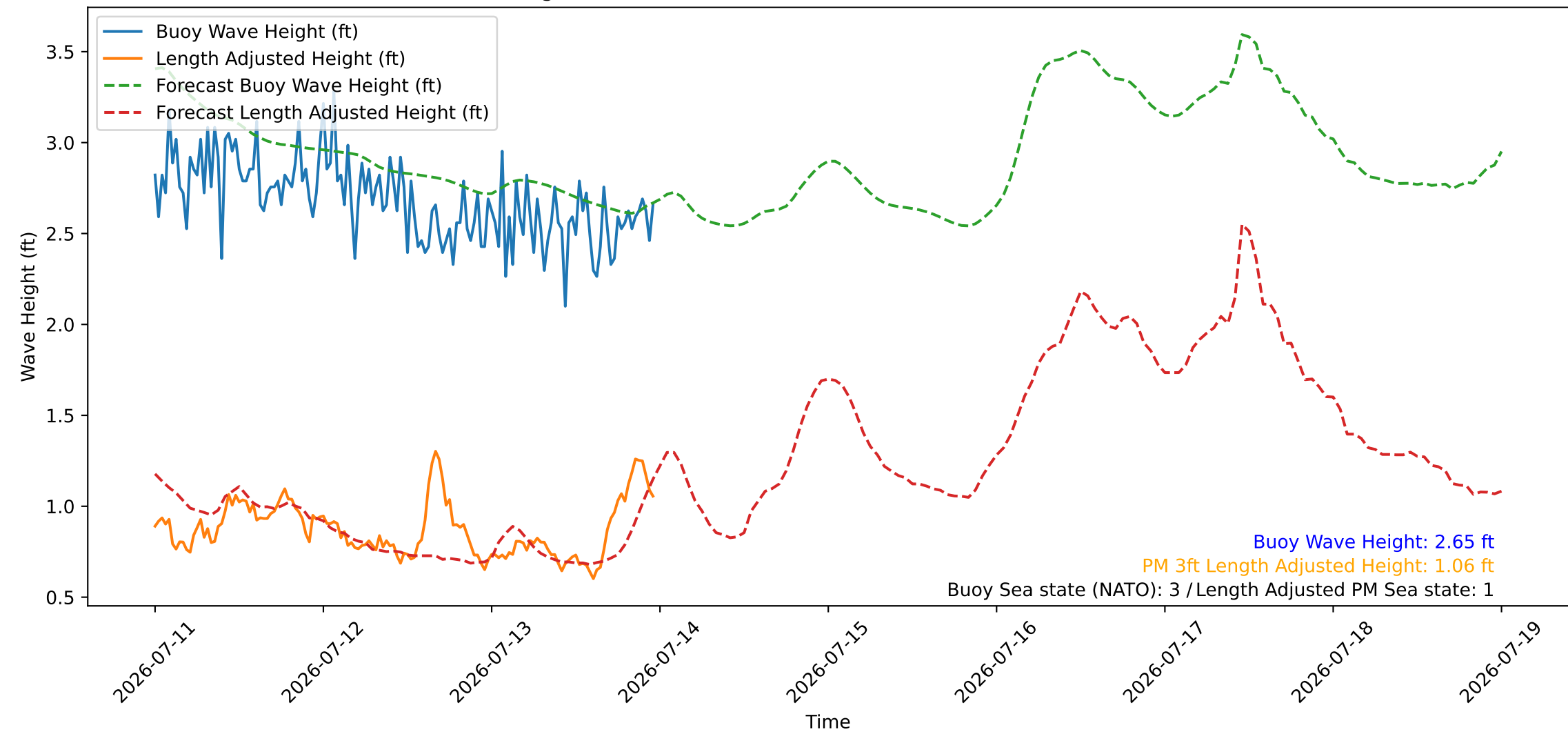
Wave Heights over Time for Oceanside Harbor at 2026-07-14 00:00:26
