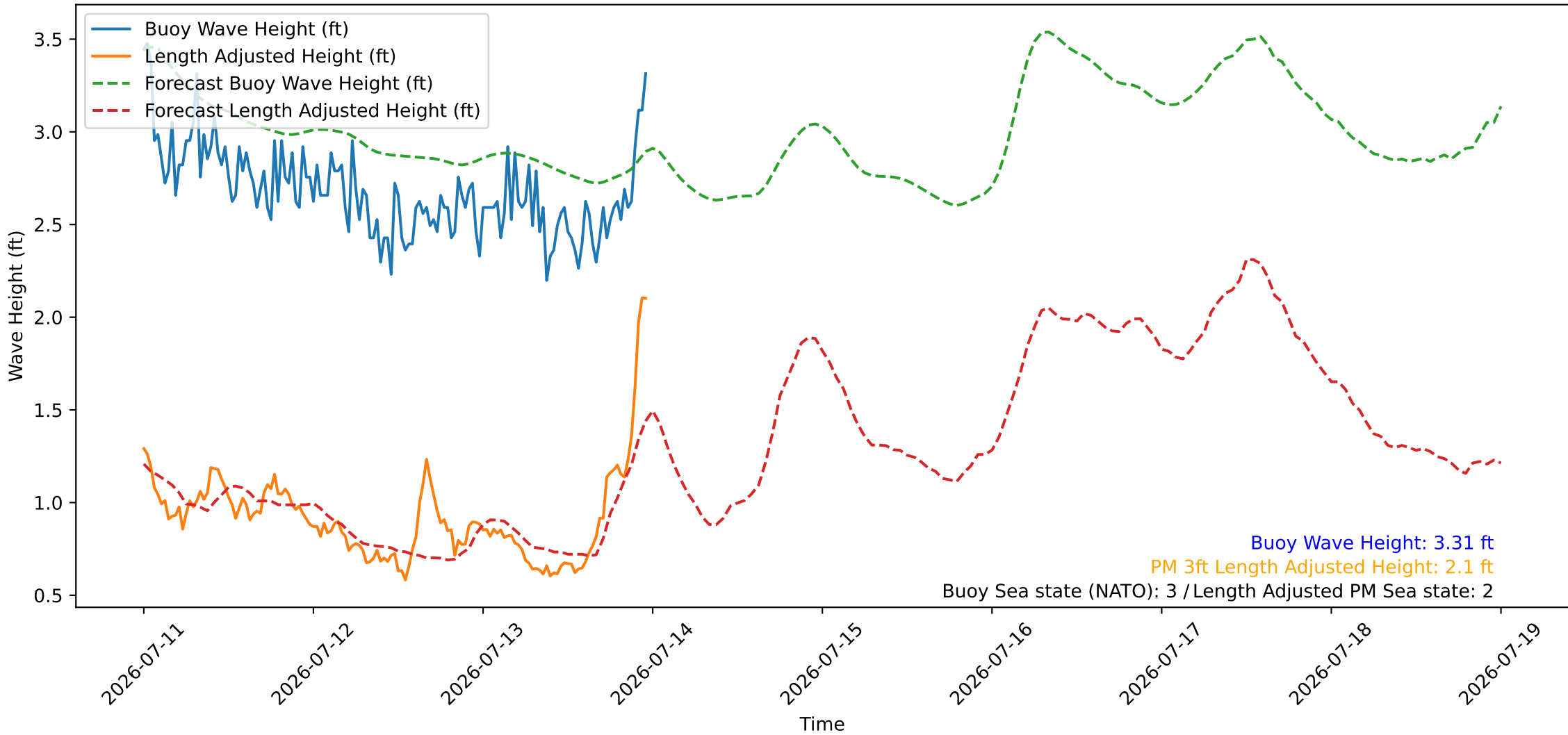
Wave Heights over Time for Green Beach at 2026-07-14 00:01:07
