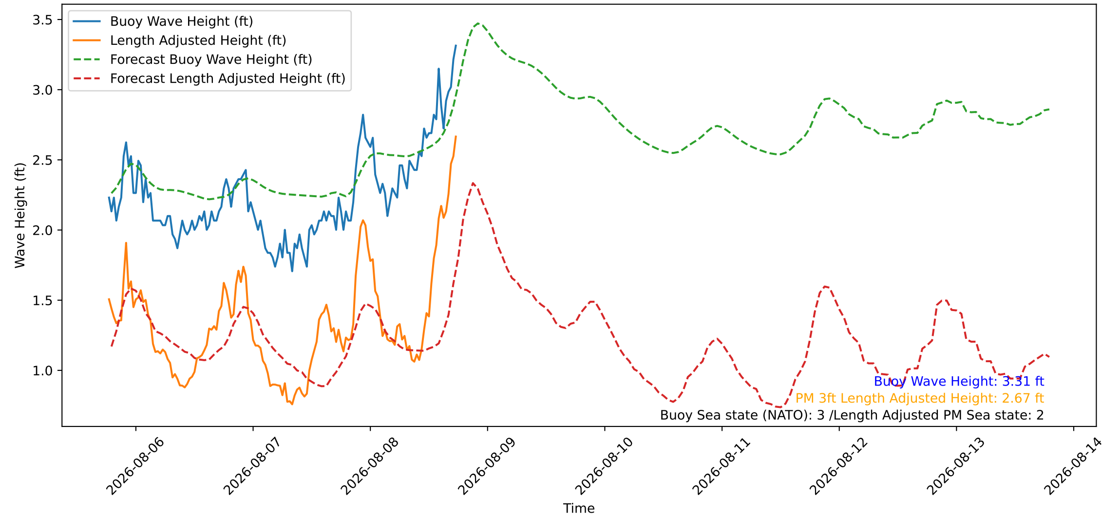
Wave Heights over Time for Green Beach at 2026-08-08 18:31:08
