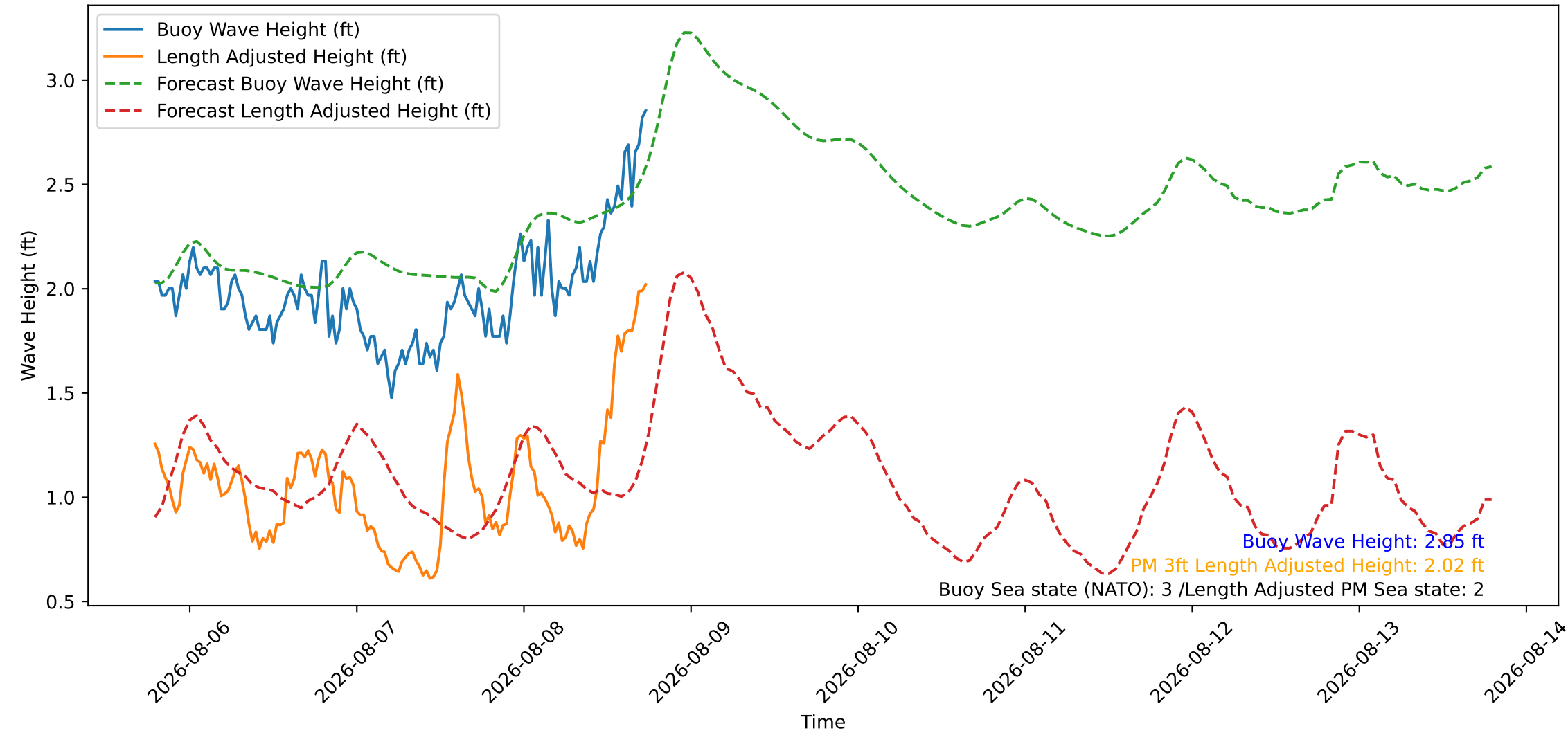
Wave Heights over Time for Red Beach at 2026-08-08 18:30:45
