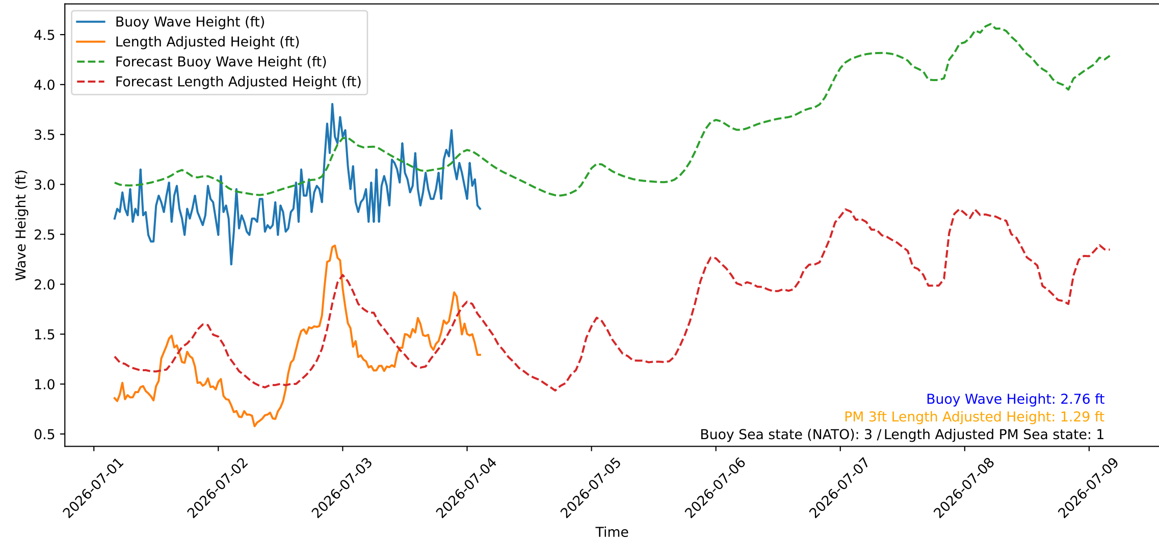
Wave Heights over Time for Red Beach at 2026-07-04 03:30:46
