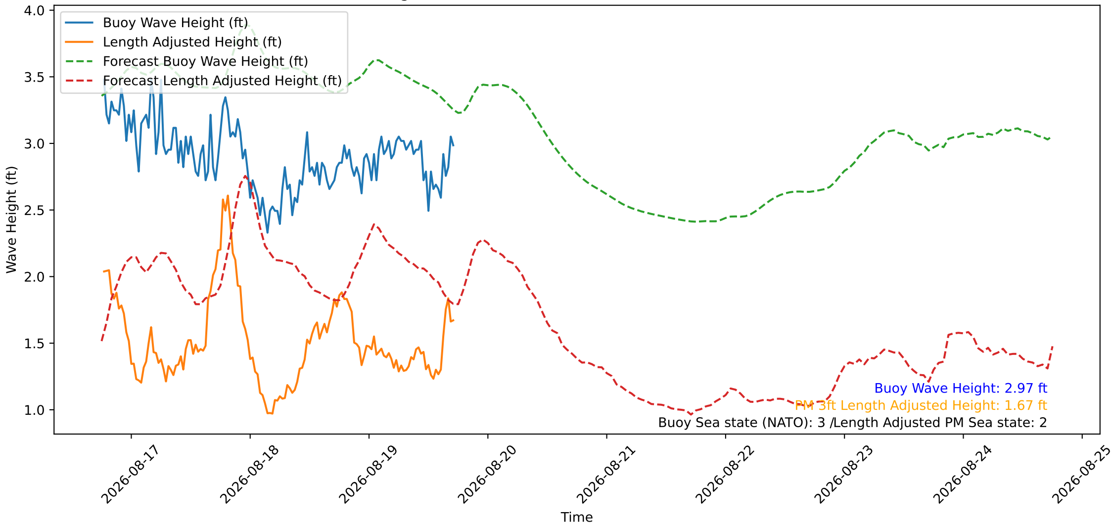
Wave Heights over Time for Red Beach at 2026-08-19 18:00:46
