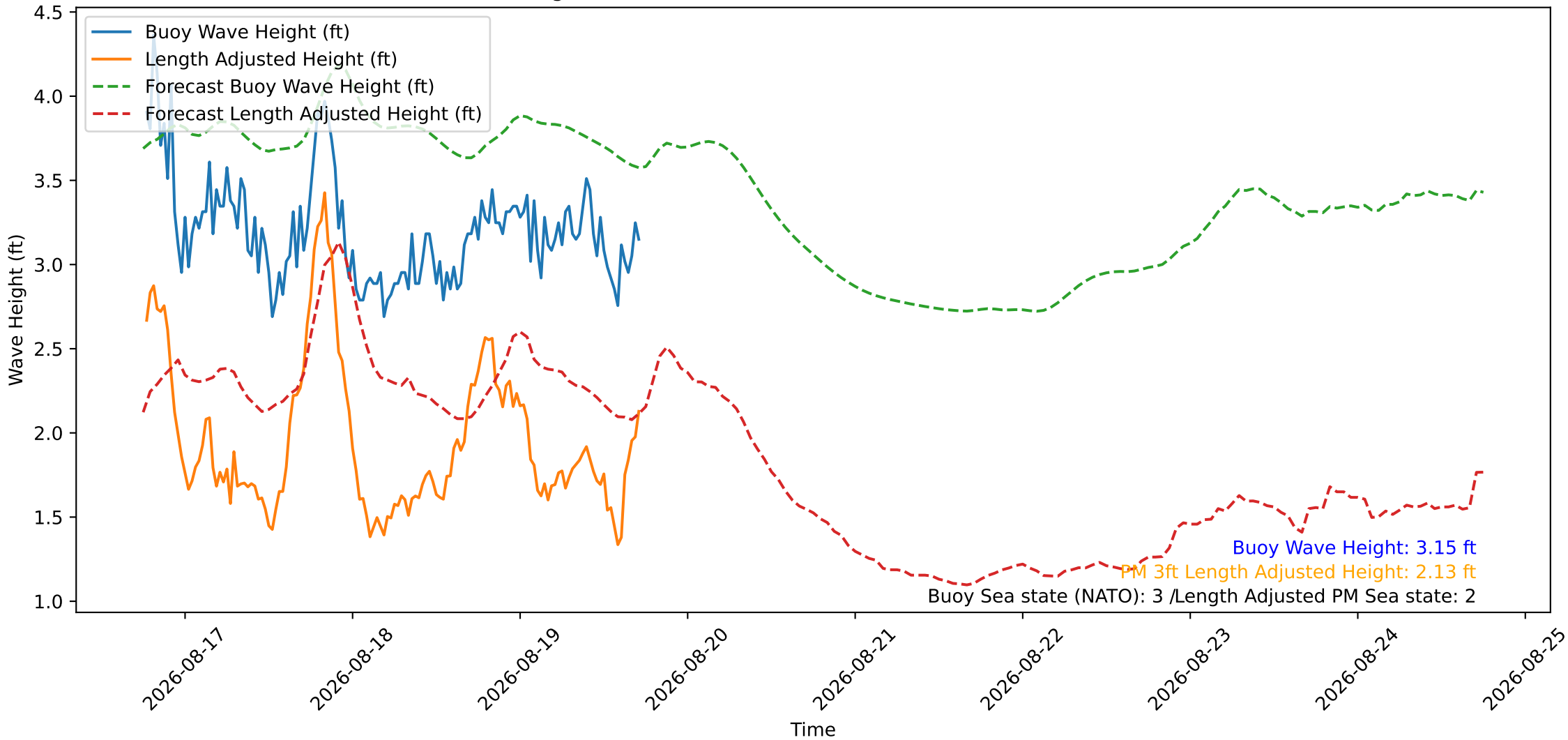
Wave Heights over Time for Green Beach at 2026-08-19 18:01:11
