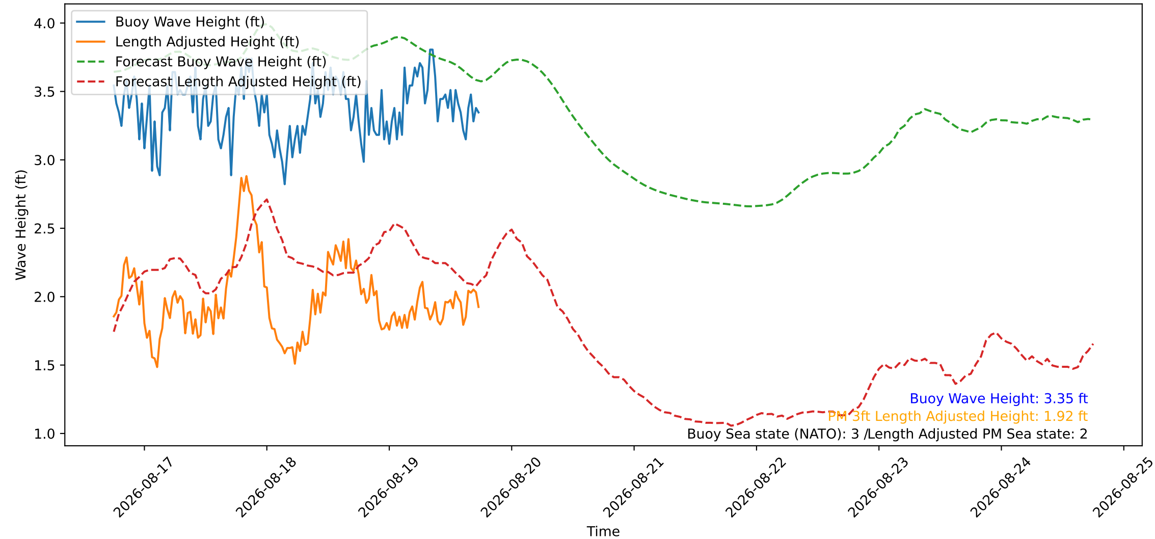
Wave Heights over Time for Oceanside Harbor at 2026-08-19 18:00:27
