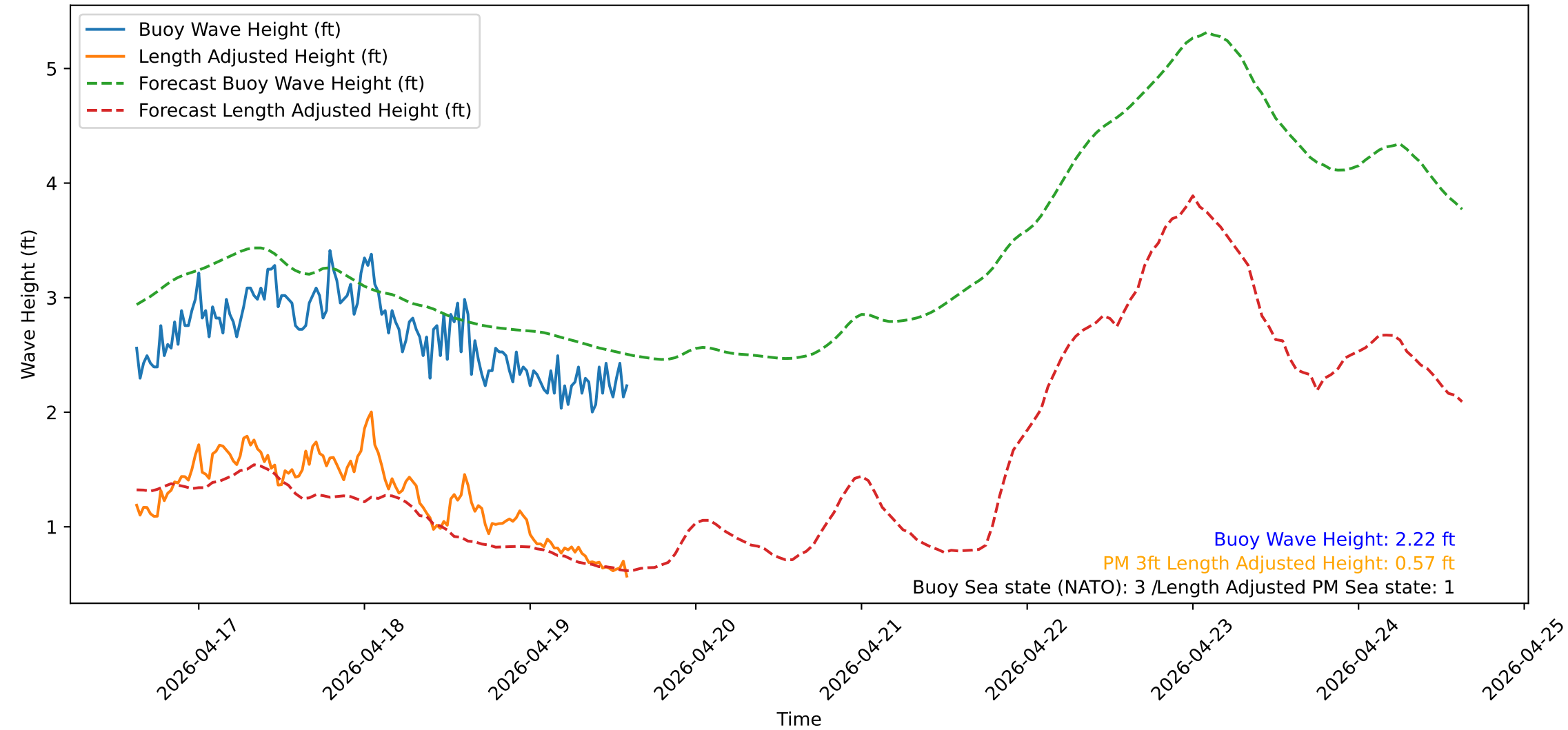
Wave Heights over Time for Oceanside Harbor at 2026-04-19 15:10:31
