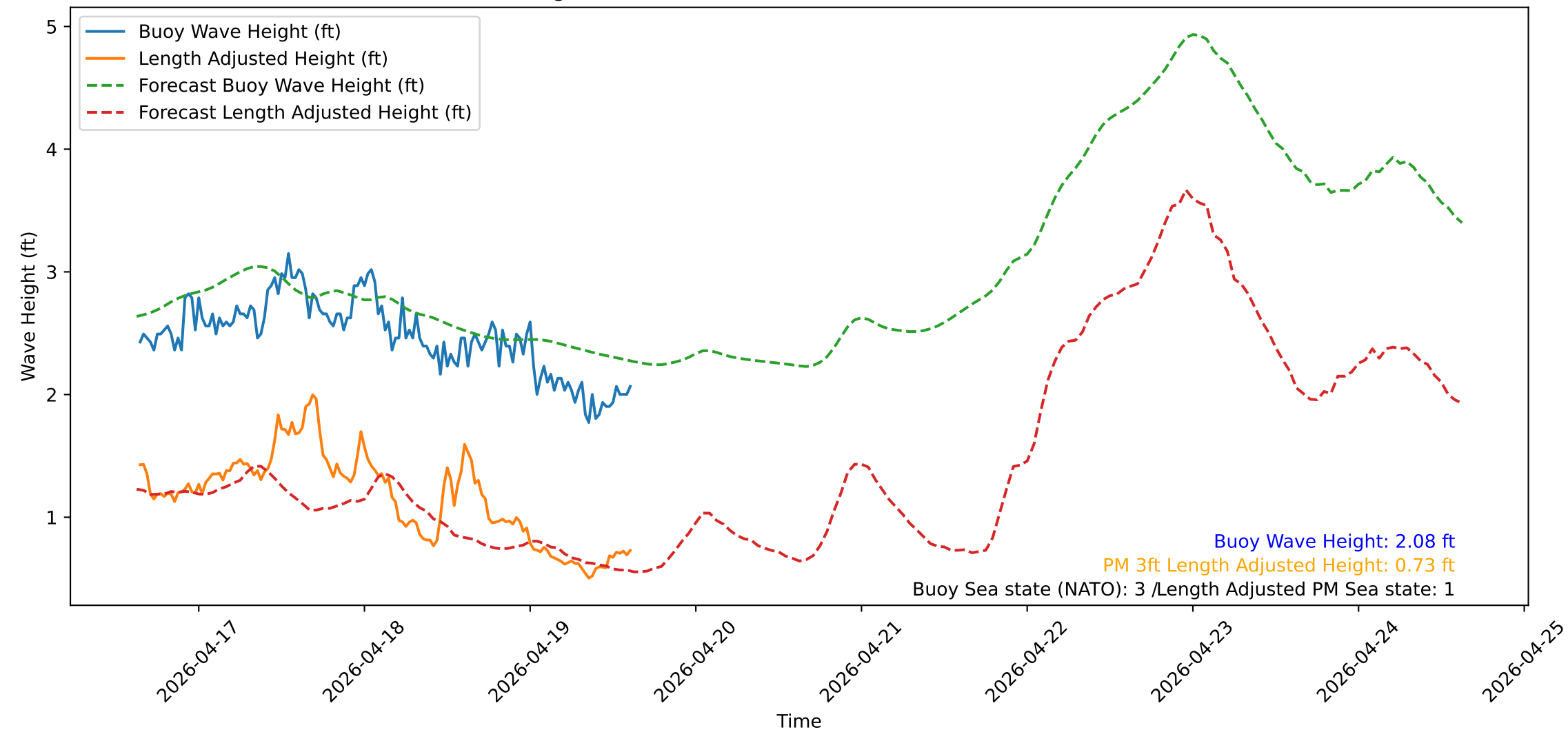
Wave Heights over Time for Red Beach at 2026-04-19 15:10:50
