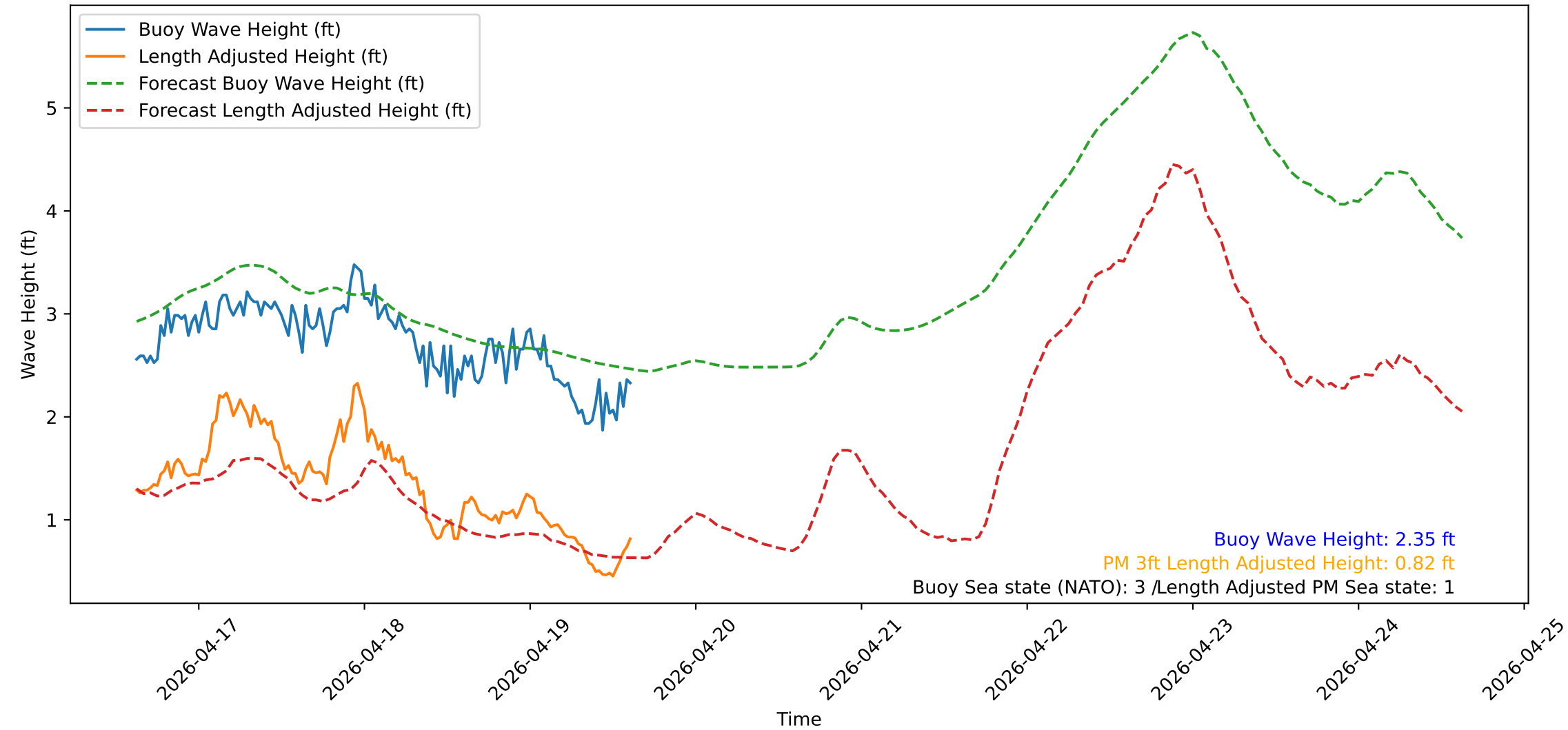
Wave Heights over Time for Green Beach at 2026-04-19 15:11:13
