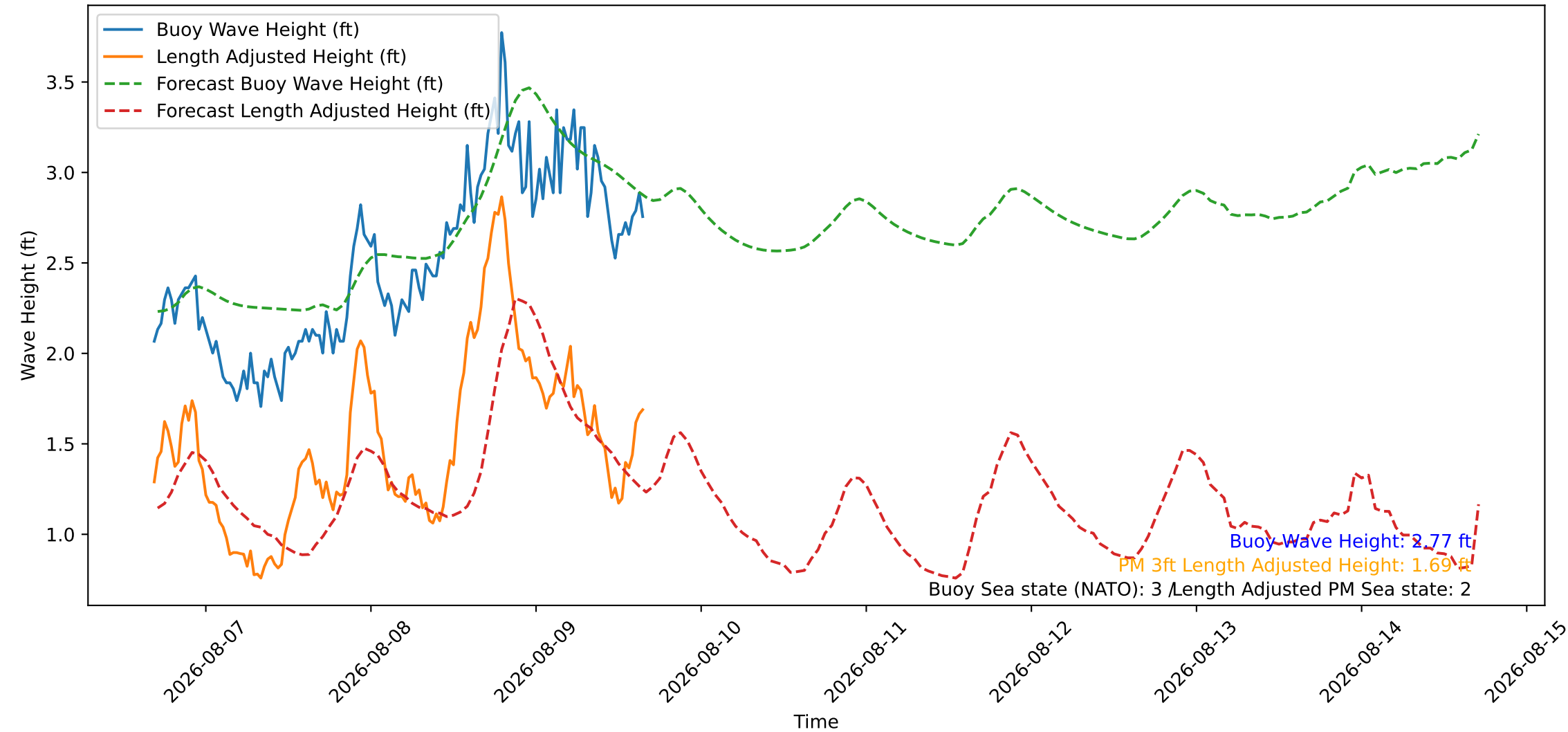
Wave Heights over Time for Green Beach at 2026-08-09 16:31:09
