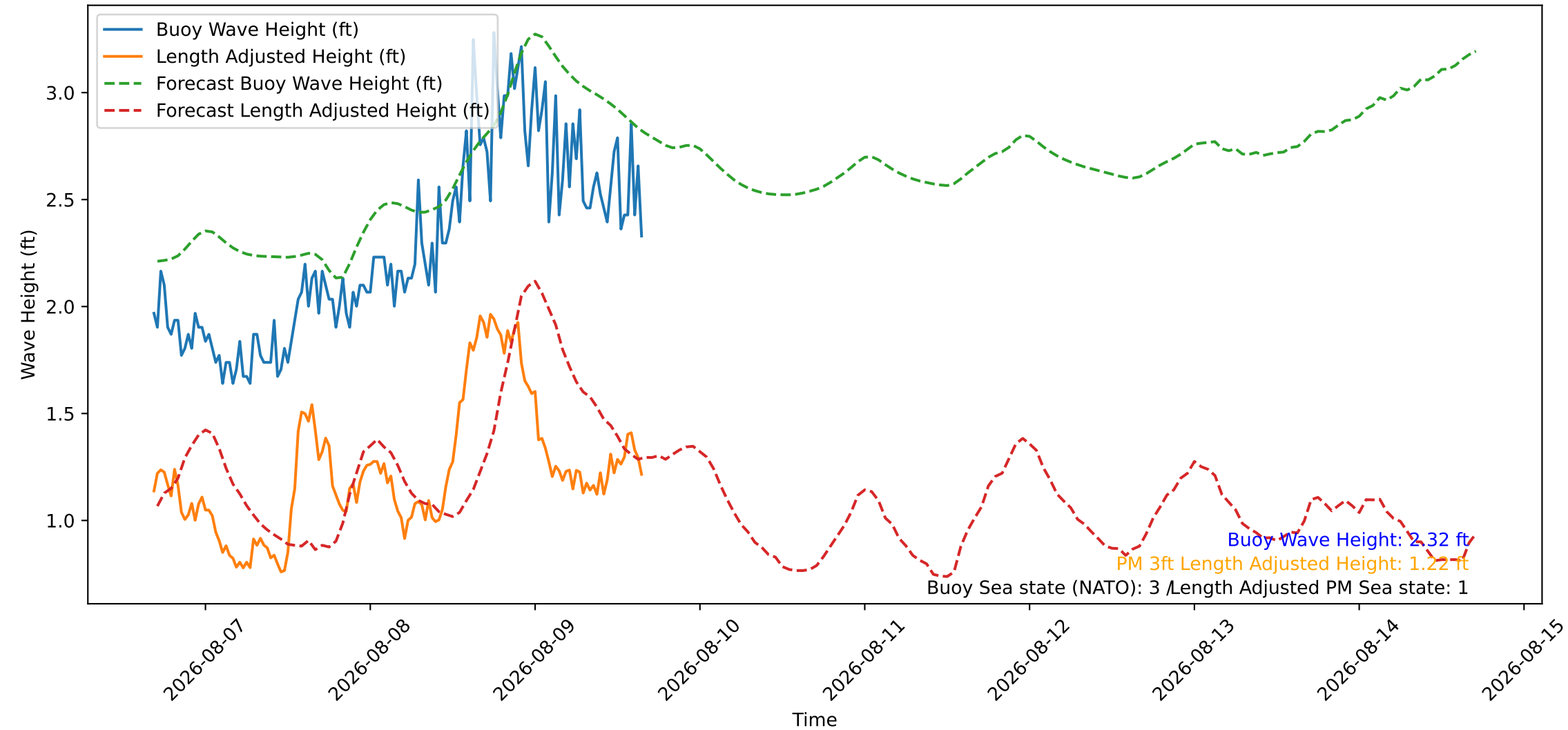
Wave Heights over Time for Oceanside Harbor at 2026-08-09 16:30:27
