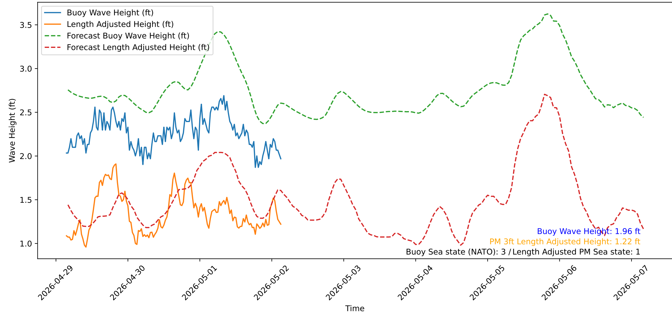
Wave Heights over Time for Oceanside Harbor at 2026-05-02 03:40:31
