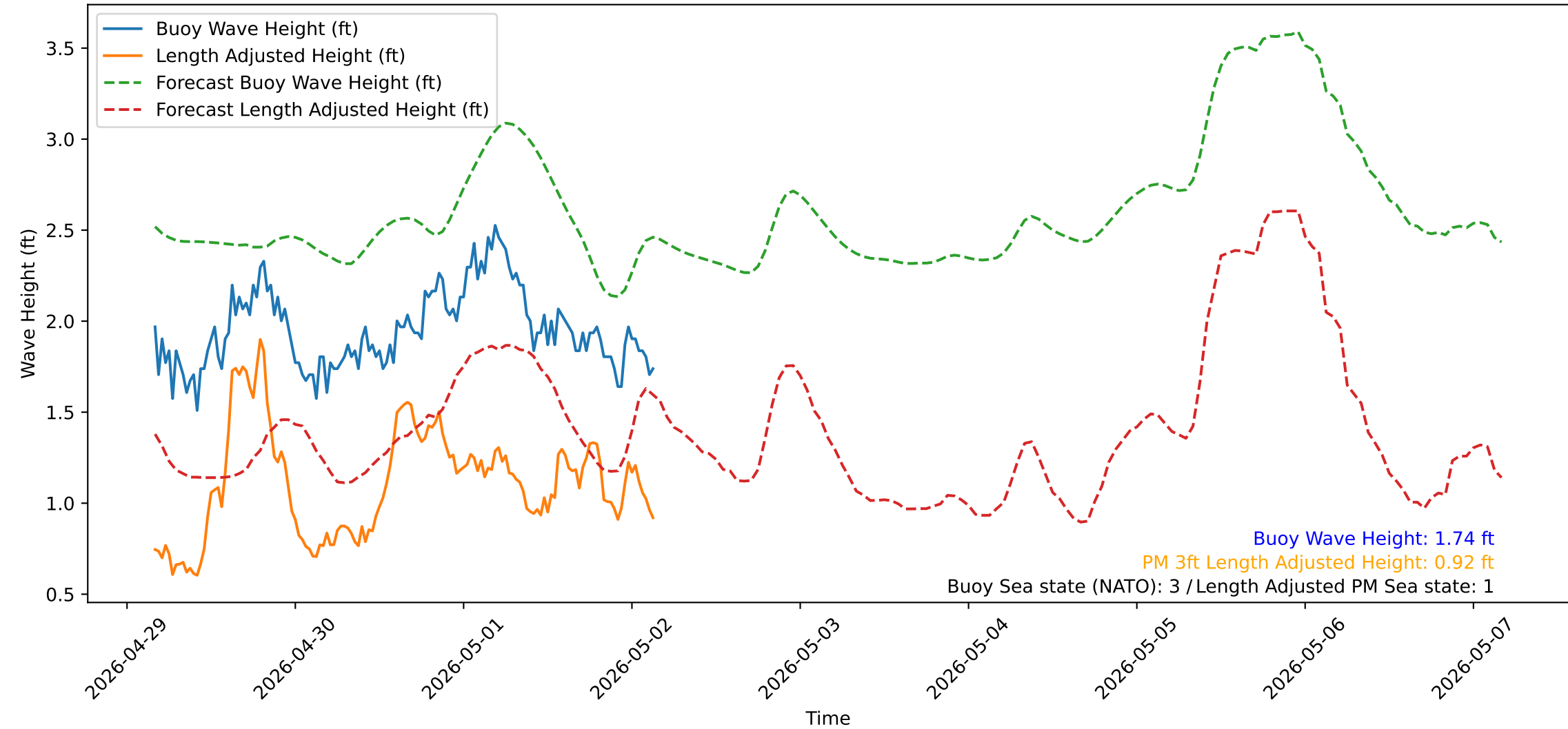
Wave Heights over Time for Red Beach at 2026-05-02 03:40:51
