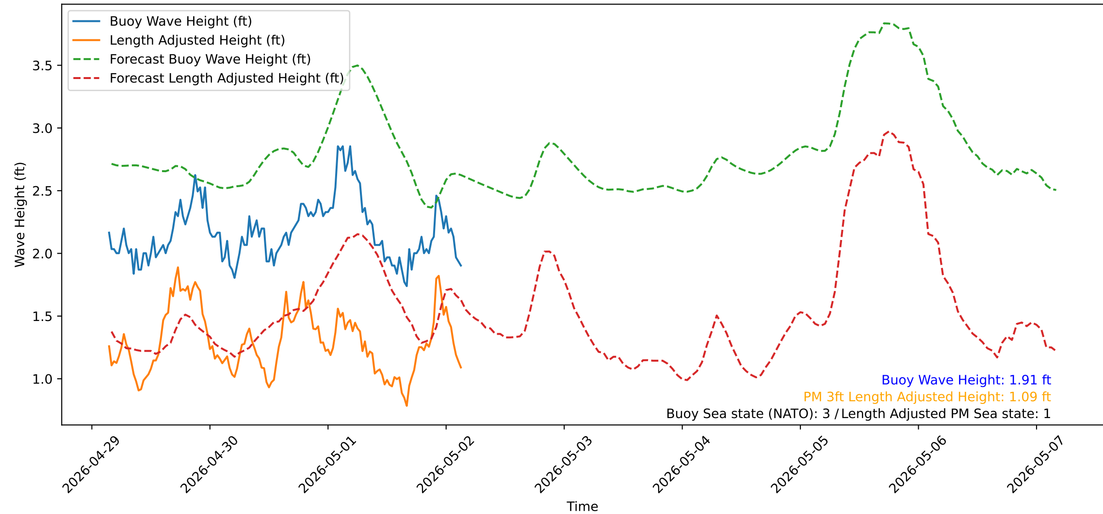
Wave Heights over Time for Green Beach at 2026-05-02 03:41:14
