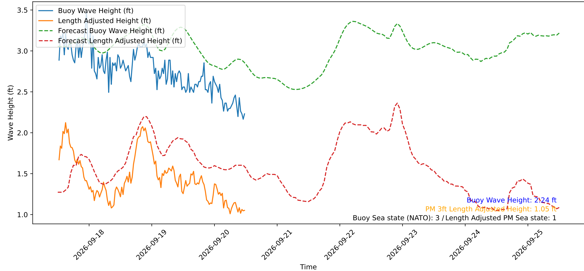
Wave Heights over Time for Green Beach at 2026-09-20 12:11:11
