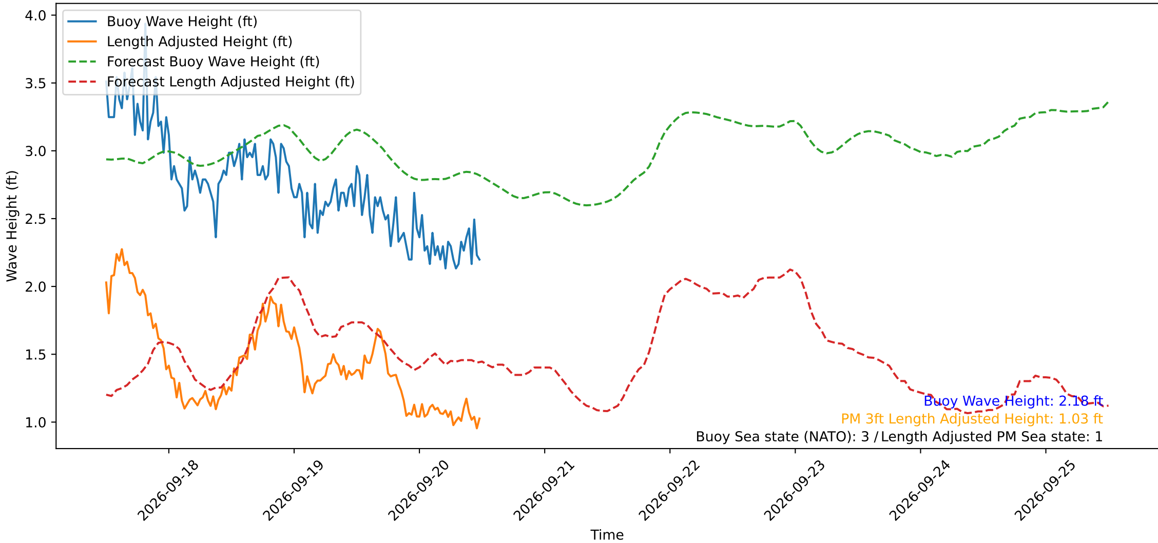
Wave Heights over Time for Oceanside Harbor at 2026-09-20 12:10:30
