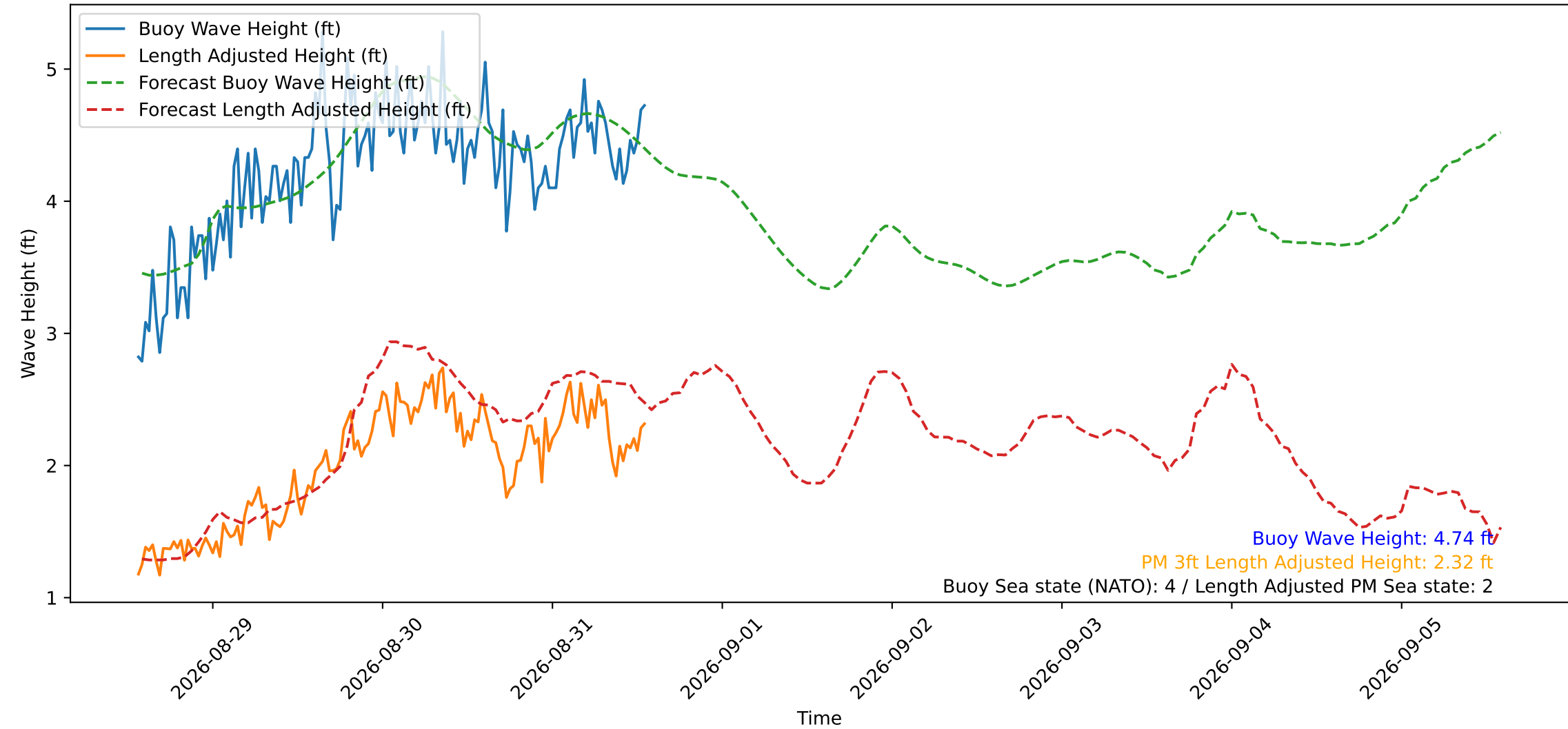
Wave Heights over Time for Oceanside Harbor at 2026-08-31 13:40:30
