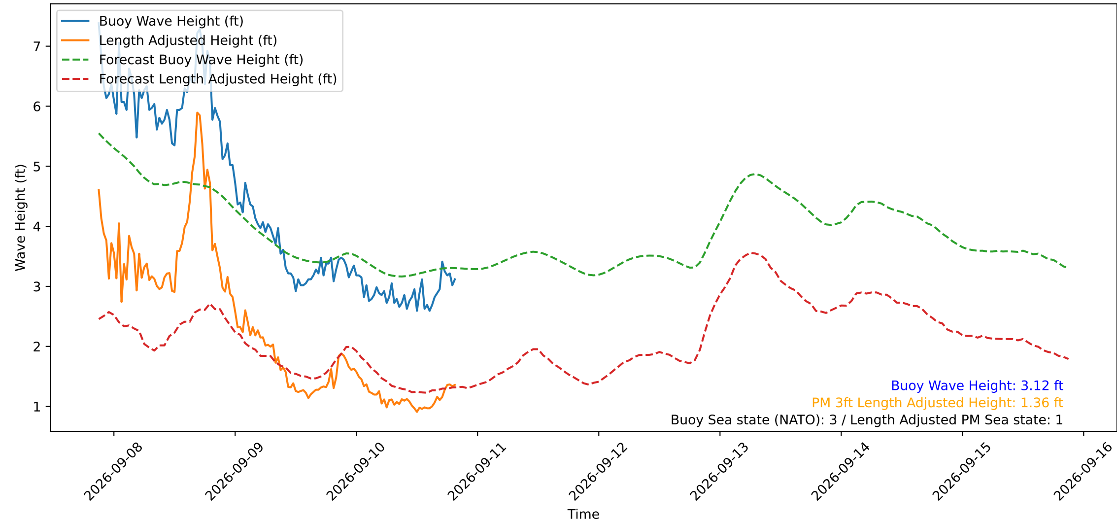
Wave Heights over Time for Green Beach at 2026-09-10 20:31:12
