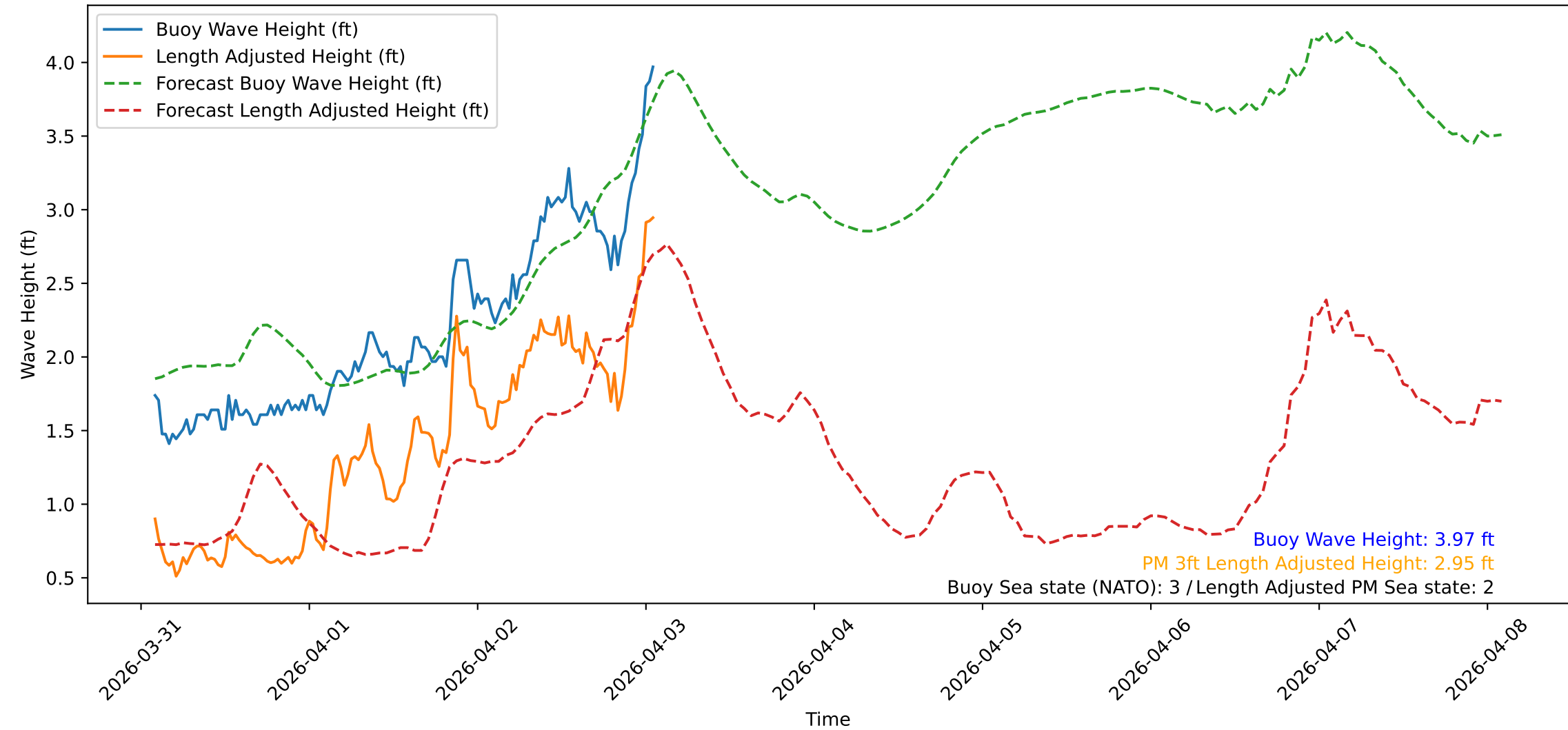
Wave Heights over Time for Green Beach at 2026-04-03 02:01:09
