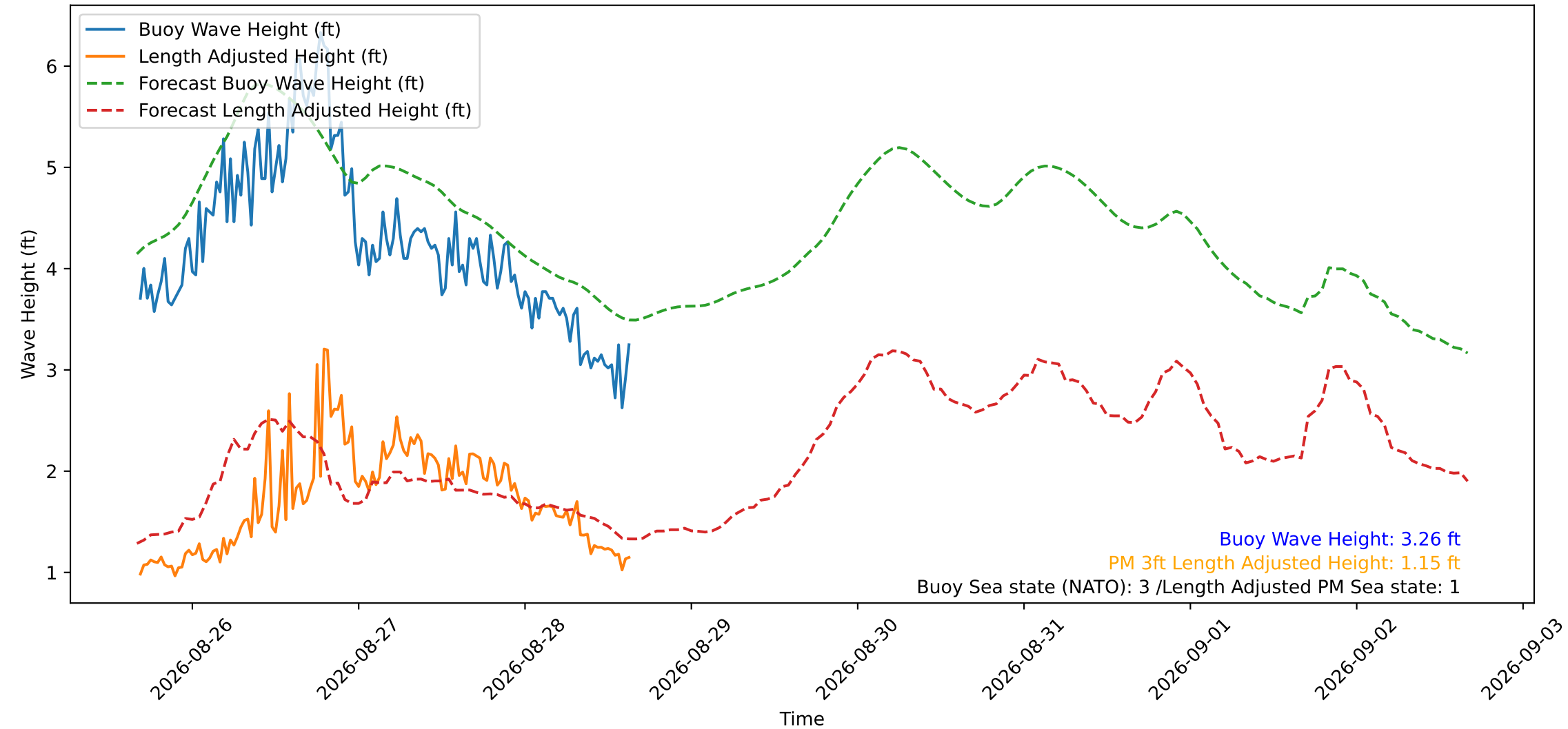
Wave Heights over Time for Green Beach at 2026-08-28 16:01:12
