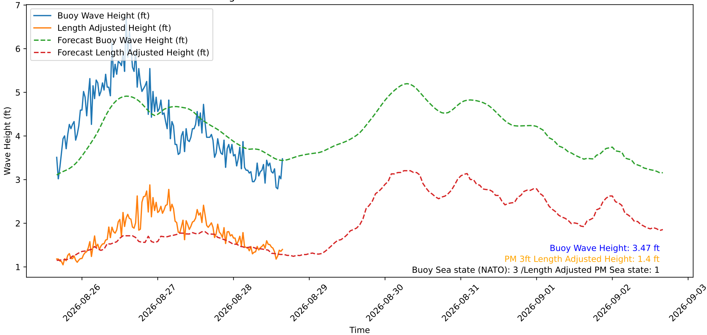
Wave Heights over Time for Oceanside Harbor at 2026-08-28 16:00:29
