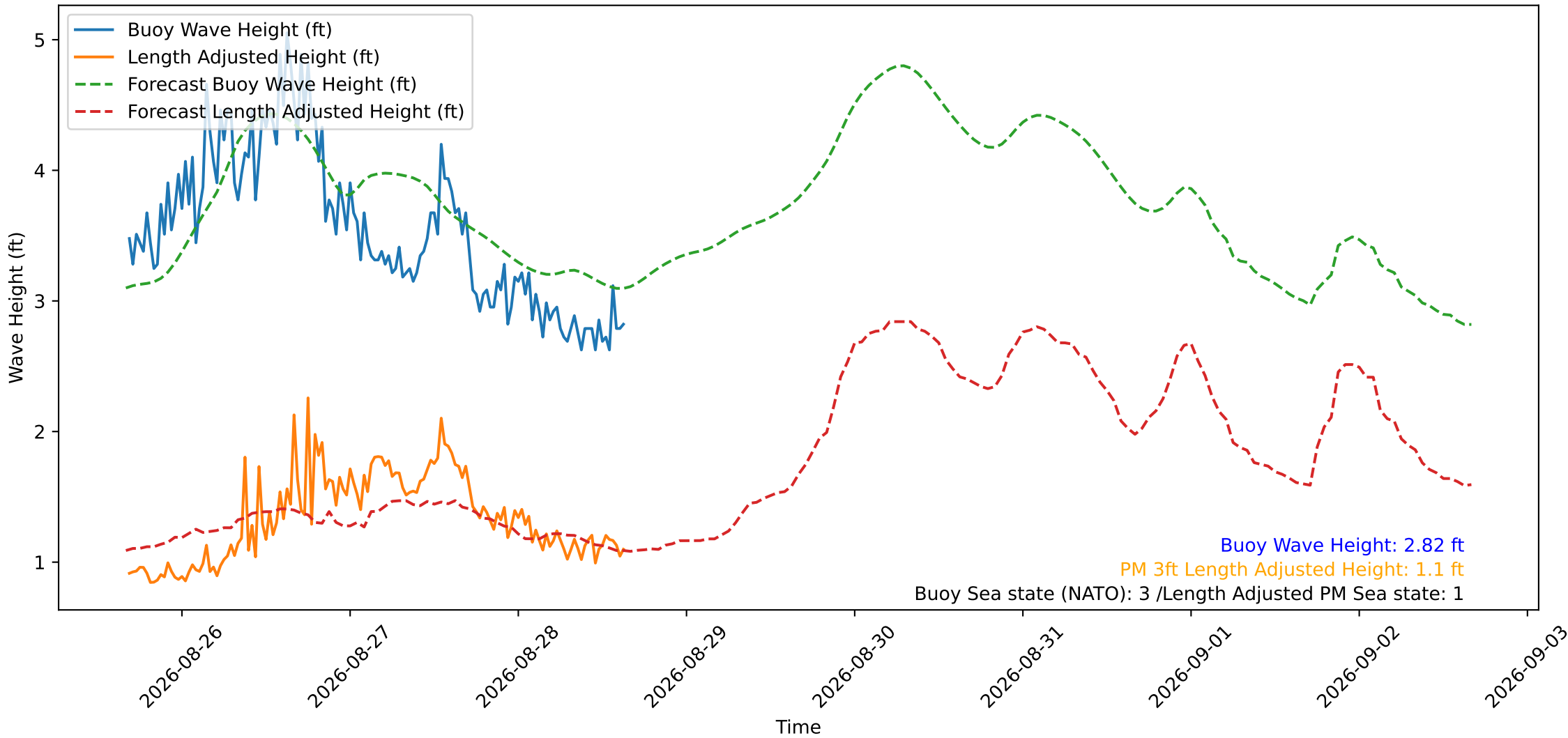
Wave Heights over Time for Red Beach at 2026-08-28 16:00:49
