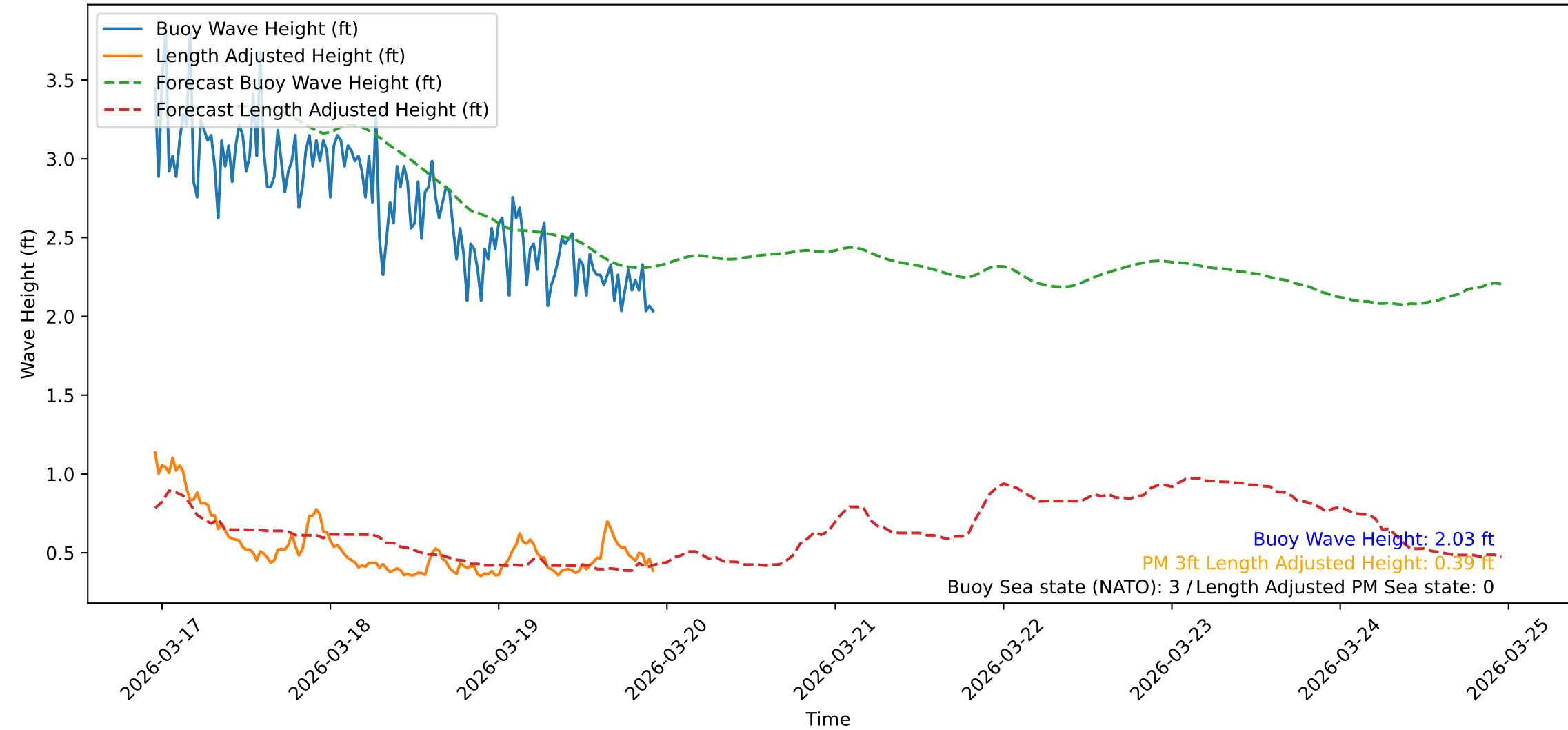
Wave Heights over Time for Red Beach at 2026-03-19 22:50:49
