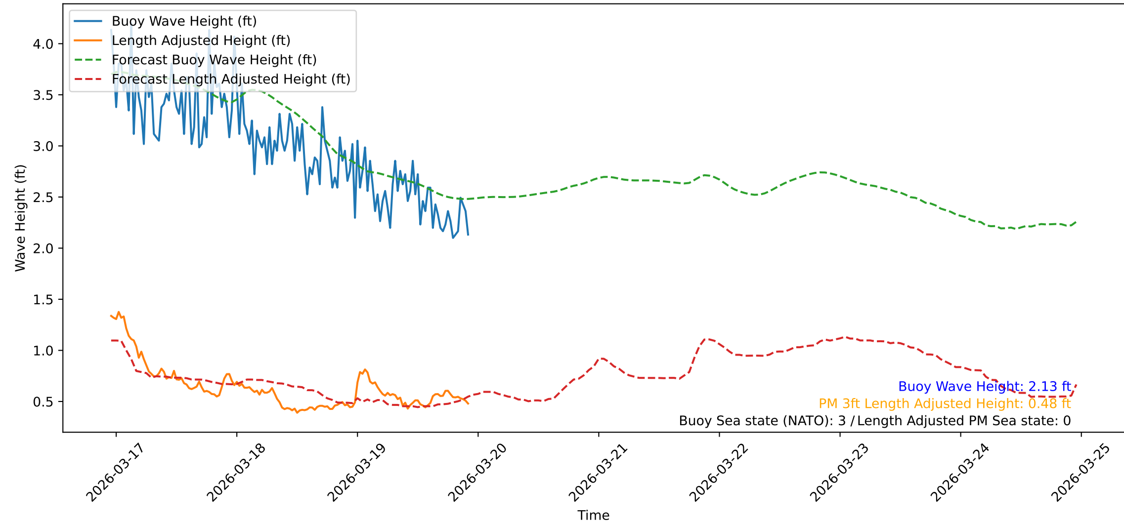
Wave Heights over Time for Green Beach at 2026-03-19 22:51:11
