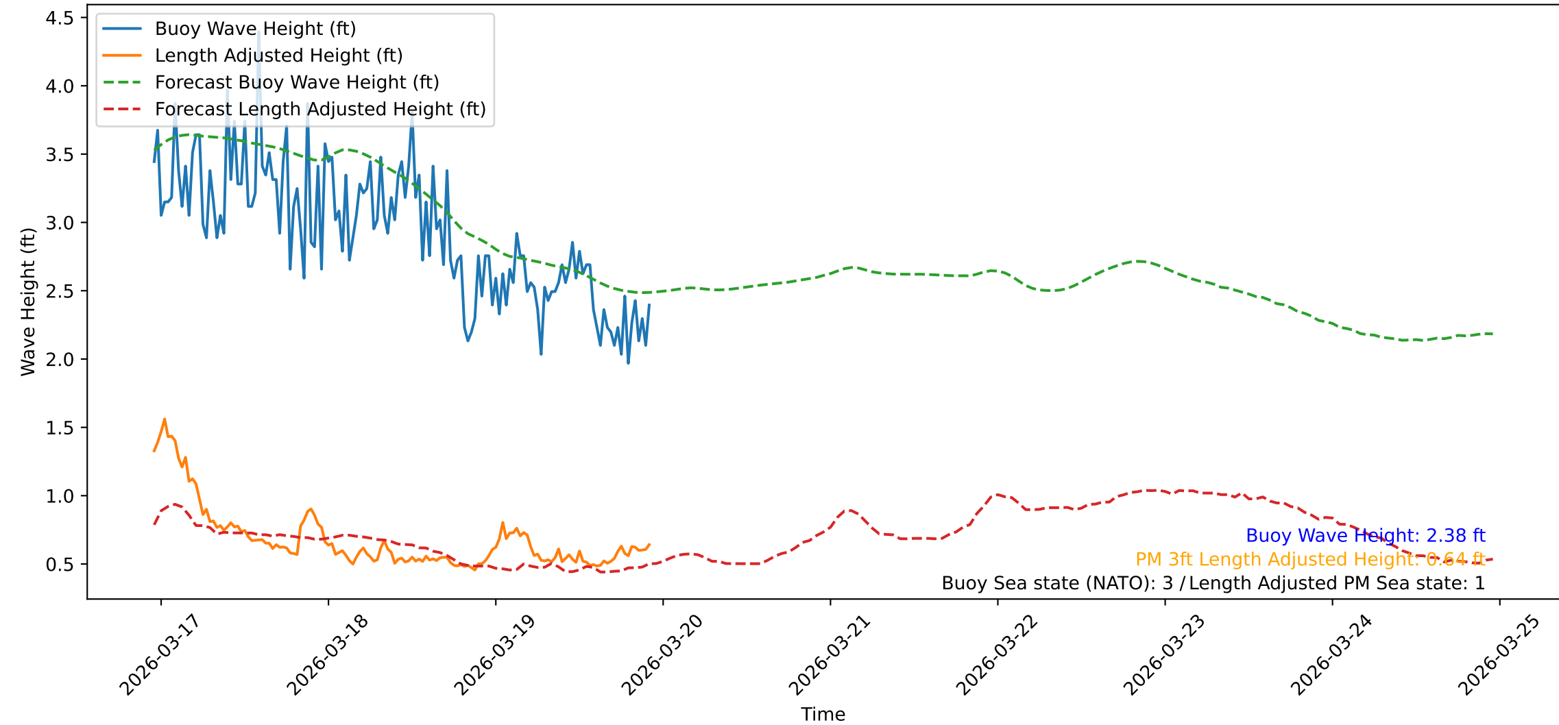
Wave Heights over Time for Oceanside Harbor at 2026-03-19 22:50:32
