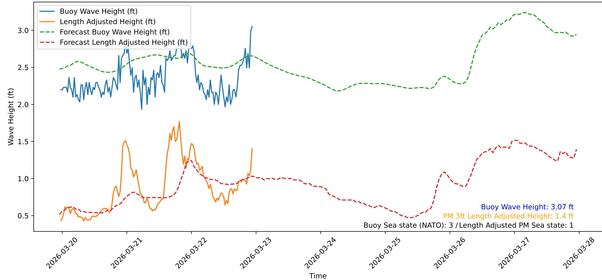
Wave Heights over Time for Green Beach at 2026-03-22 23:21:10
