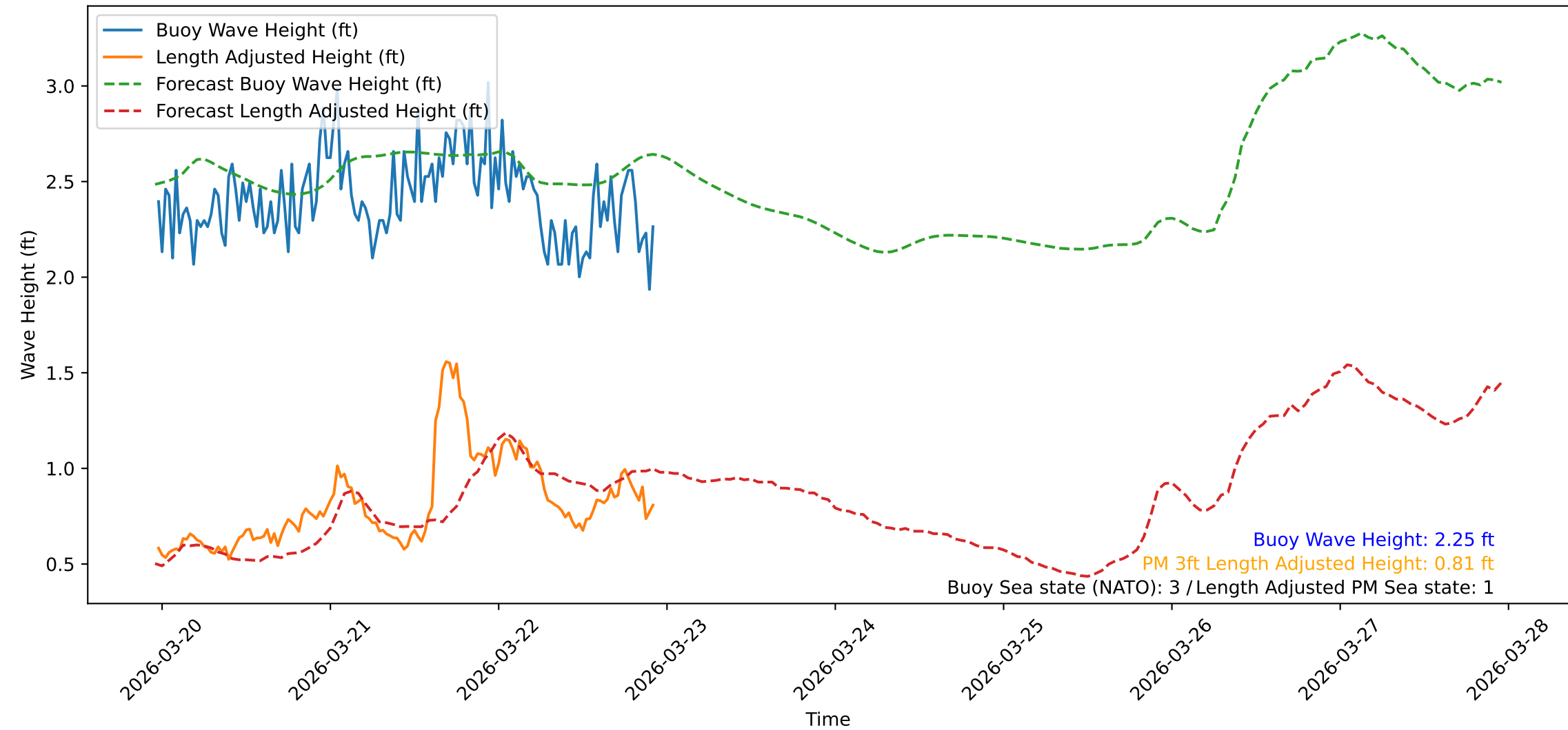
Wave Heights over Time for Oceanside Harbor at 2026-03-22 23:20:31
