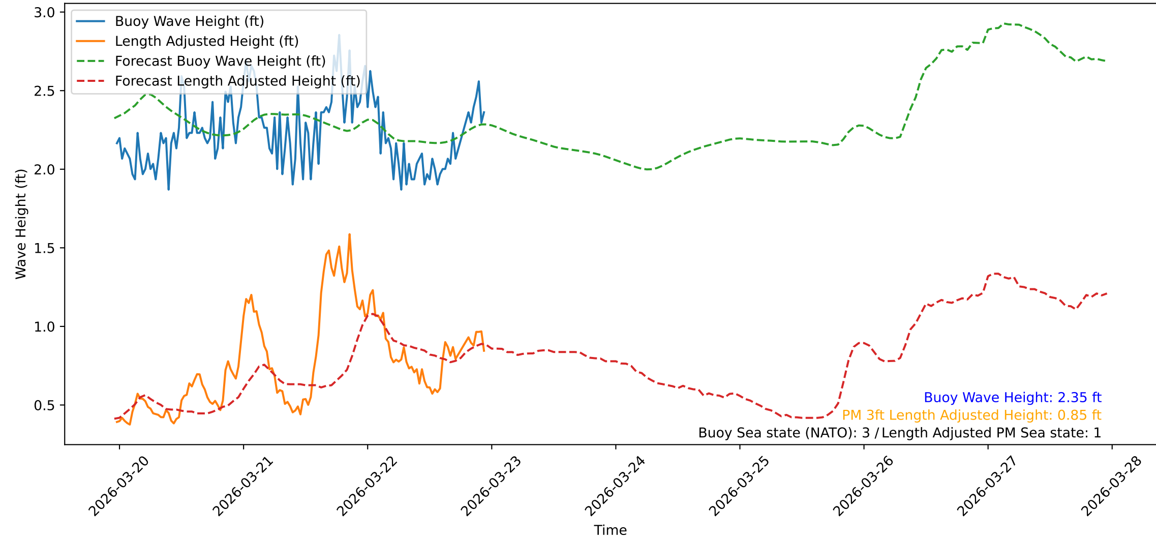
Wave Heights over Time for Red Beach at 2026-03-22 23:20:47
