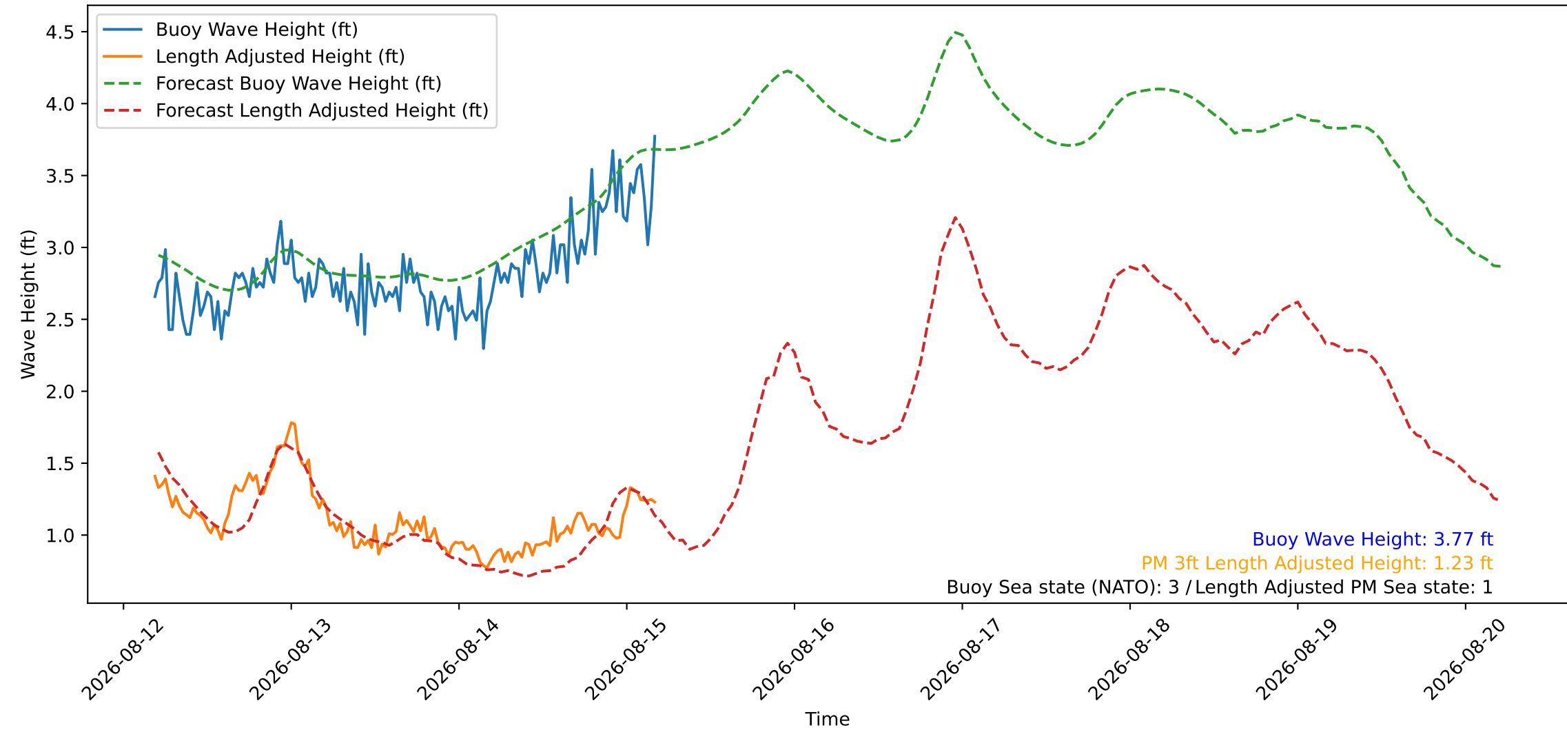
Wave Heights over Time for Oceanside Harbor at 2026-08-15 04:40:27
