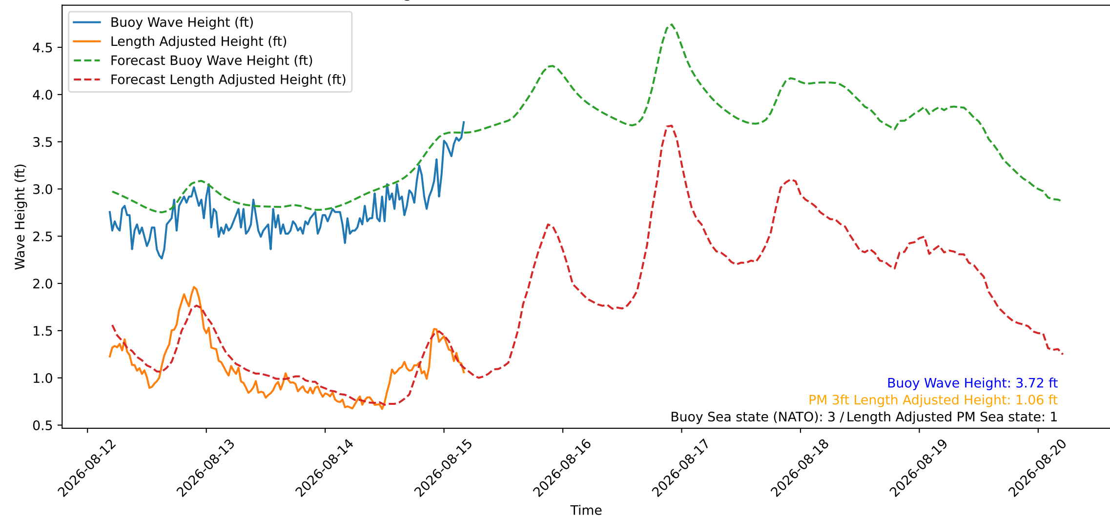
Wave Heights over Time for Green Beach at 2026-08-15 04:41:09
