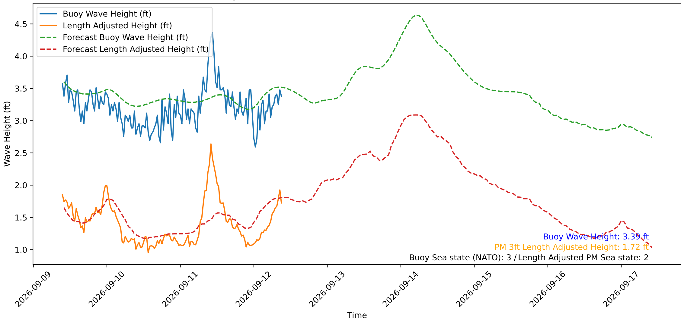
Wave Heights over Time for Oceanside Harbor at 2026-09-12 09:40:30
