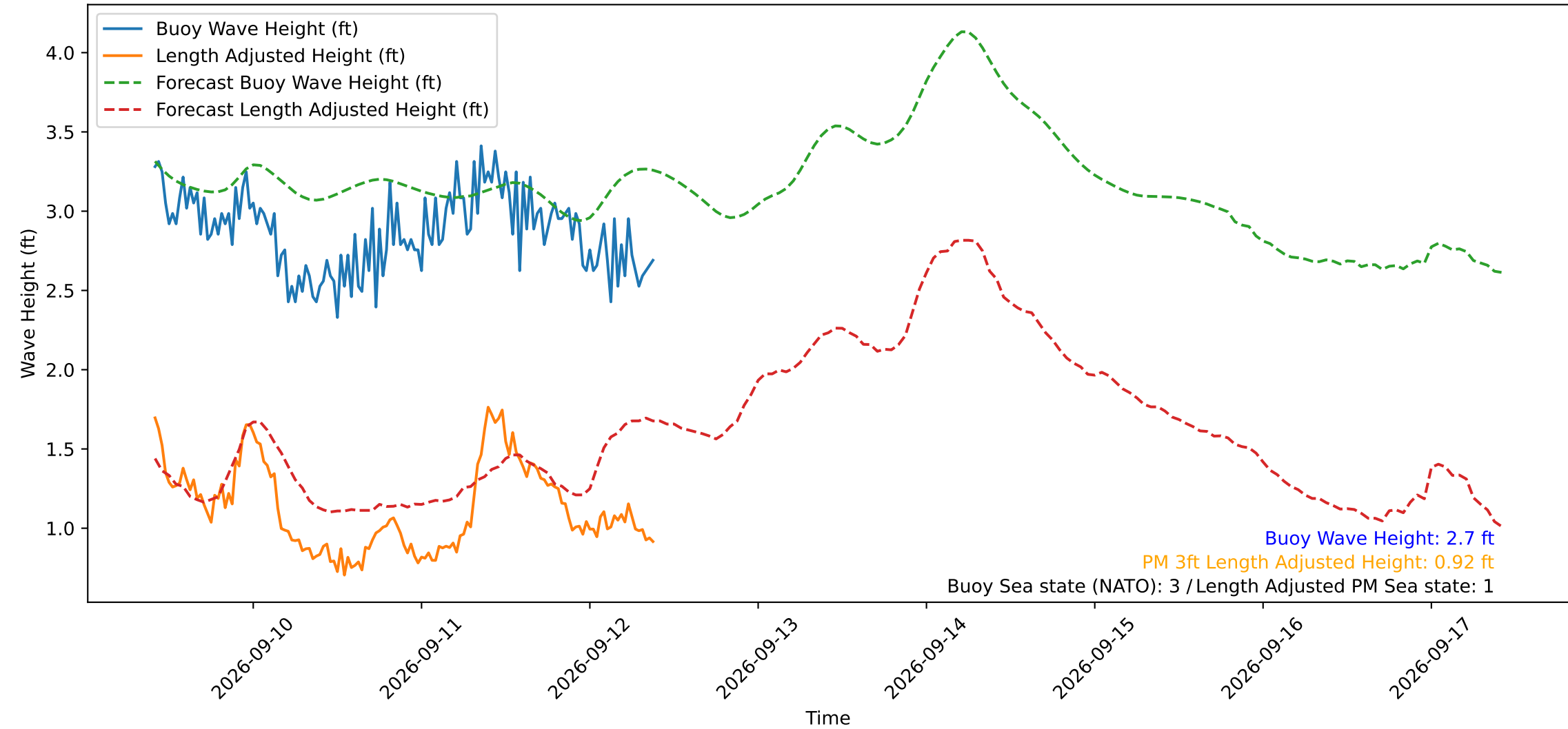
Wave Heights over Time for Red Beach at 2026-09-12 09:40:50
