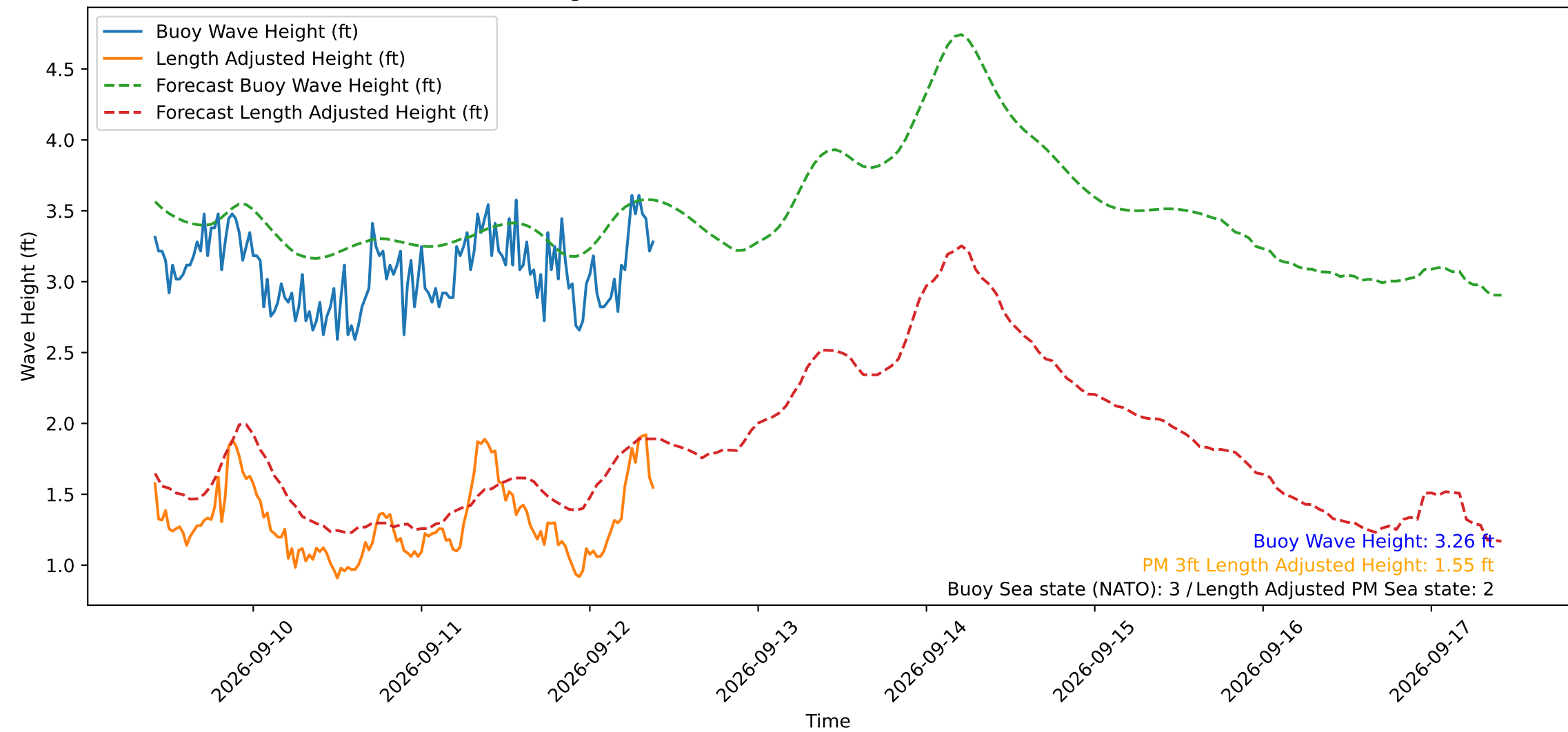
Wave Heights over Time for Green Beach at 2026-09-12 09:41:13
