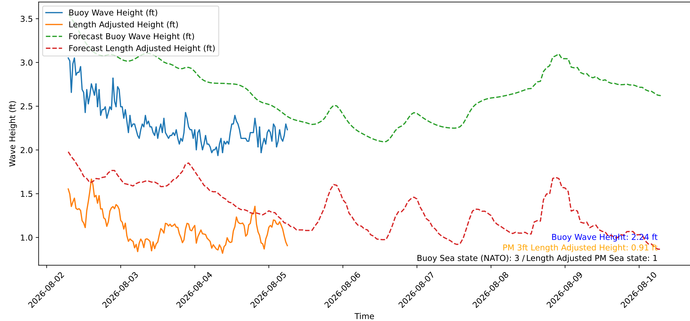
Wave Heights over Time for Green Beach at 2026-08-05 06:51:09
