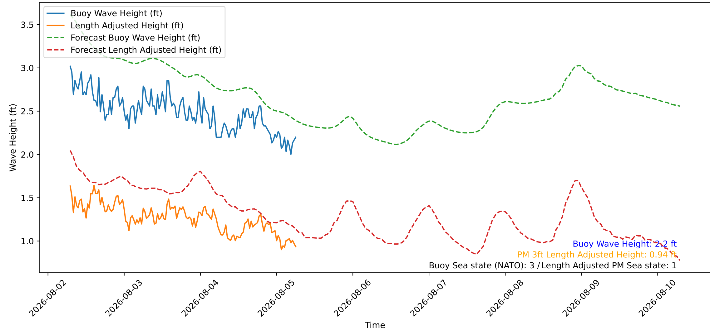
Wave Heights over Time for Oceanside Harbor at 2026-08-05 06:50:26
