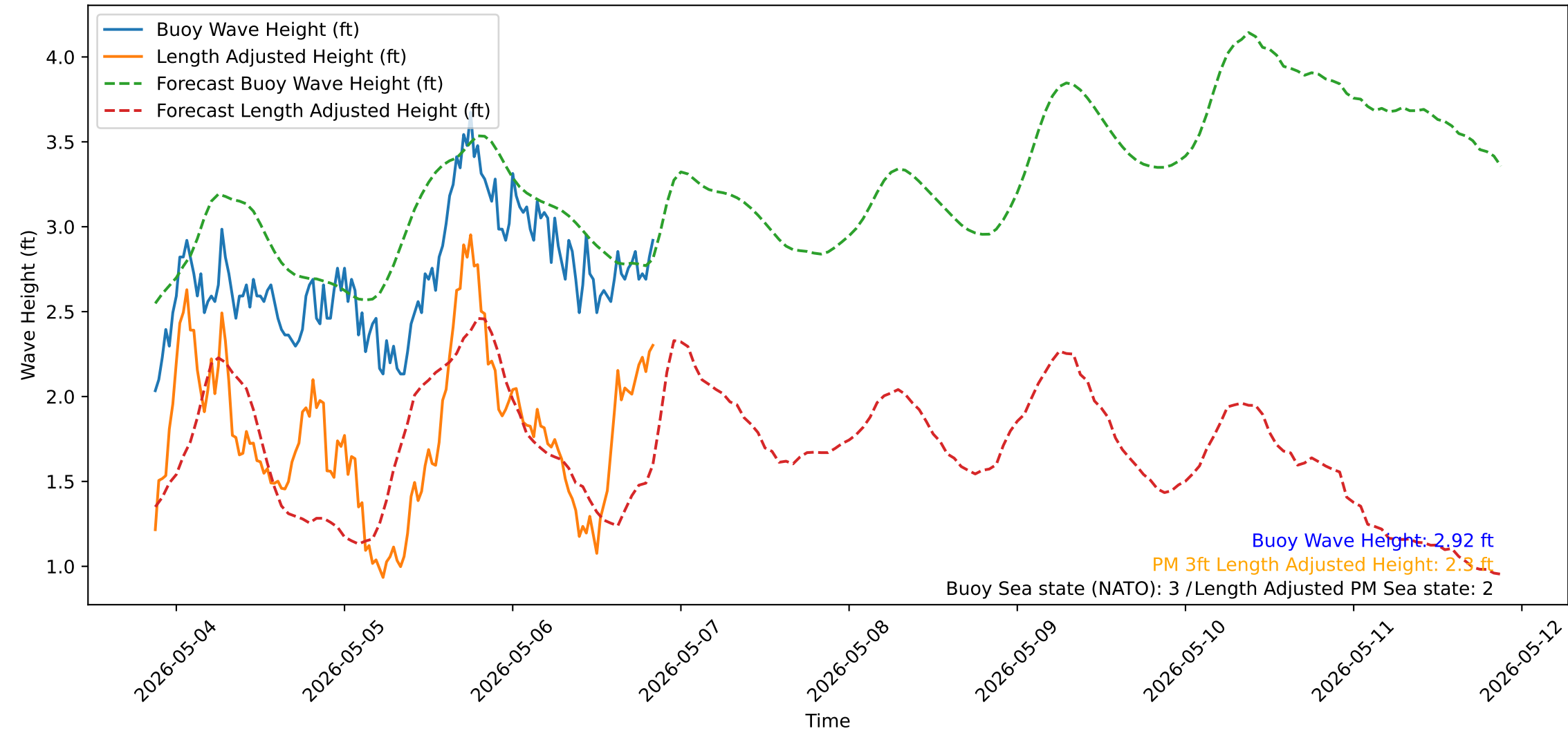
Wave Heights over Time for Green Beach at 2026-05-06 20:51:15
