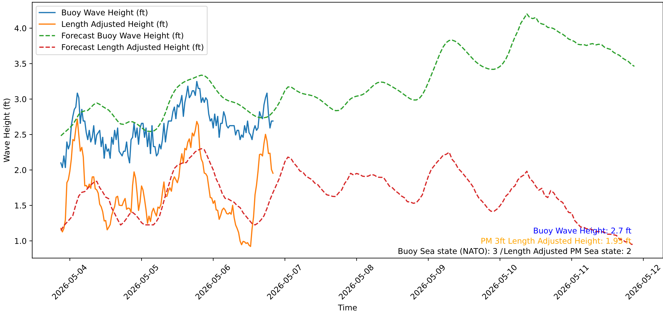
Wave Heights over Time for Oceanside Harbor at 2026-05-06 20:50:31
