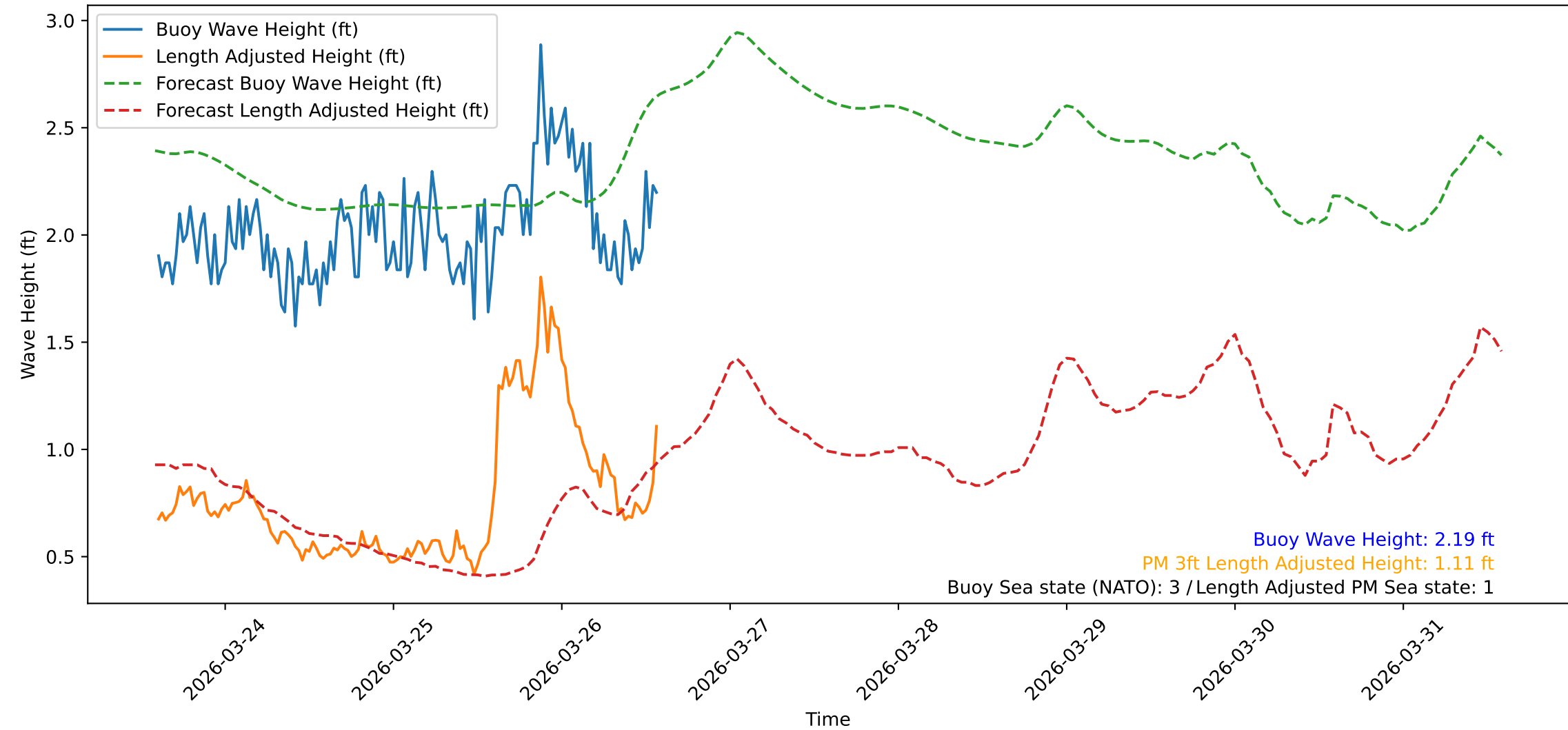
Wave Heights over Time for Oceanside Harbor at 2026-03-26 14:20:31
