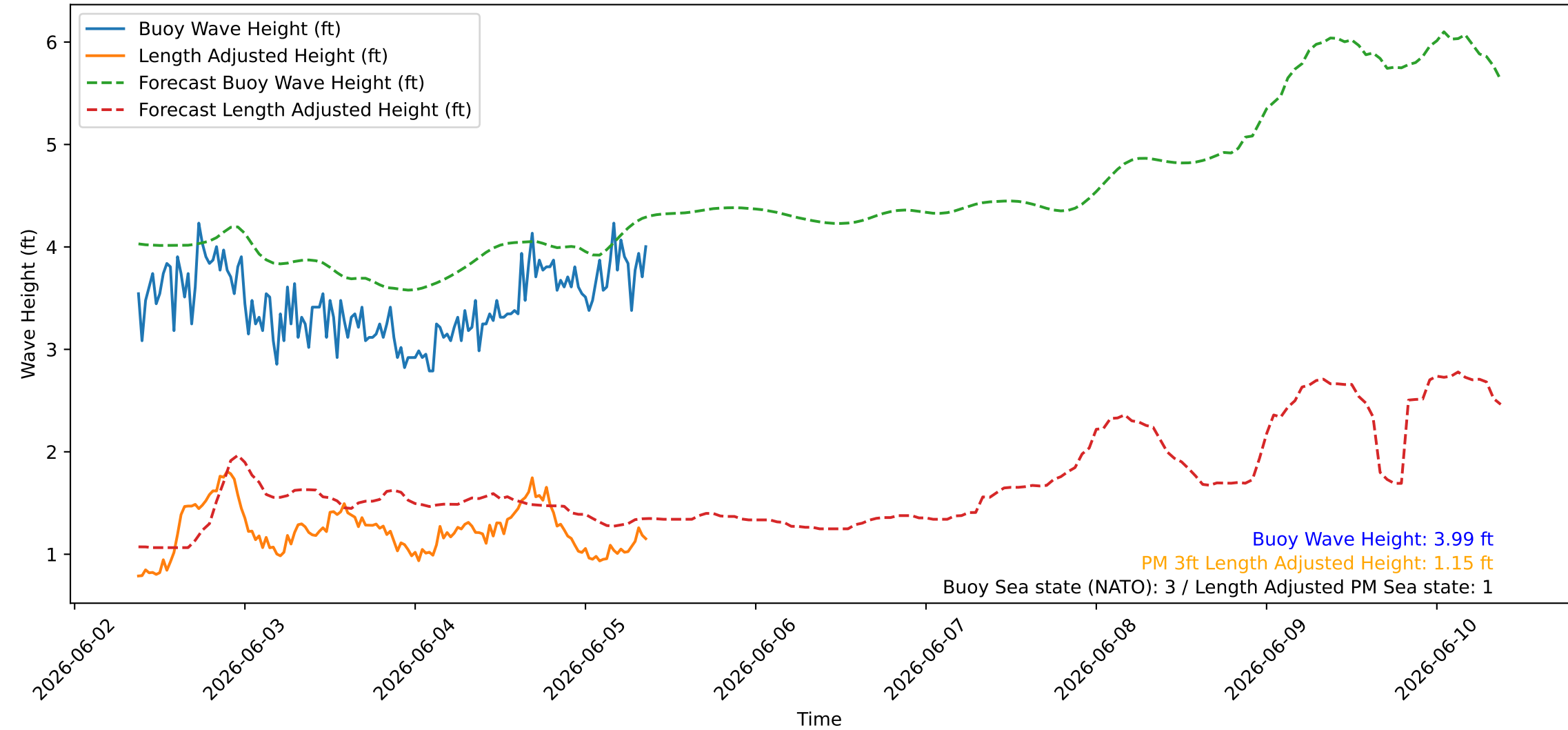
Wave Heights over Time for Green Beach at 2026-06-05 09:11:06
