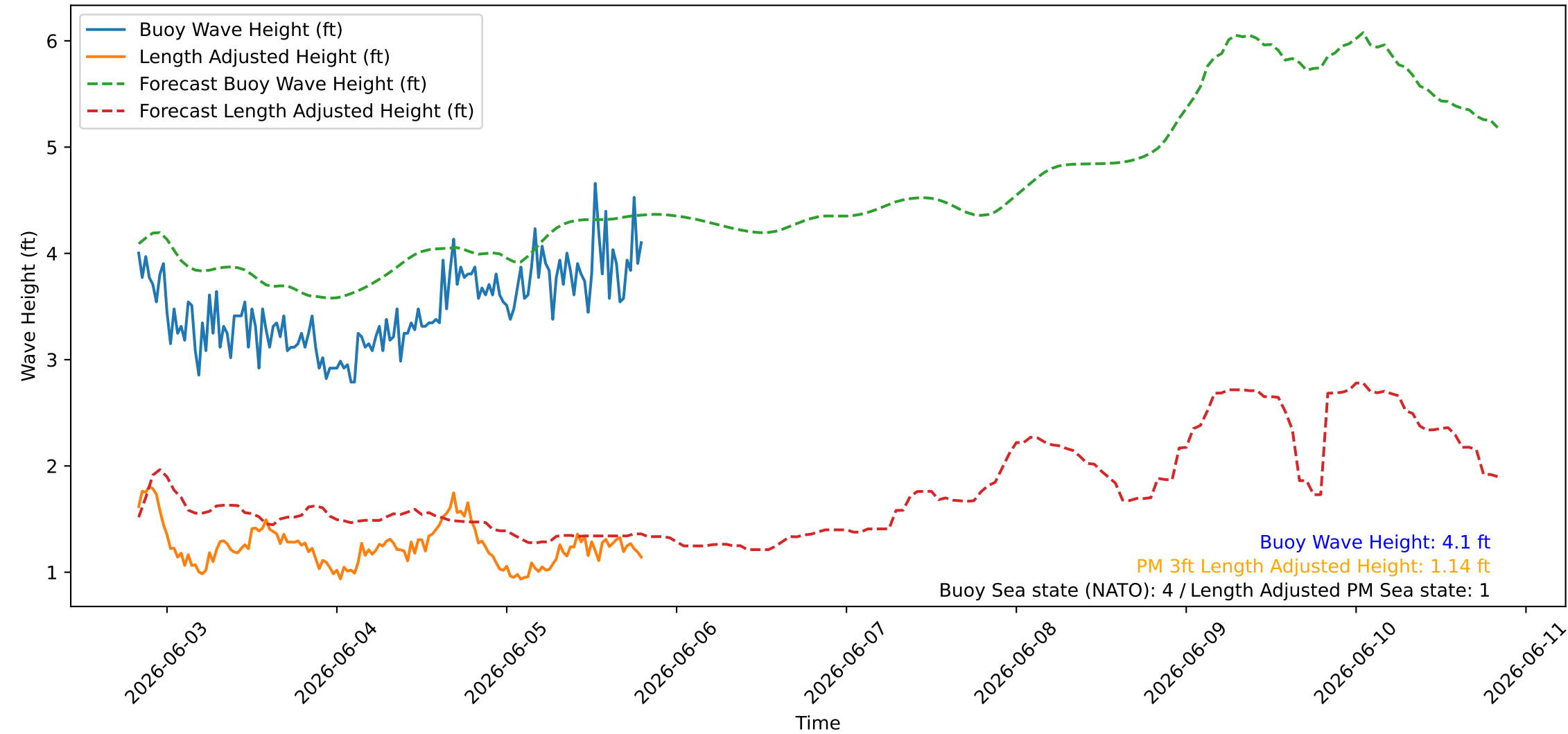
Wave Heights over Time for Green Beach at 2026-06-05 20:01:08
