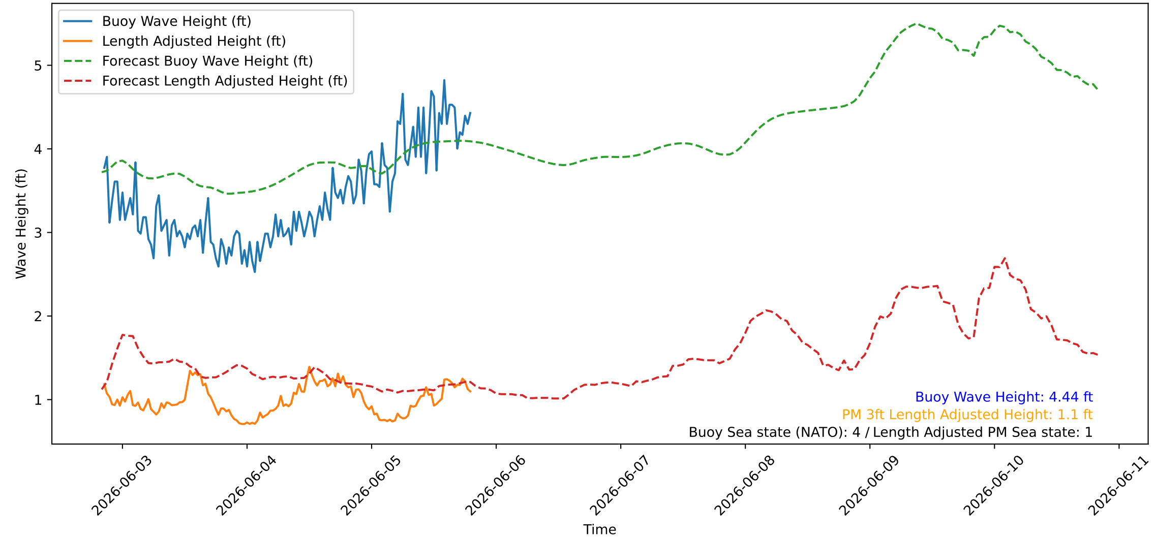
Wave Heights over Time for Red Beach at 2026-06-05 20:00:45
