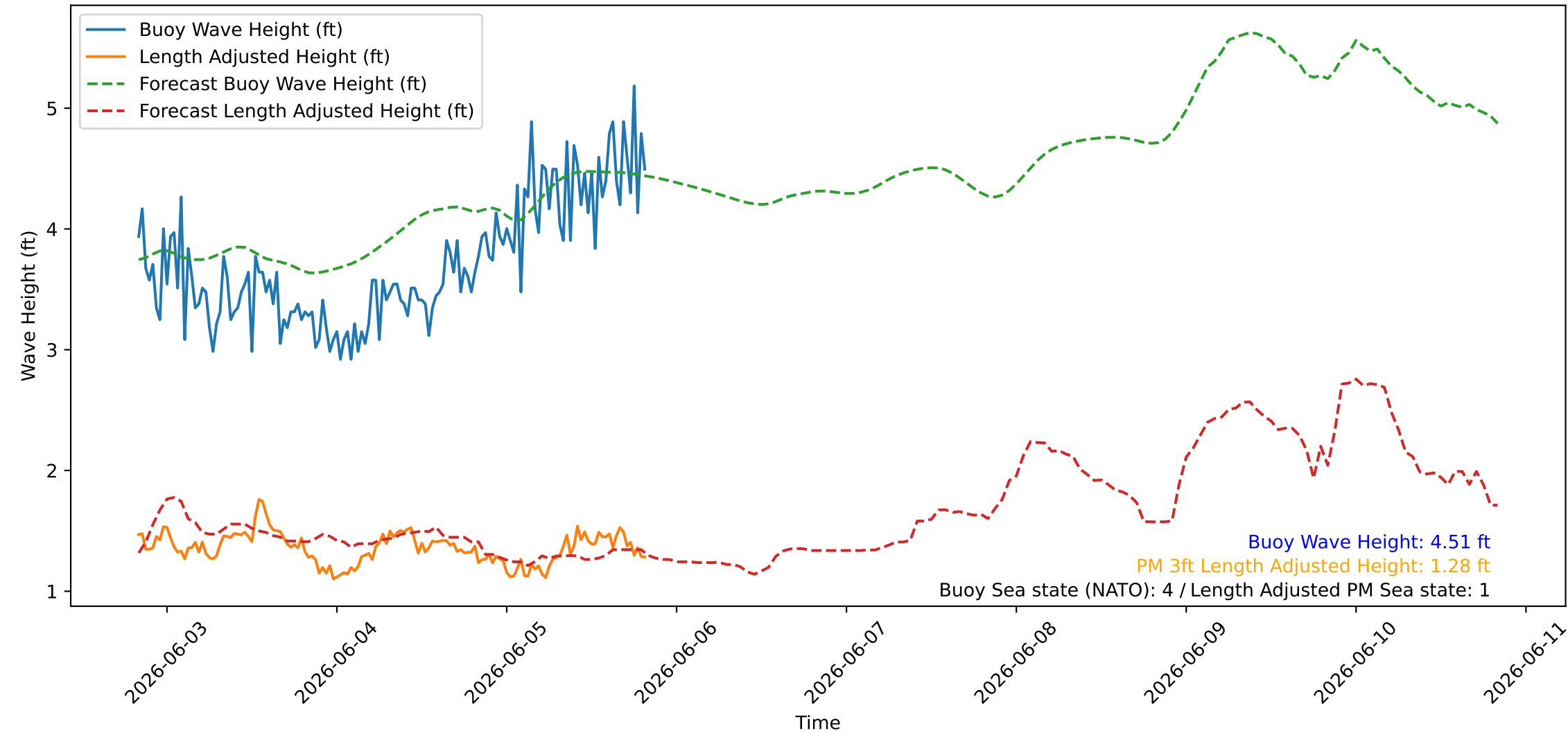
Wave Heights over Time for Oceanside Harbor at 2026-06-05 20:00:26
