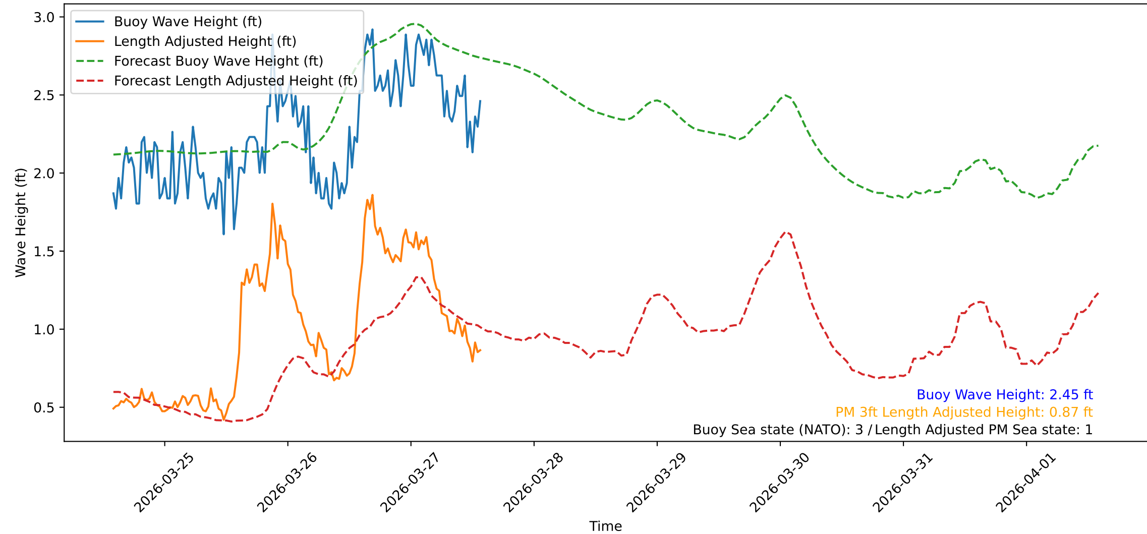
Wave Heights over Time for Oceanside Harbor at 2026-03-27 14:10:31
