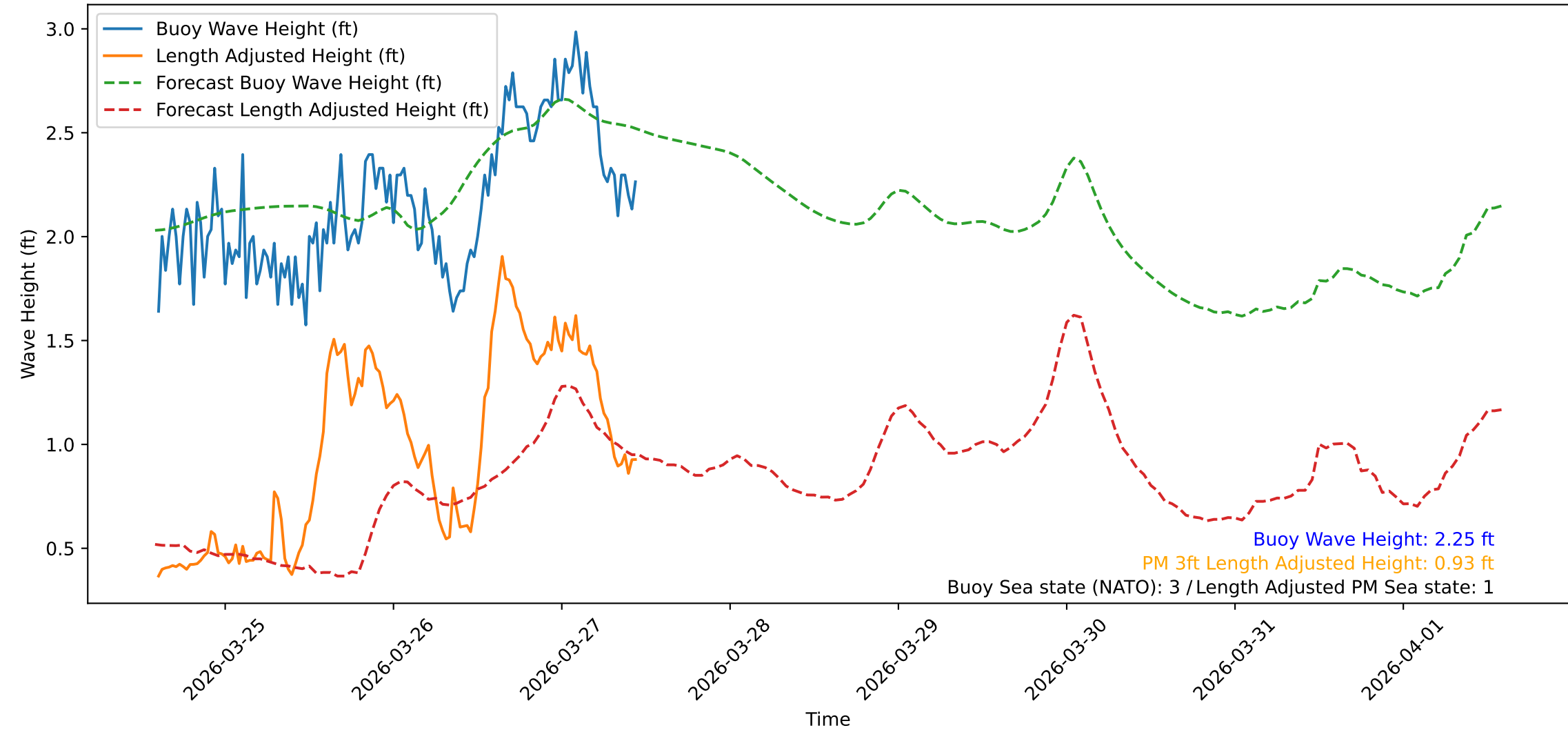
Wave Heights over Time for Red Beach at 2026-03-27 14:10:47
