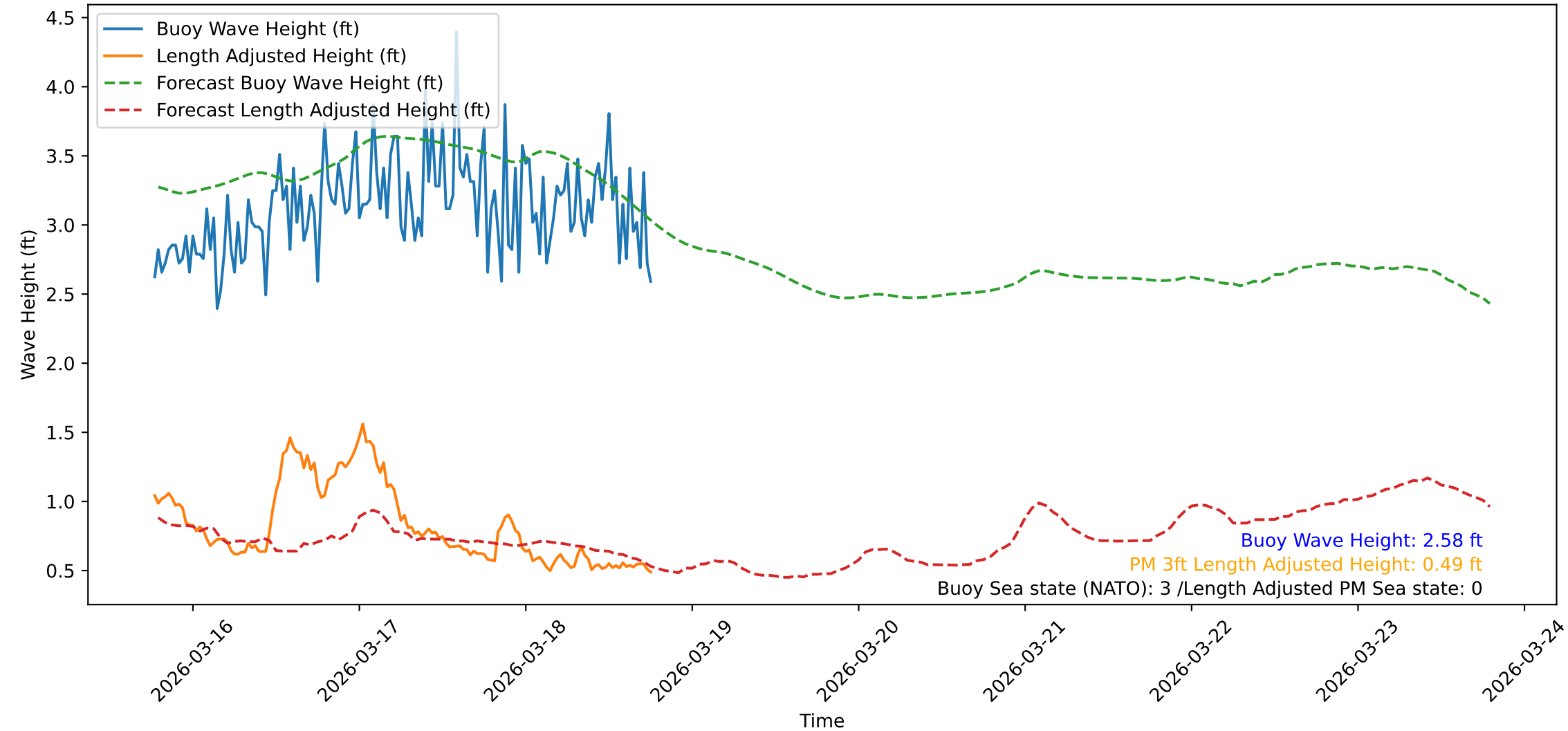
Wave Heights over Time for Oceanside Harbor at 2026-03-18 18:40:32
