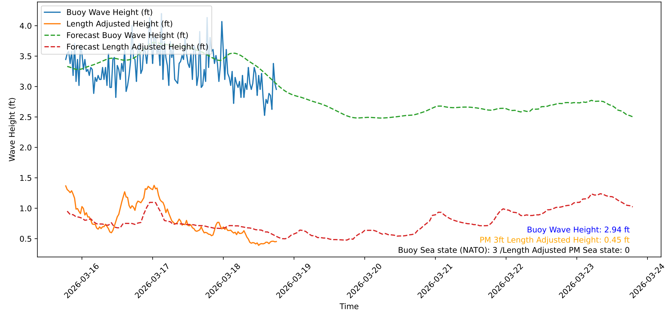
Wave Heights over Time for Green Beach at 2026-03-18 18:41:11
