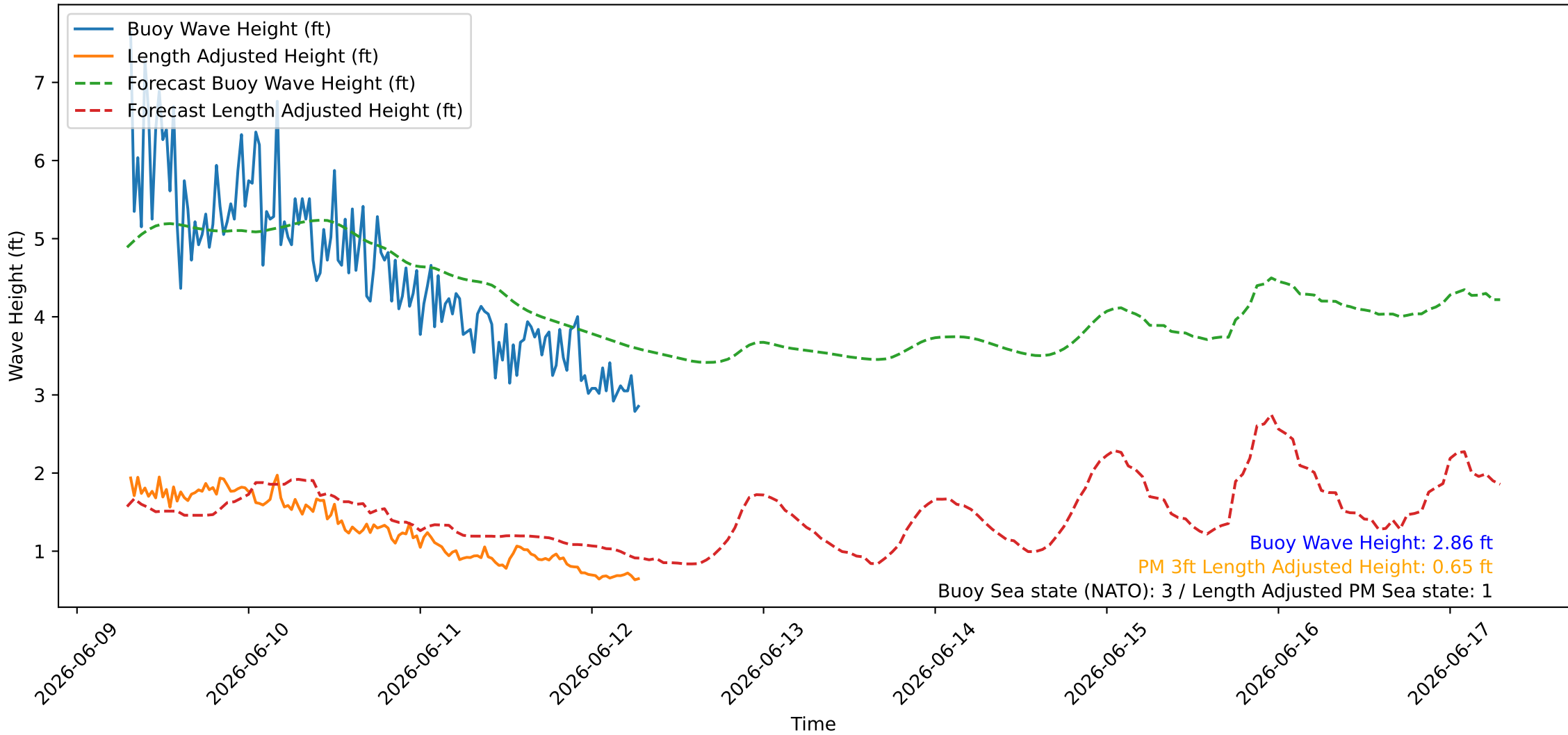
Wave Heights over Time for Red Beach at 2026-06-12 07:10:46
