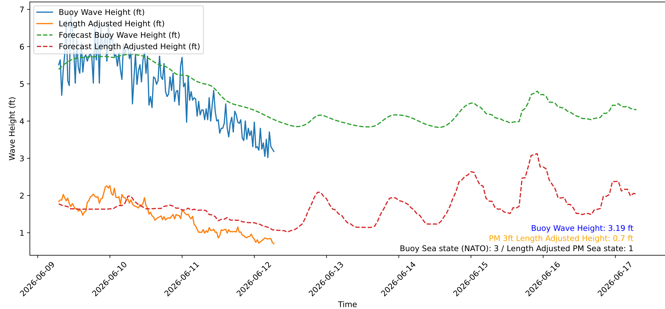
Wave Heights over Time for Green Beach at 2026-06-12 07:11:08
