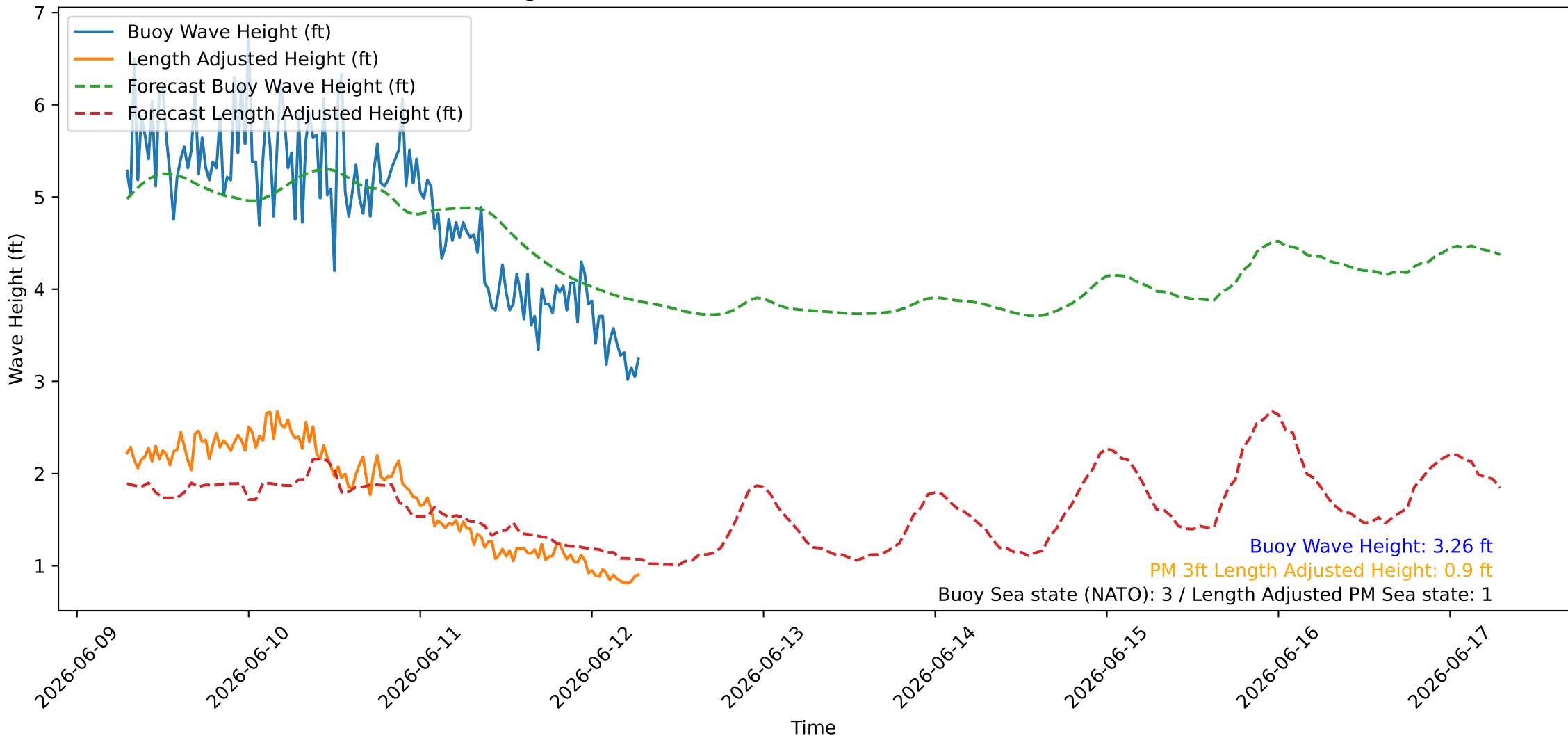
Wave Heights over Time for Oceanside Harbor at 2026-06-12 07:10:26
