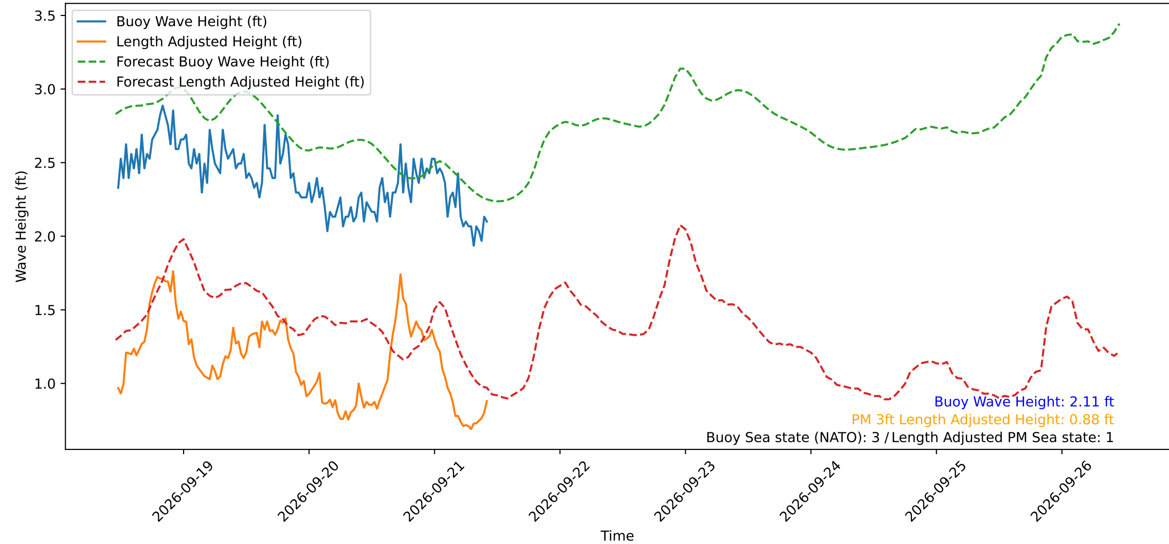
Wave Heights over Time for Red Beach at 2026-09-21 11:10:55
