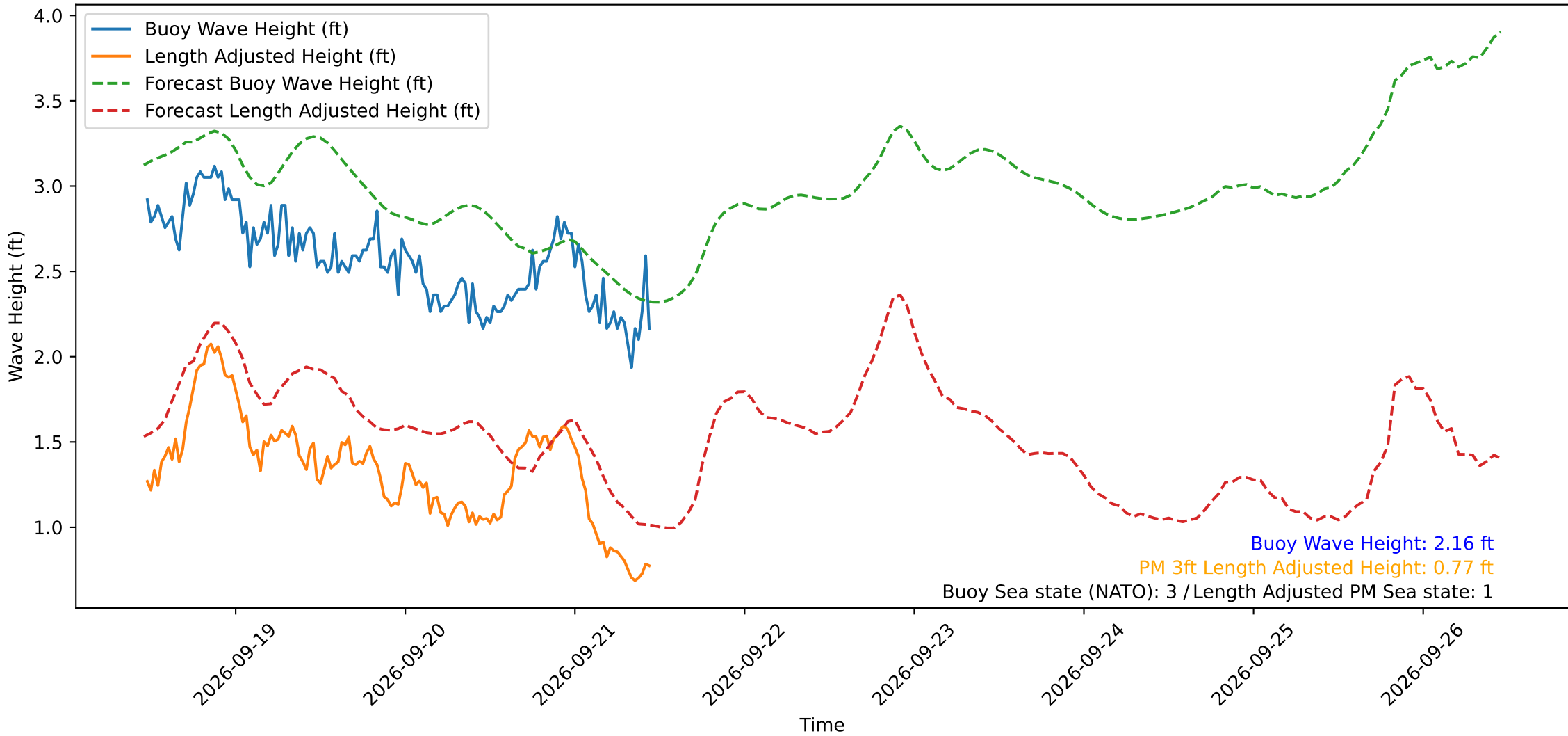
Wave Heights over Time for Green Beach at 2026-09-21 11:11:21
