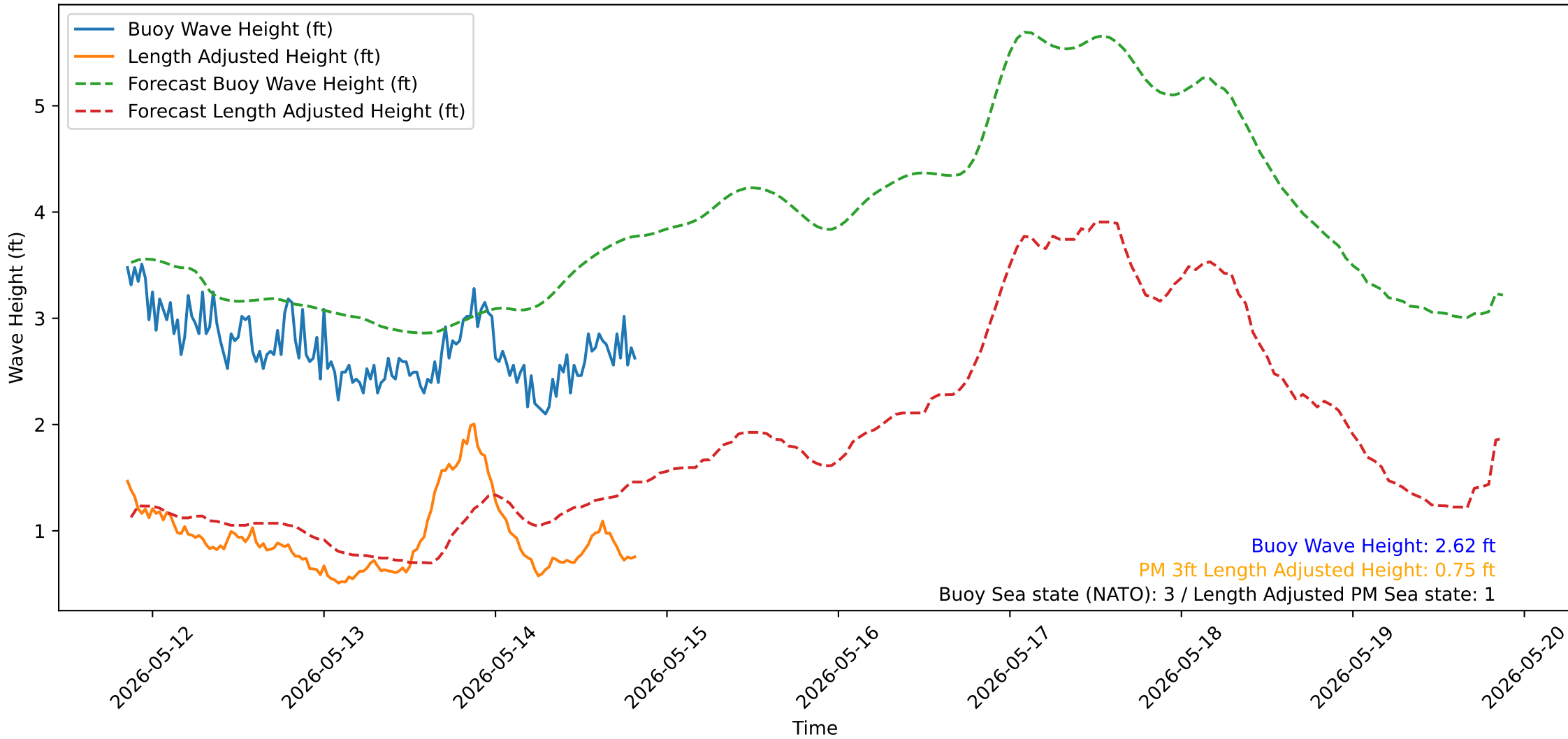
Wave Heights over Time for Green Beach at 2026-05-14 20:31:16
