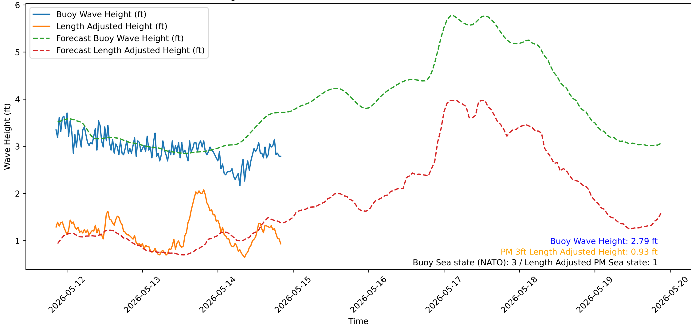
Wave Heights over Time for Oceanside Harbor at 2026-05-14 20:30:33
