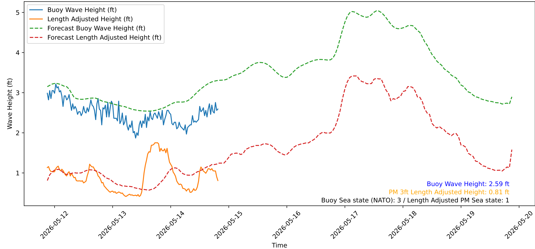
Wave Heights over Time for Red Beach at 2026-05-14 20:30:53
