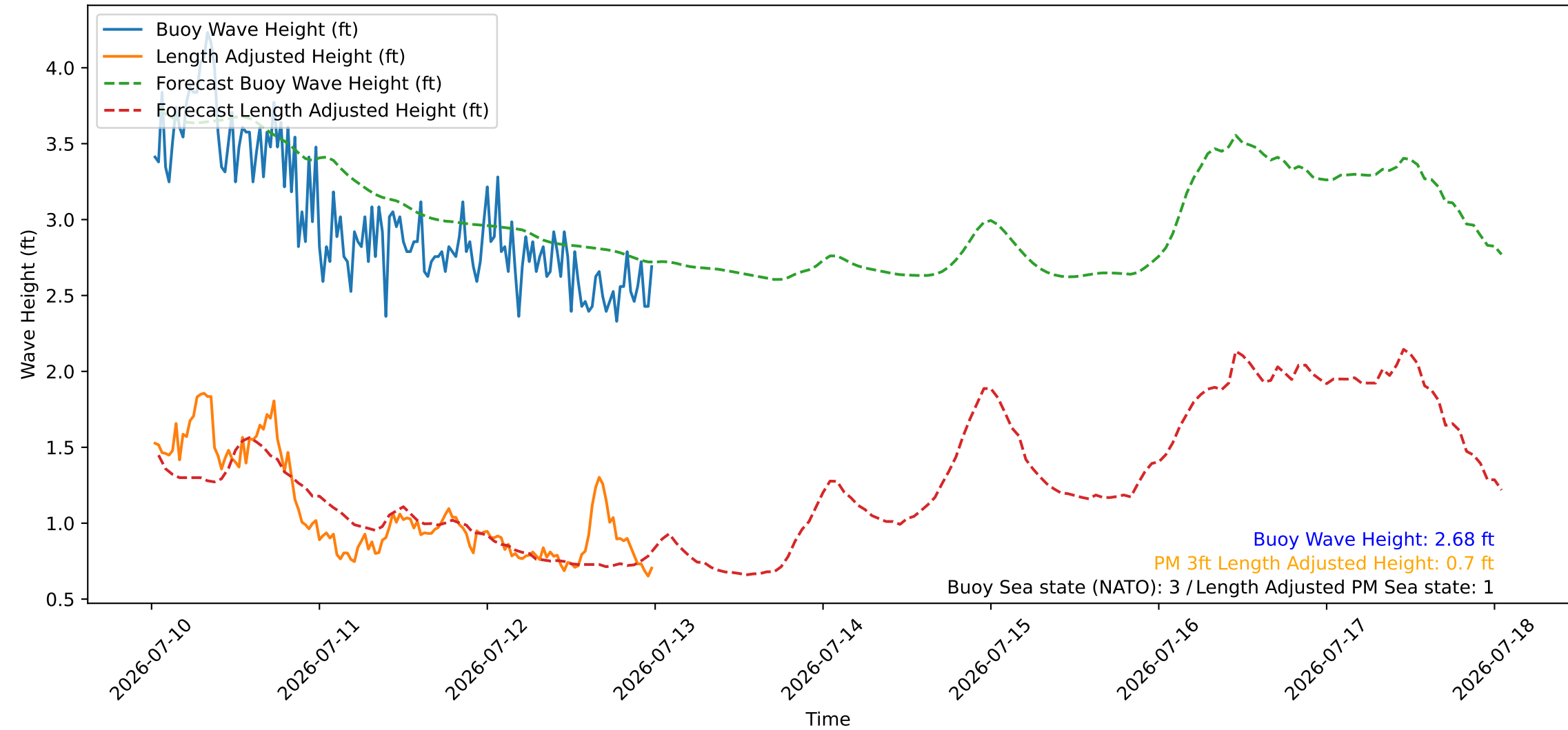
Wave Heights over Time for Oceanside Harbor at 2026-07-13 00:30:26
