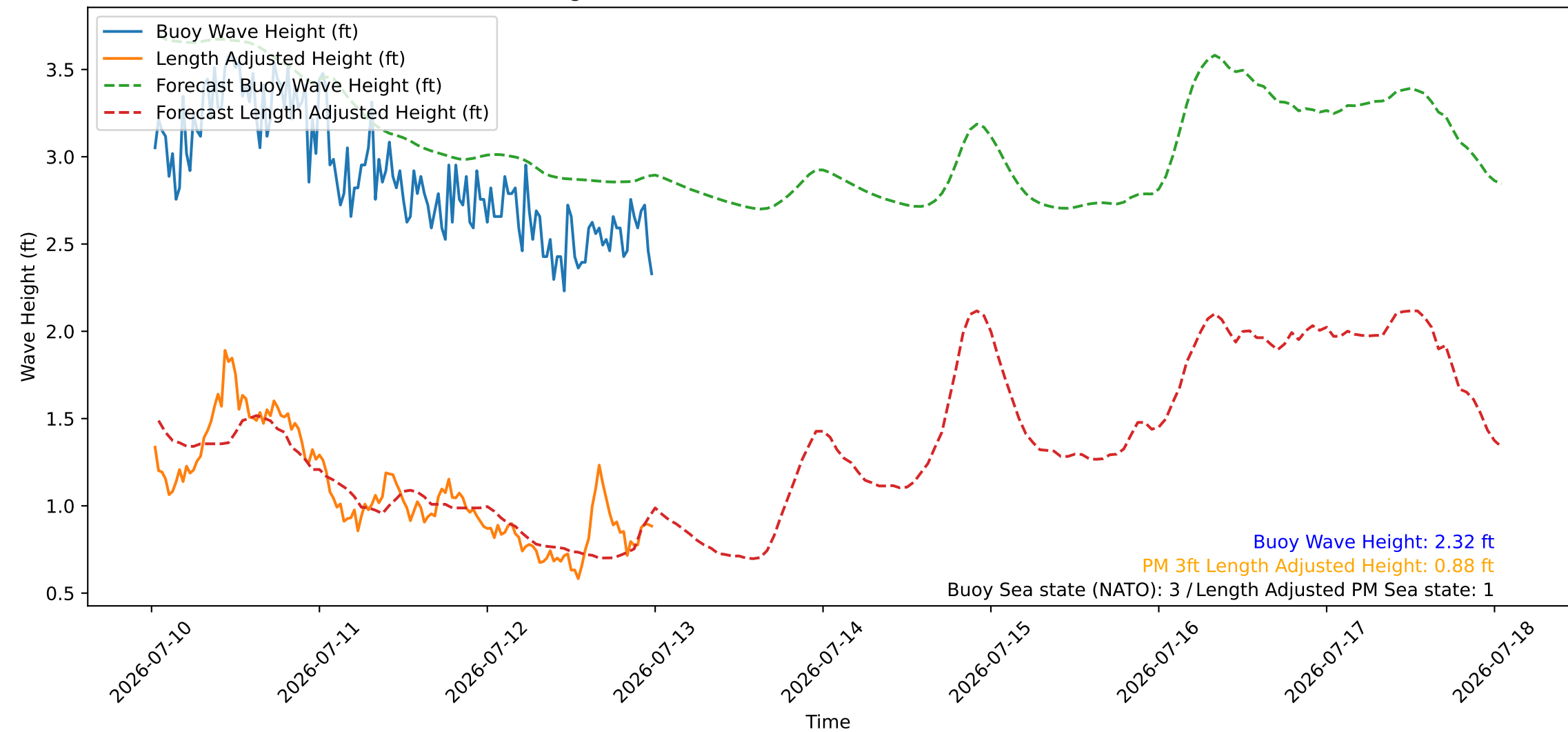
Wave Heights over Time for Green Beach at 2026-07-13 00:31:07
