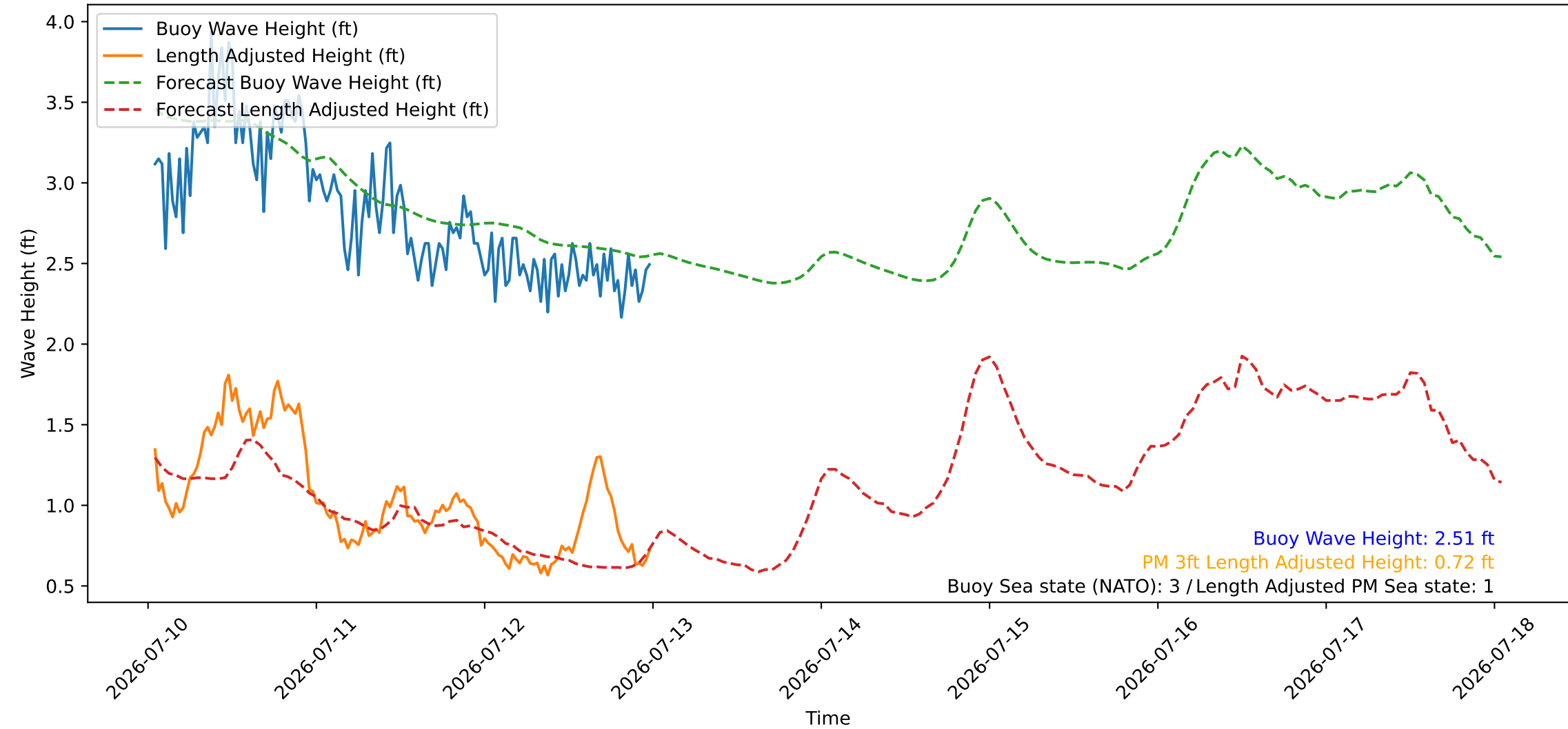
Wave Heights over Time for Red Beach at 2026-07-13 00:30:45
