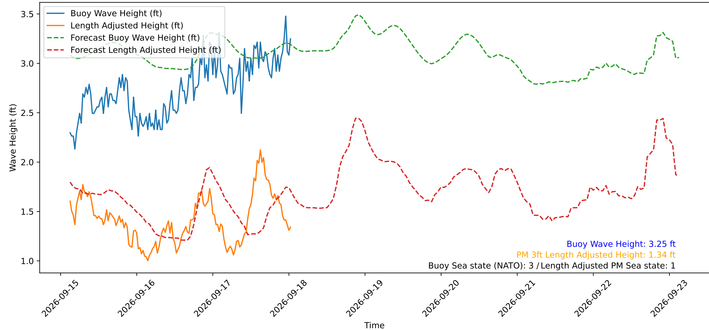
Wave Heights over Time for Green Beach at 2026-09-18 02:31:11
