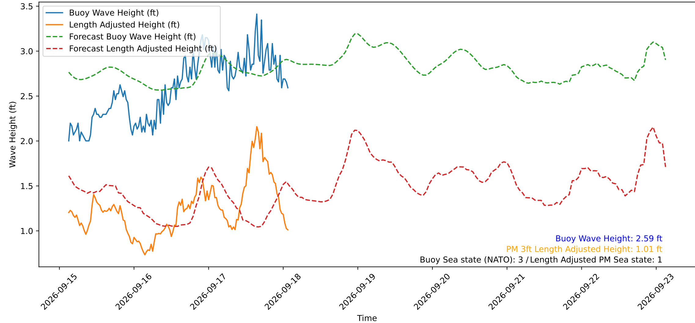
Wave Heights over Time for Red Beach at 2026-09-18 02:30:48
