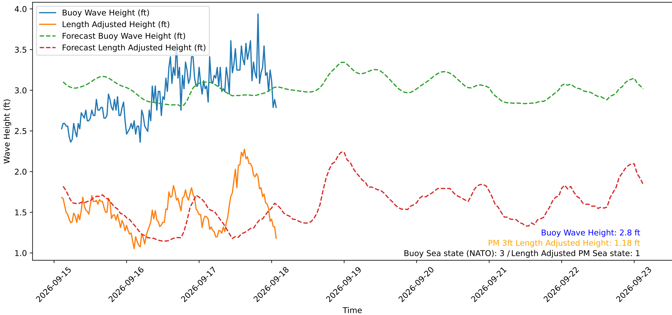
Wave Heights over Time for Oceanside Harbor at 2026-09-18 02:30:29
