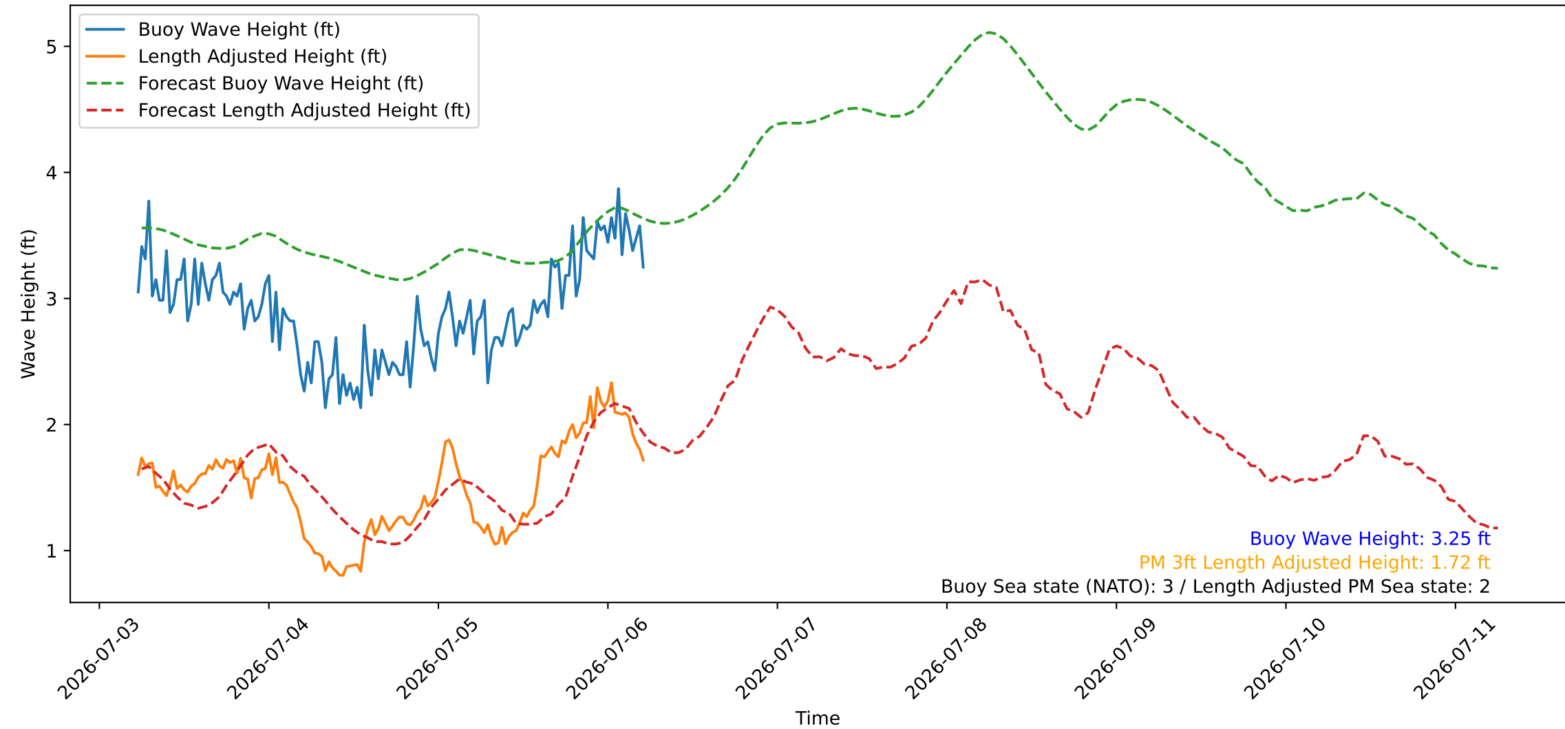
Wave Heights over Time for Oceanside Harbor at 2026-07-06 05:40:26
