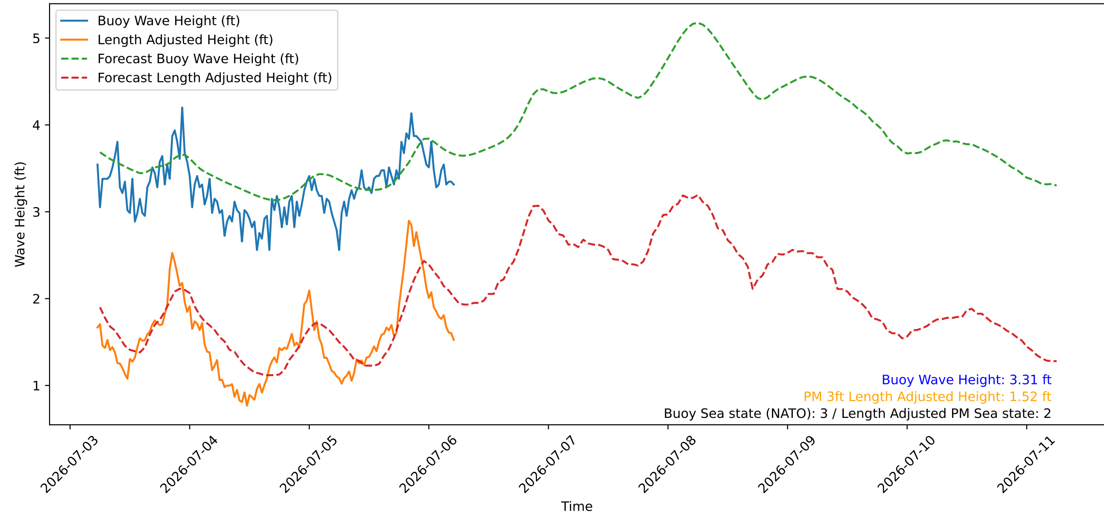
Wave Heights over Time for Green Beach at 2026-07-06 05:41:08
