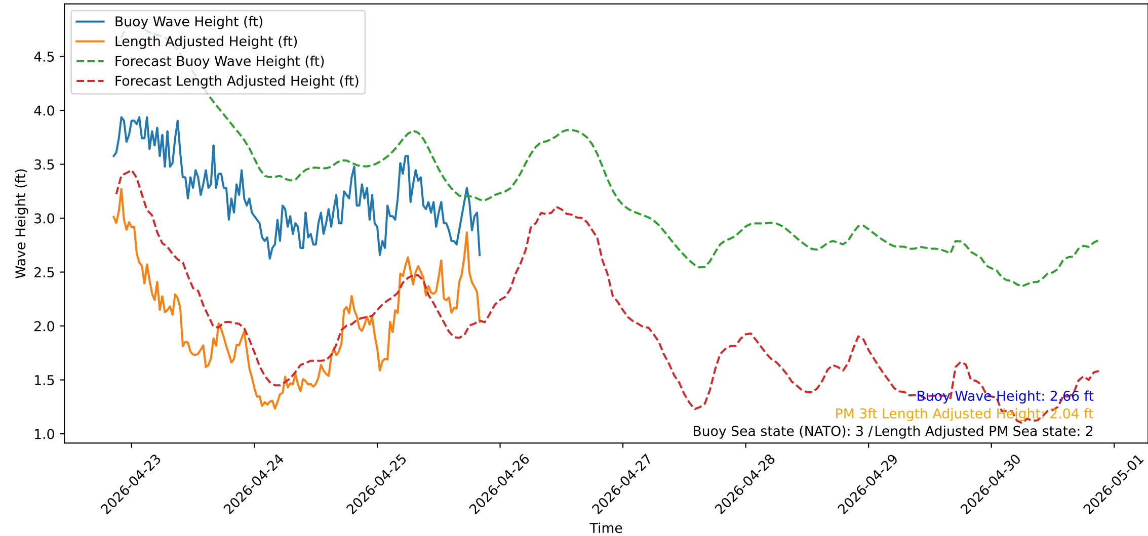
Wave Heights over Time for Green Beach at 2026-04-25 20:41:13
