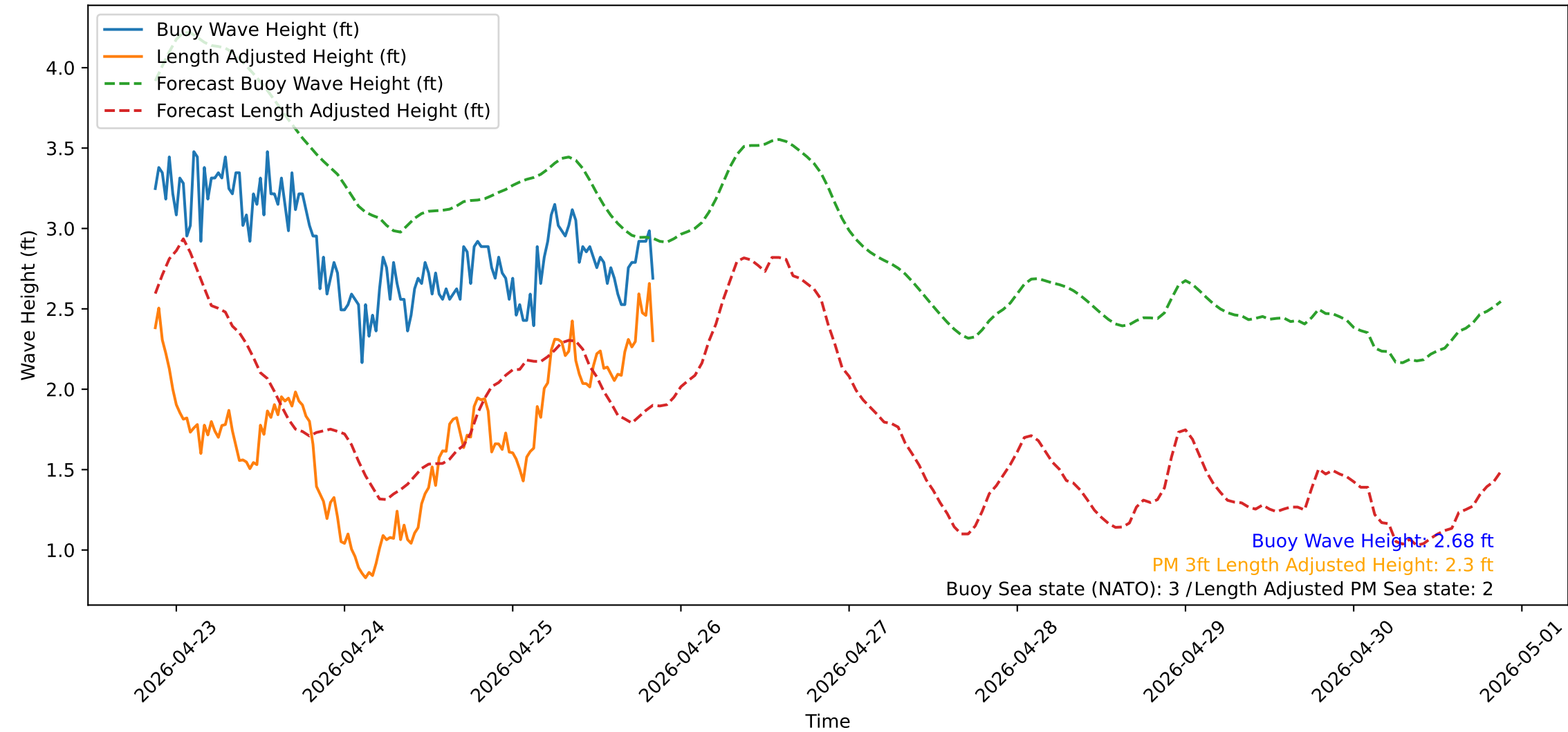
Wave Heights over Time for Red Beach at 2026-04-25 20:40:51
