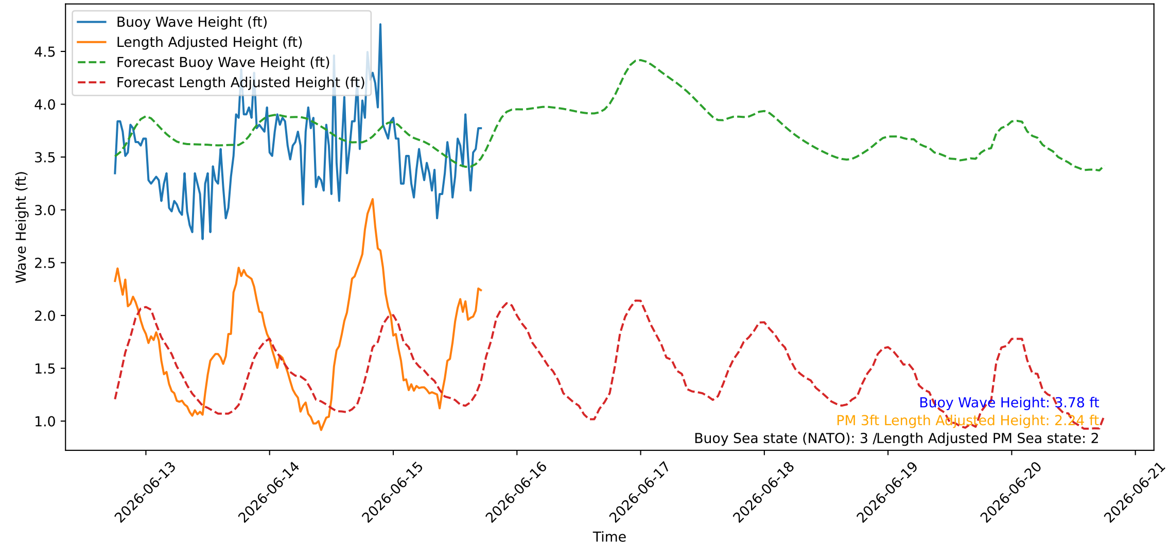
Wave Heights over Time for Red Beach at 2026-06-15 17:50:46
