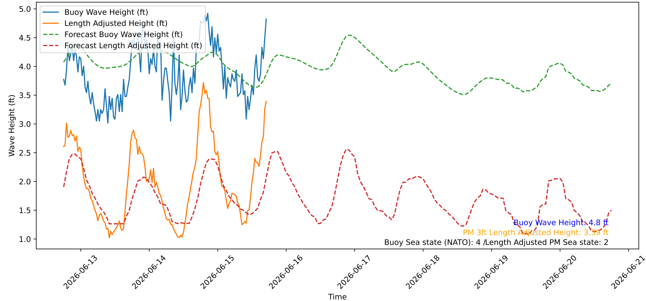
Wave Heights over Time for Green Beach at 2026-06-15 17:51:08
