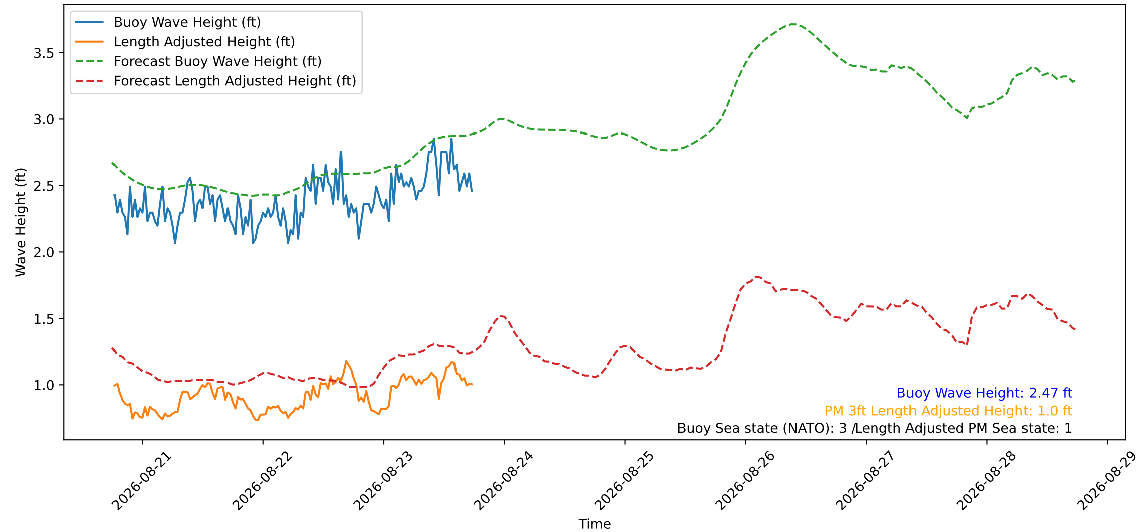
Wave Heights over Time for Red Beach at 2026-08-23 18:10:50
