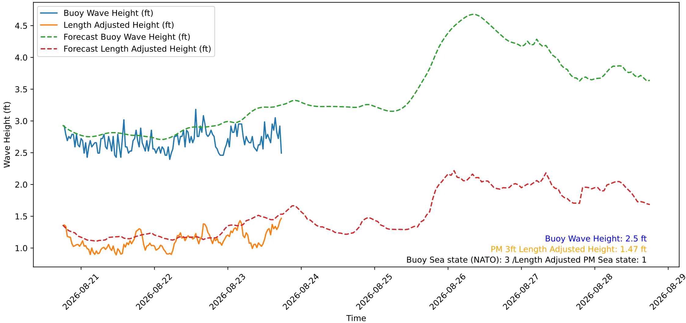
Wave Heights over Time for Green Beach at 2026-08-23 18:11:12
