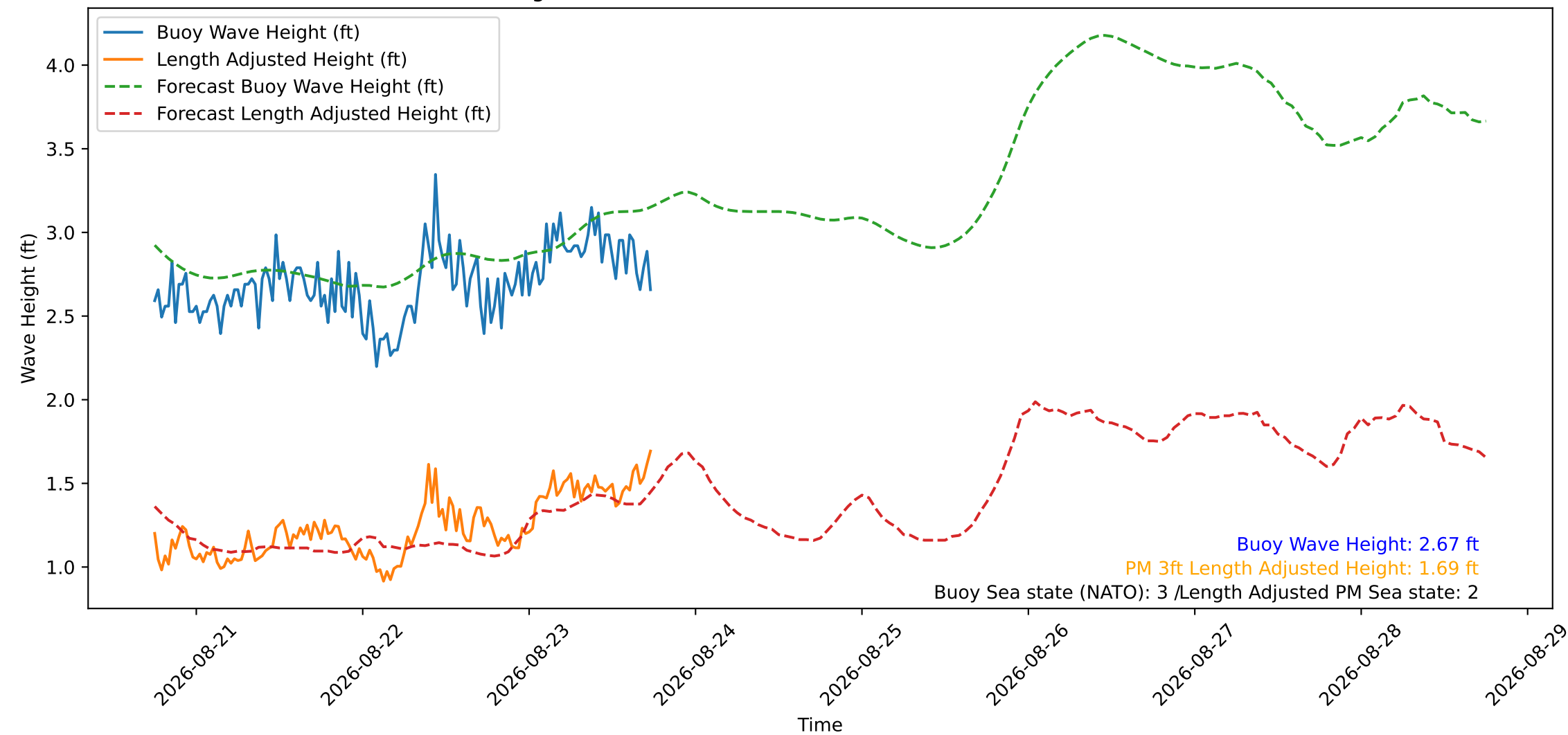
Wave Heights over Time for Oceanside Harbor at 2026-08-23 18:10:30
