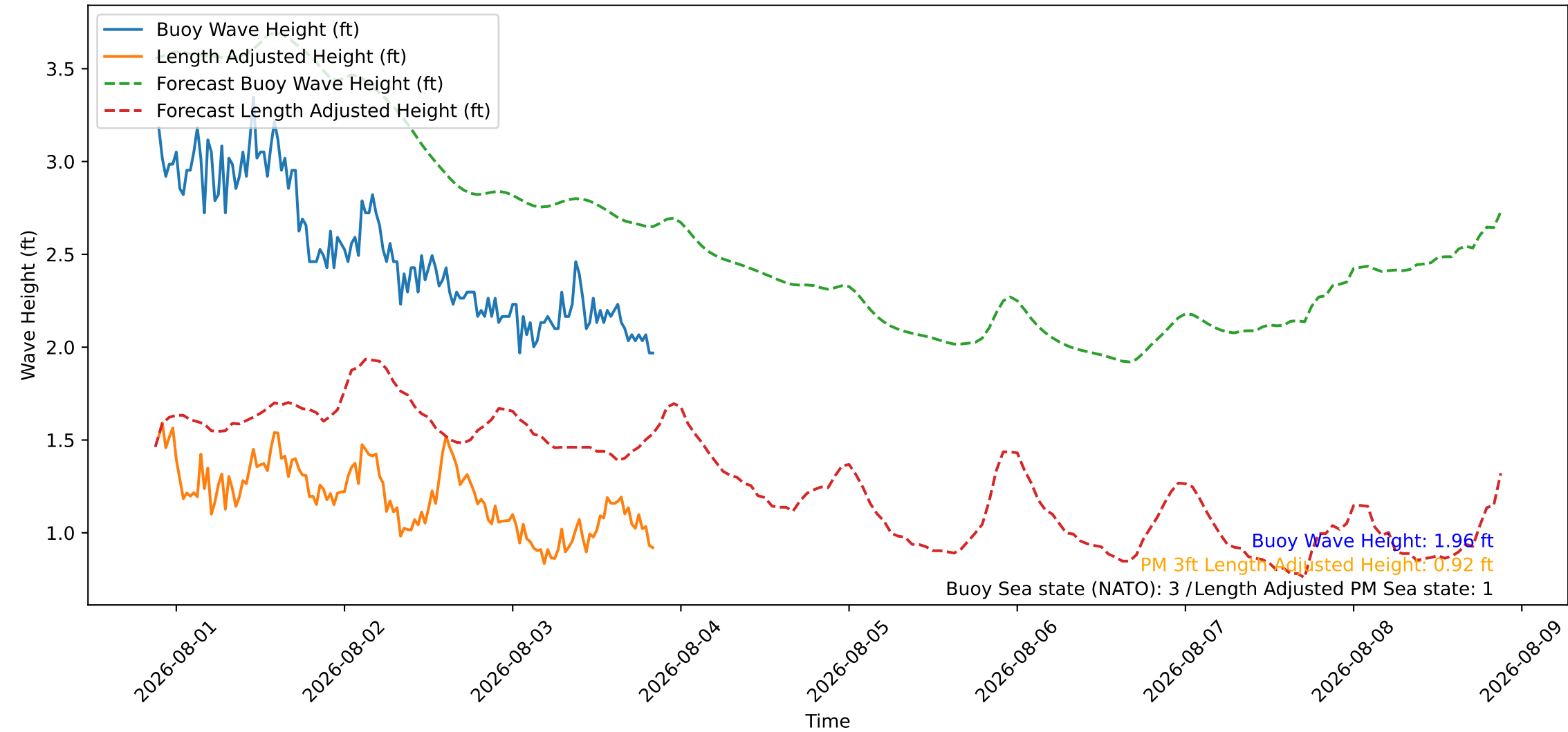
Wave Heights over Time for Red Beach at 2026-08-03 21:00:45
