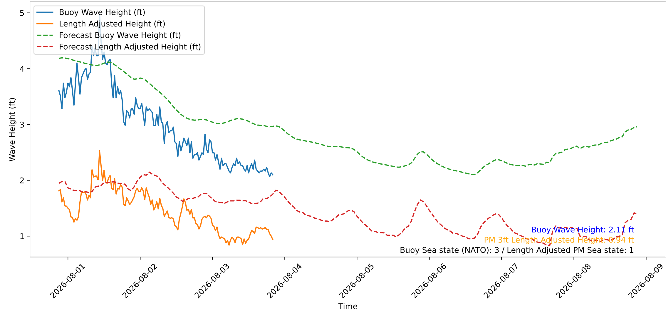
Wave Heights over Time for Green Beach at 2026-08-03 21:01:07
