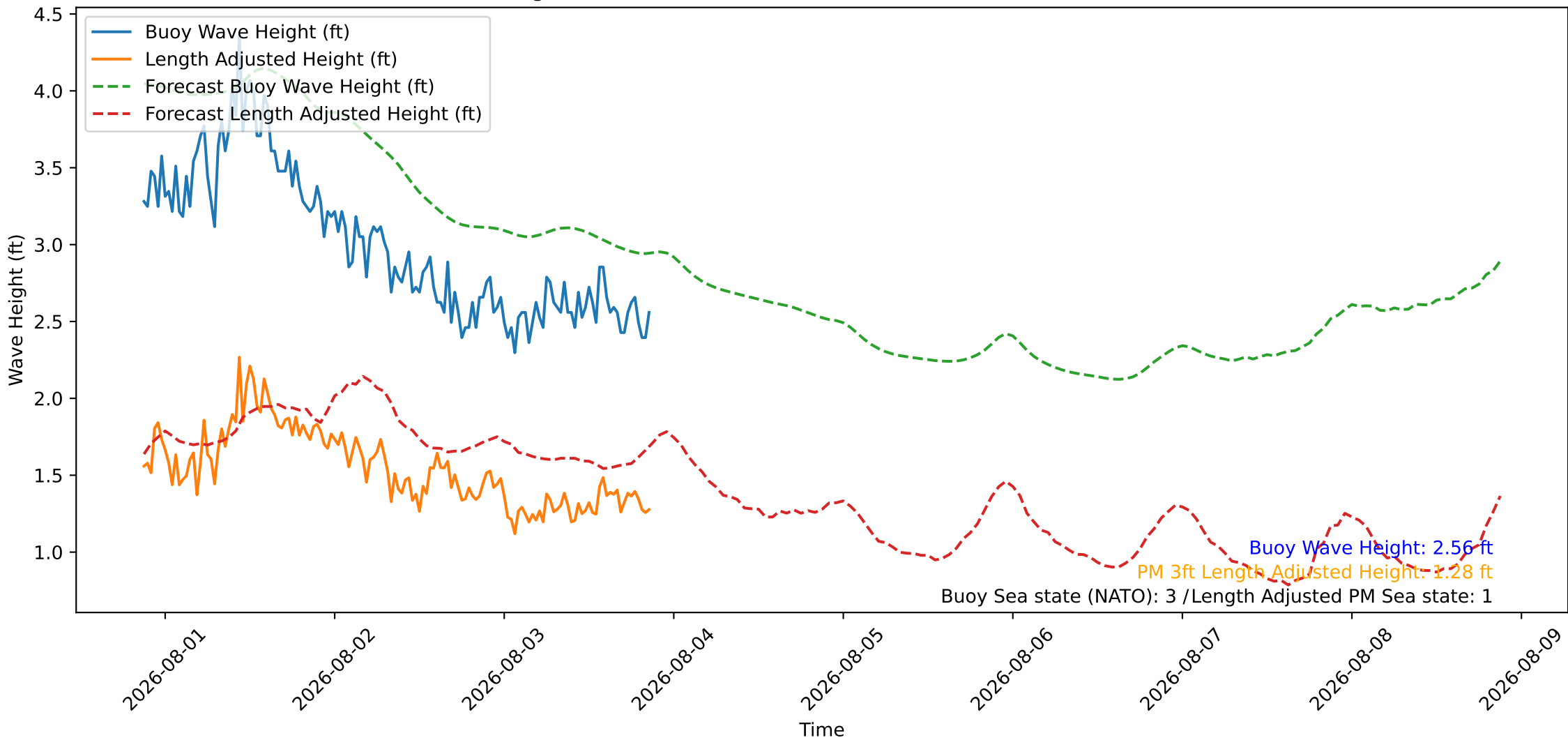
Wave Heights over Time for Oceanside Harbor at 2026-08-03 21:00:26
