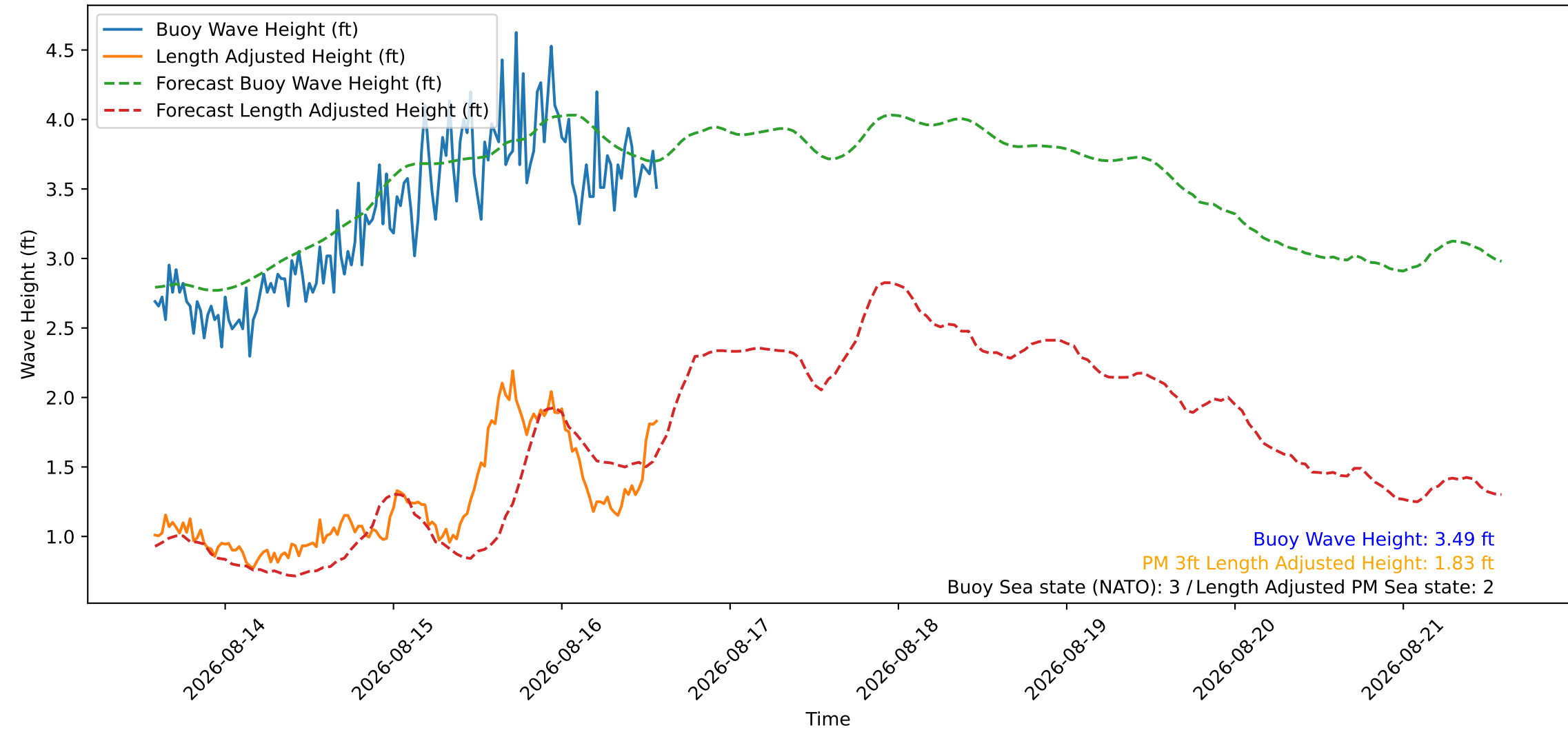
Wave Heights over Time for Oceanside Harbor at 2026-08-16 14:10:27
