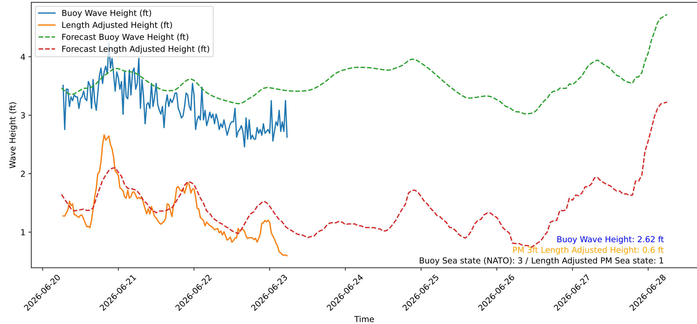
Wave Heights over Time for Green Beach at 2026-06-23 06:21:09
