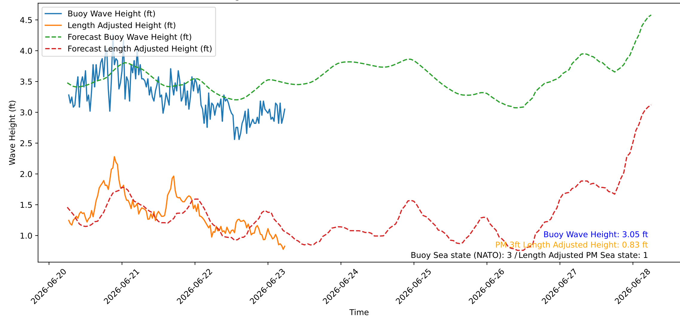
Wave Heights over Time for Oceanside Harbor at 2026-06-23 06:20:26
