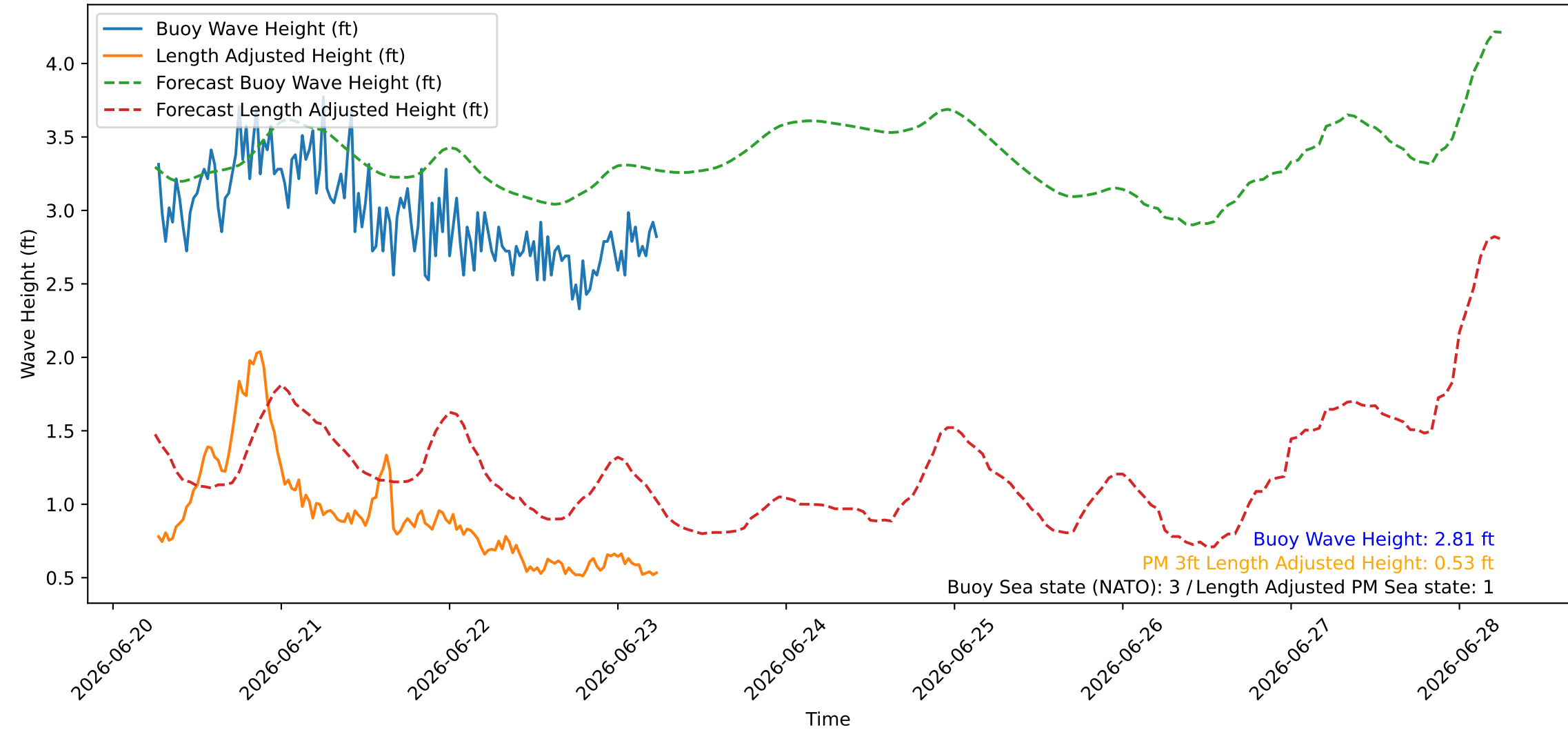
Wave Heights over Time for Red Beach at 2026-06-23 06:20:47
