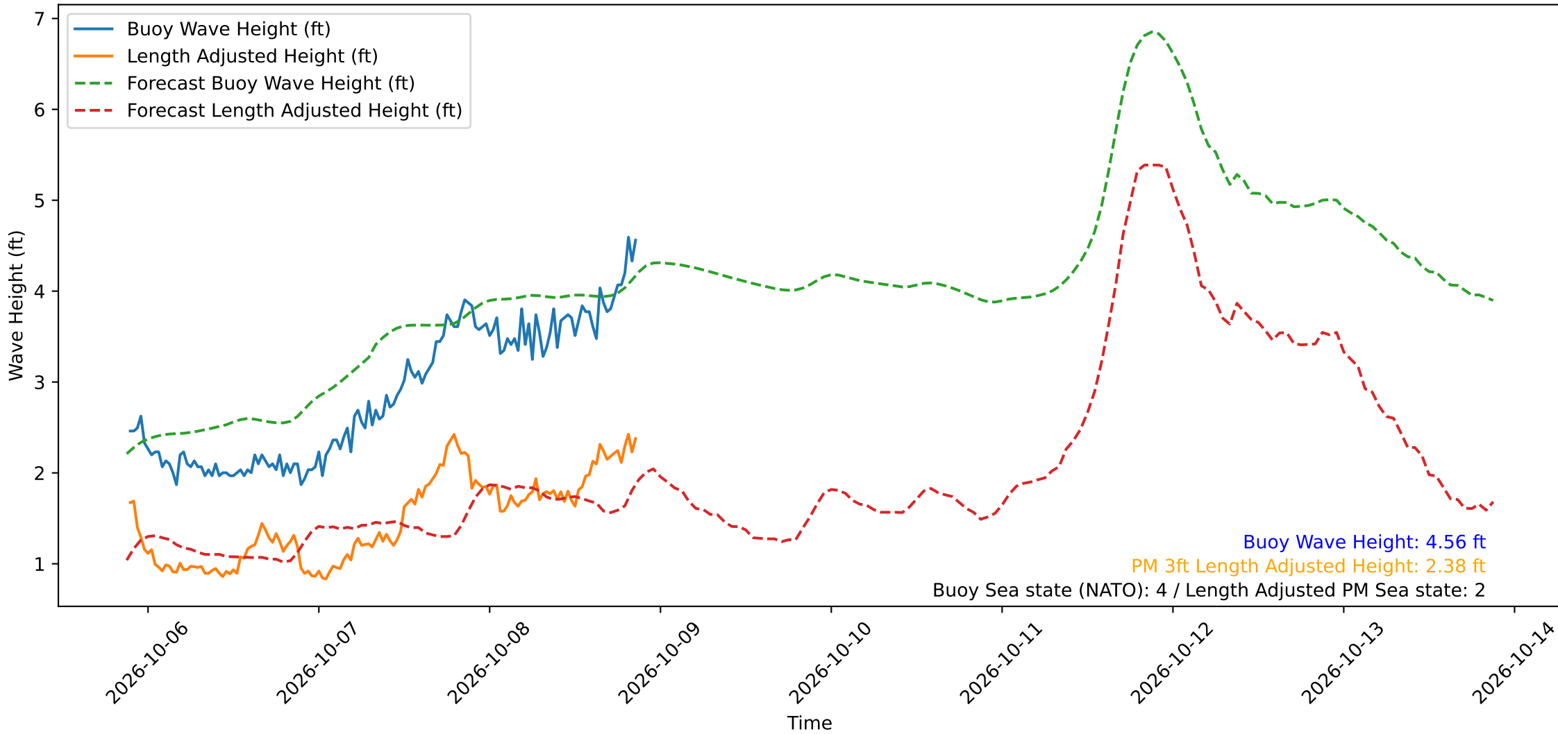
Wave Heights over Time for Red Beach at 2026-10-08 21:10:49
