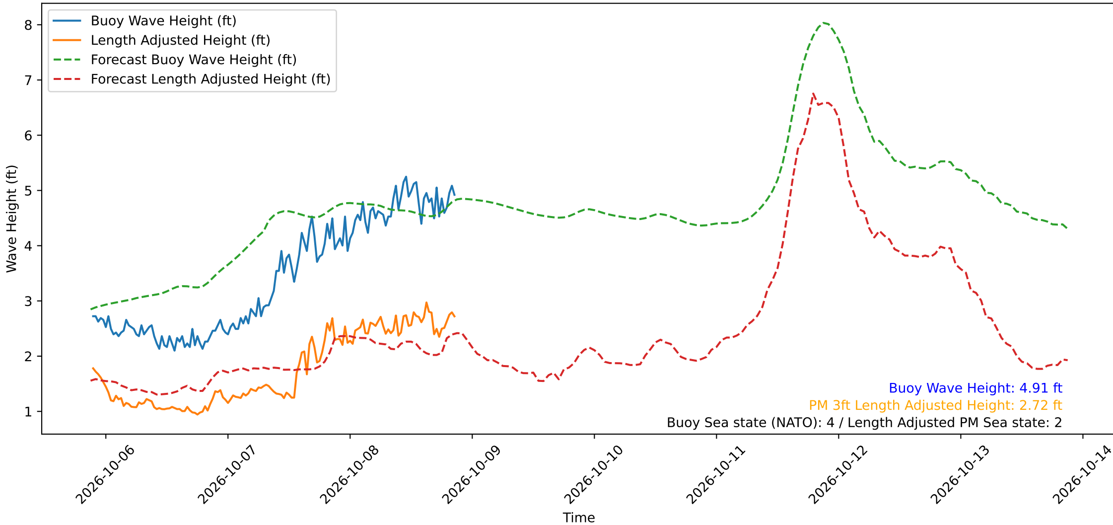
Wave Heights over Time for Green Beach at 2026-10-08 21:11:11
