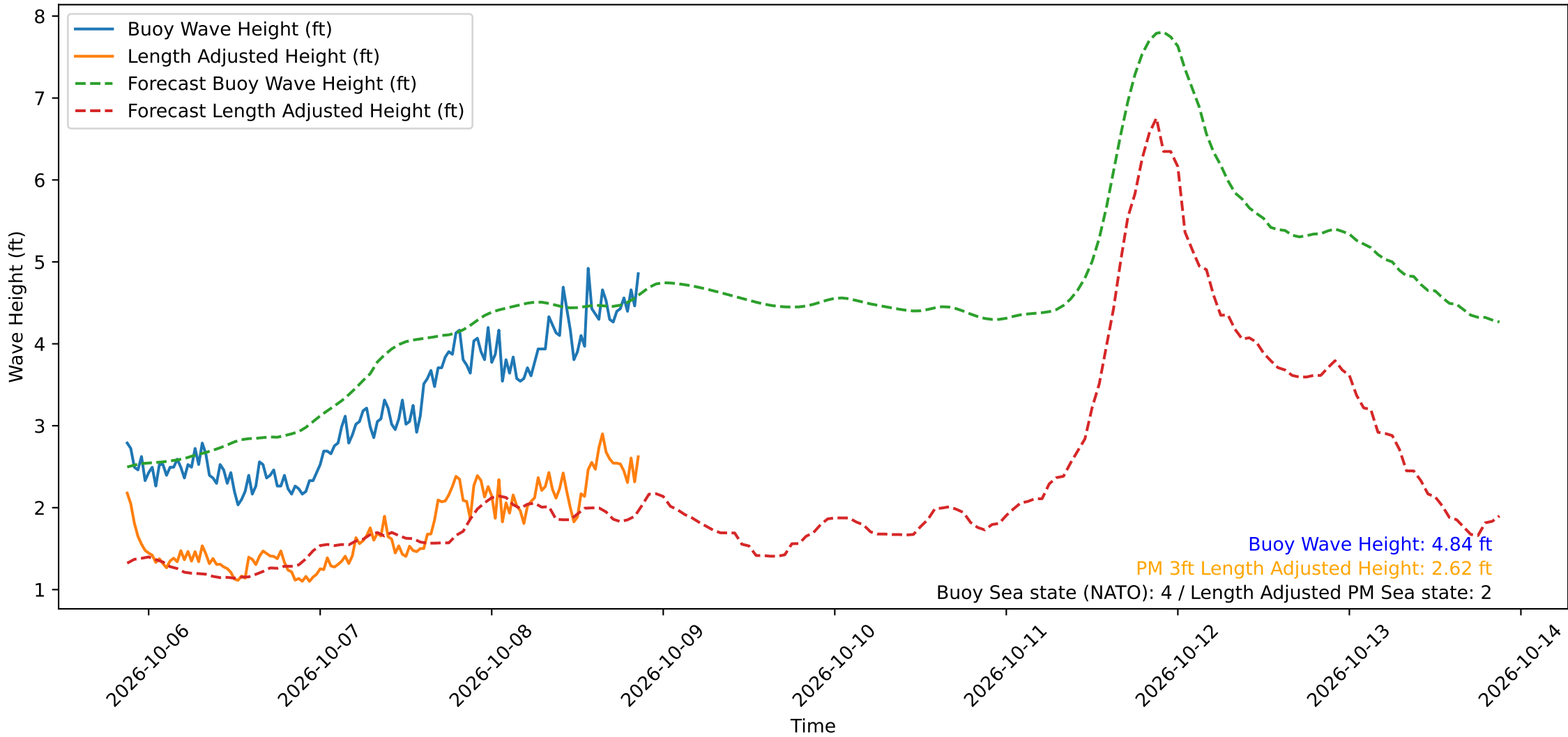
Wave Heights over Time for Oceanside Harbor at 2026-10-08 21:10:30
