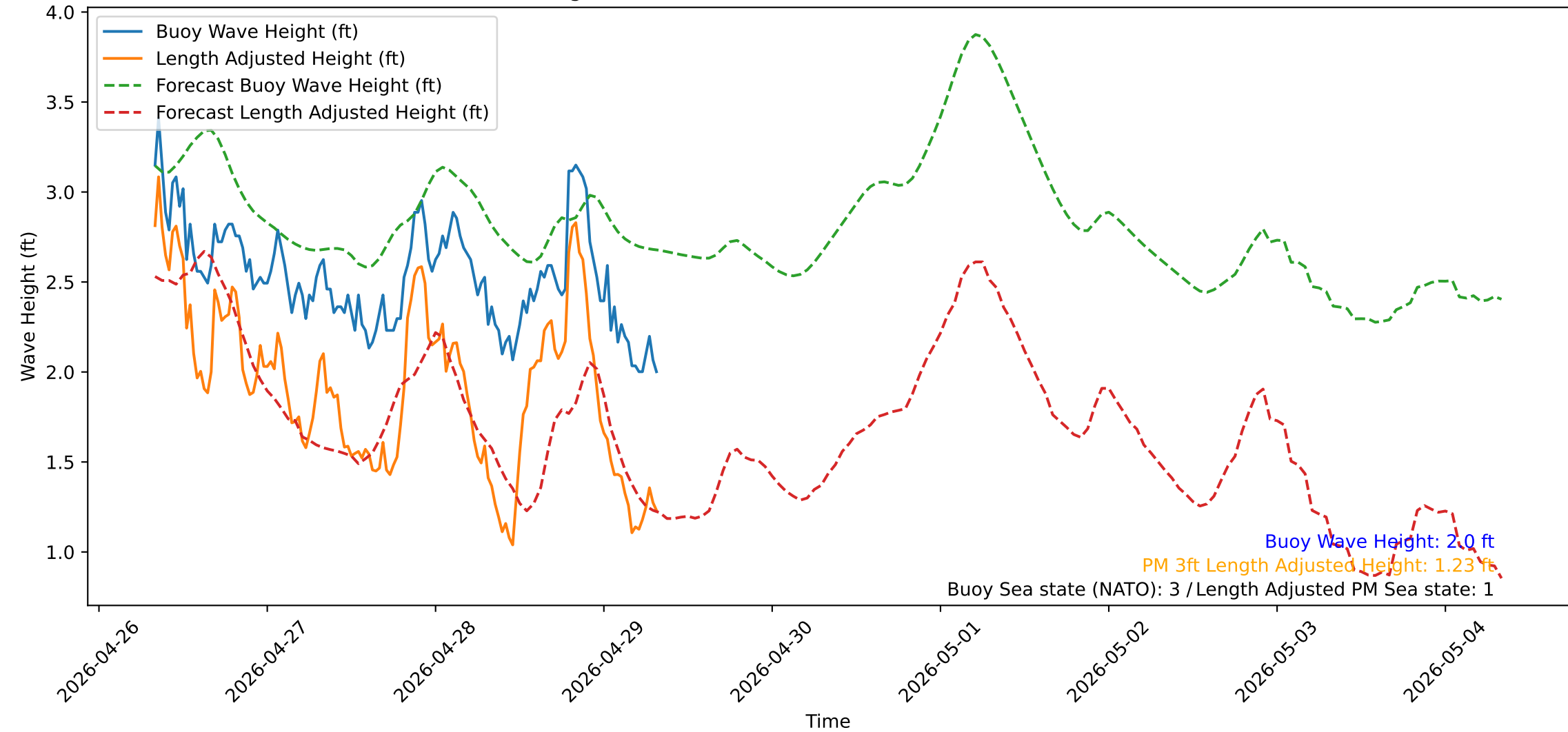
Wave Heights over Time for Green Beach at 2026-04-29 08:11:13
