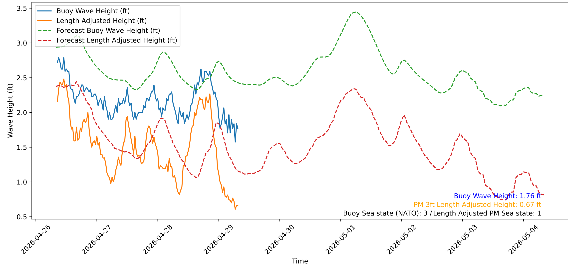
Wave Heights over Time for Red Beach at 2026-04-29 08:10:51
