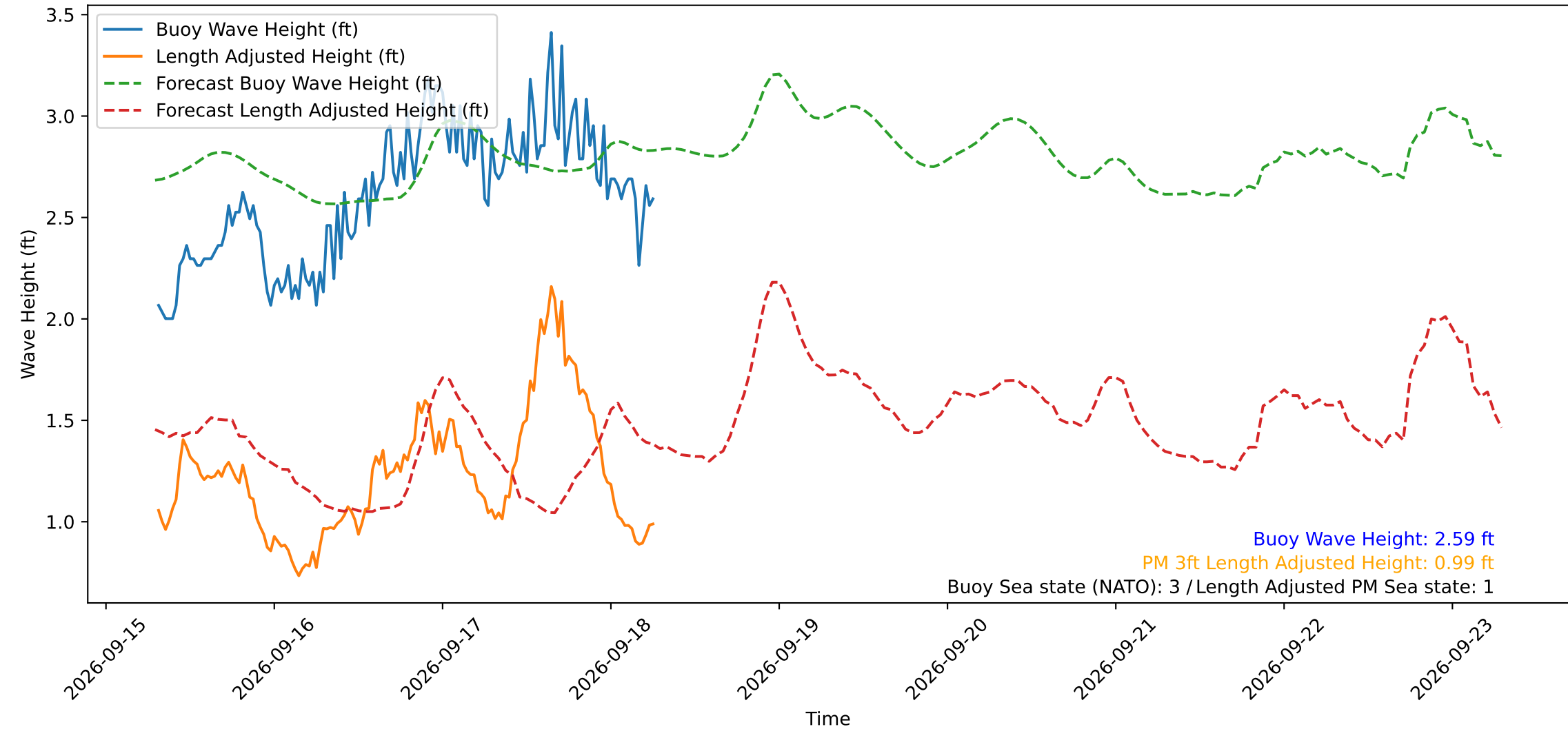
Wave Heights over Time for Red Beach at 2026-09-18 07:00:49
