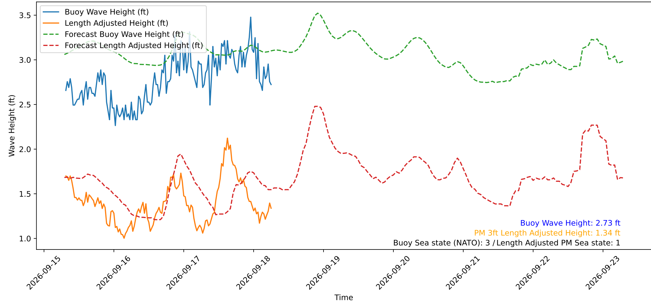
Wave Heights over Time for Green Beach at 2026-09-18 07:01:12
